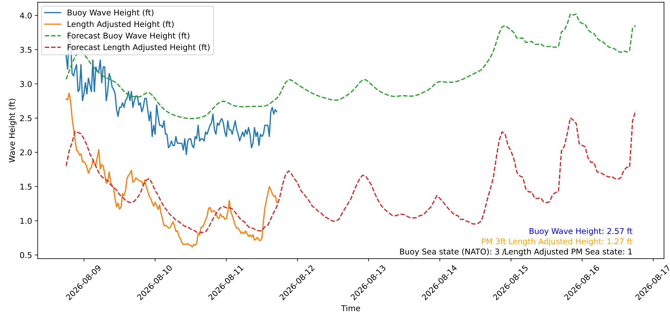
Wave Heights over Time for Green Beach at 2026-08-11 18:01:08
