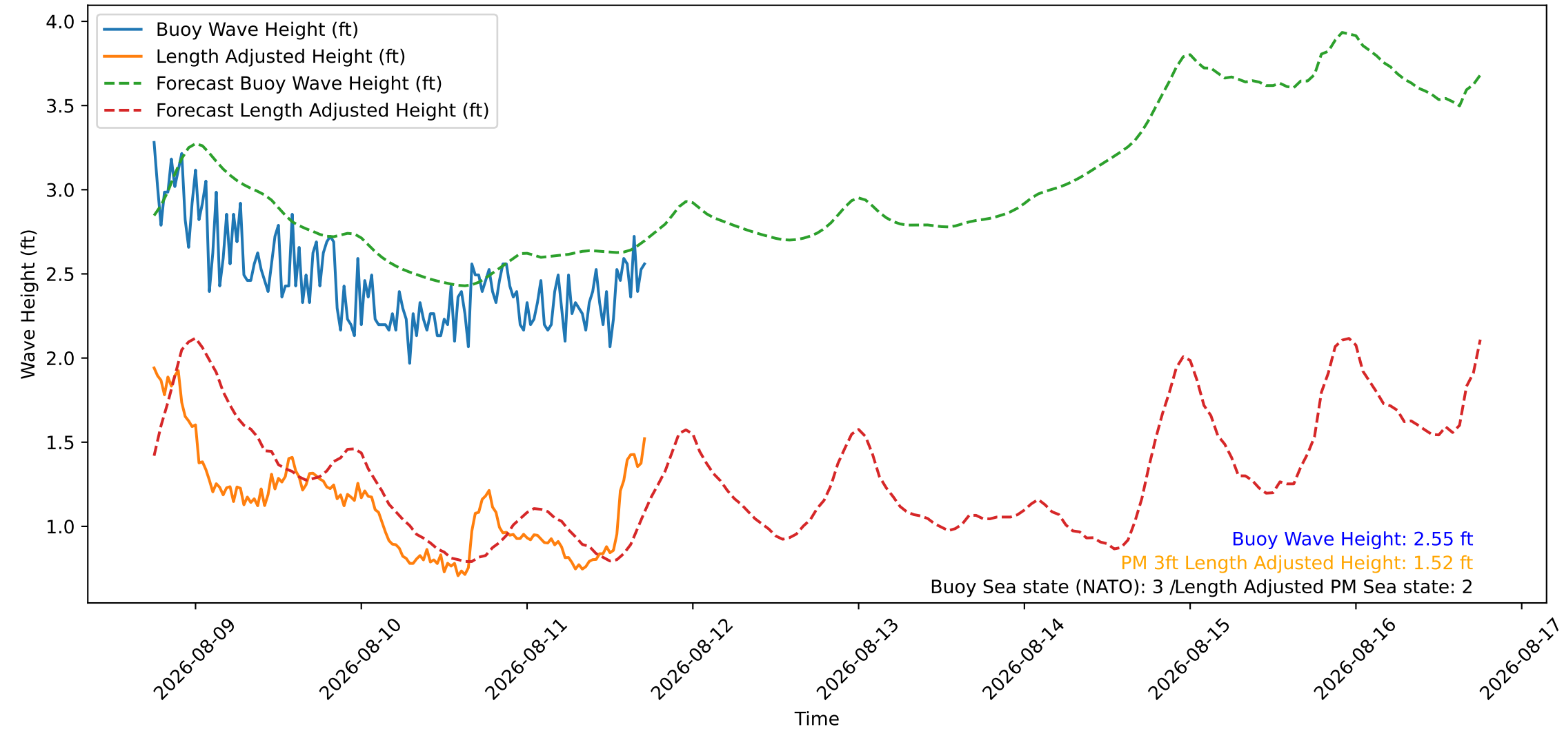
Wave Heights over Time for Oceanside Harbor at 2026-08-11 18:00:26
