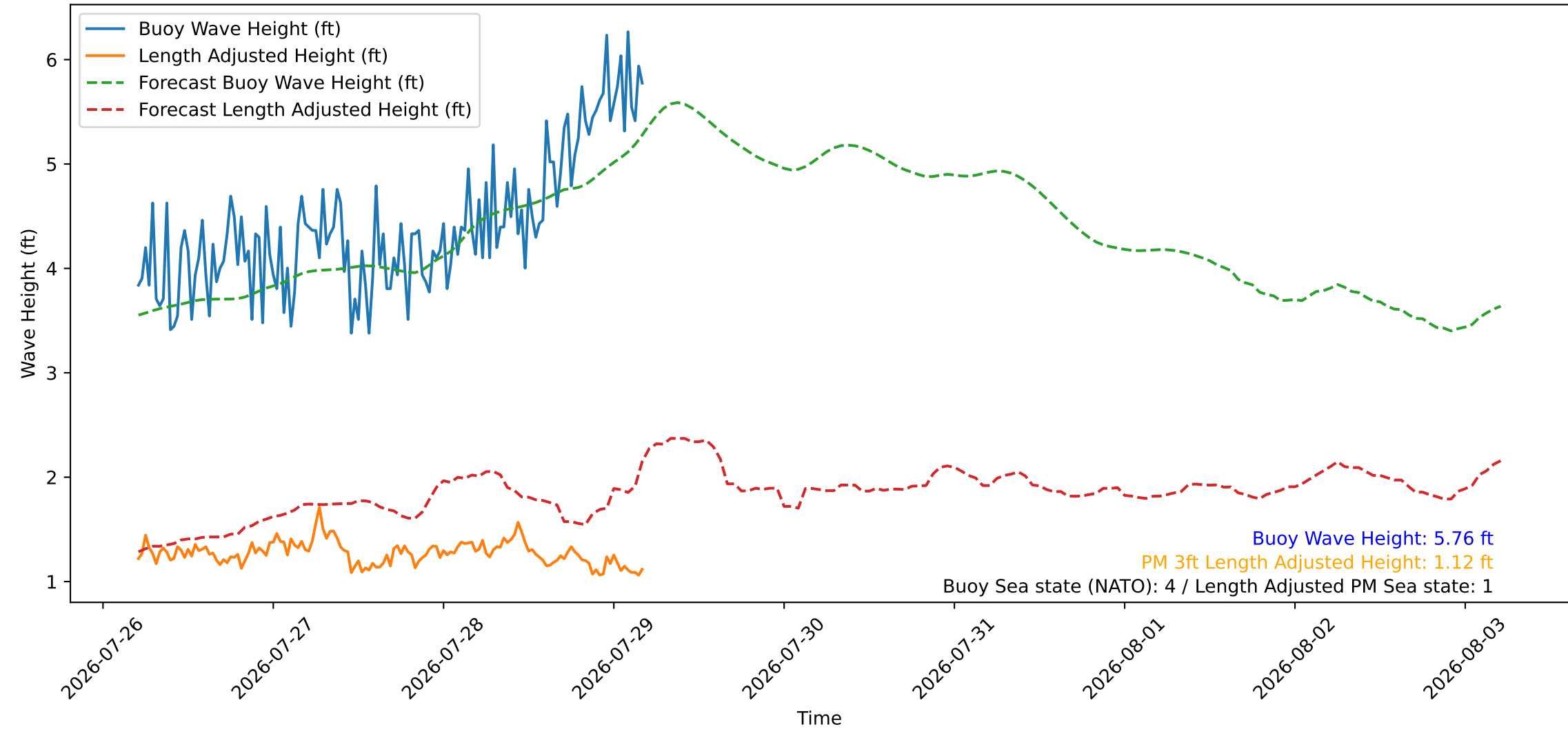
Wave Heights over Time for Green Beach at 2026-07-29 05:01:08
