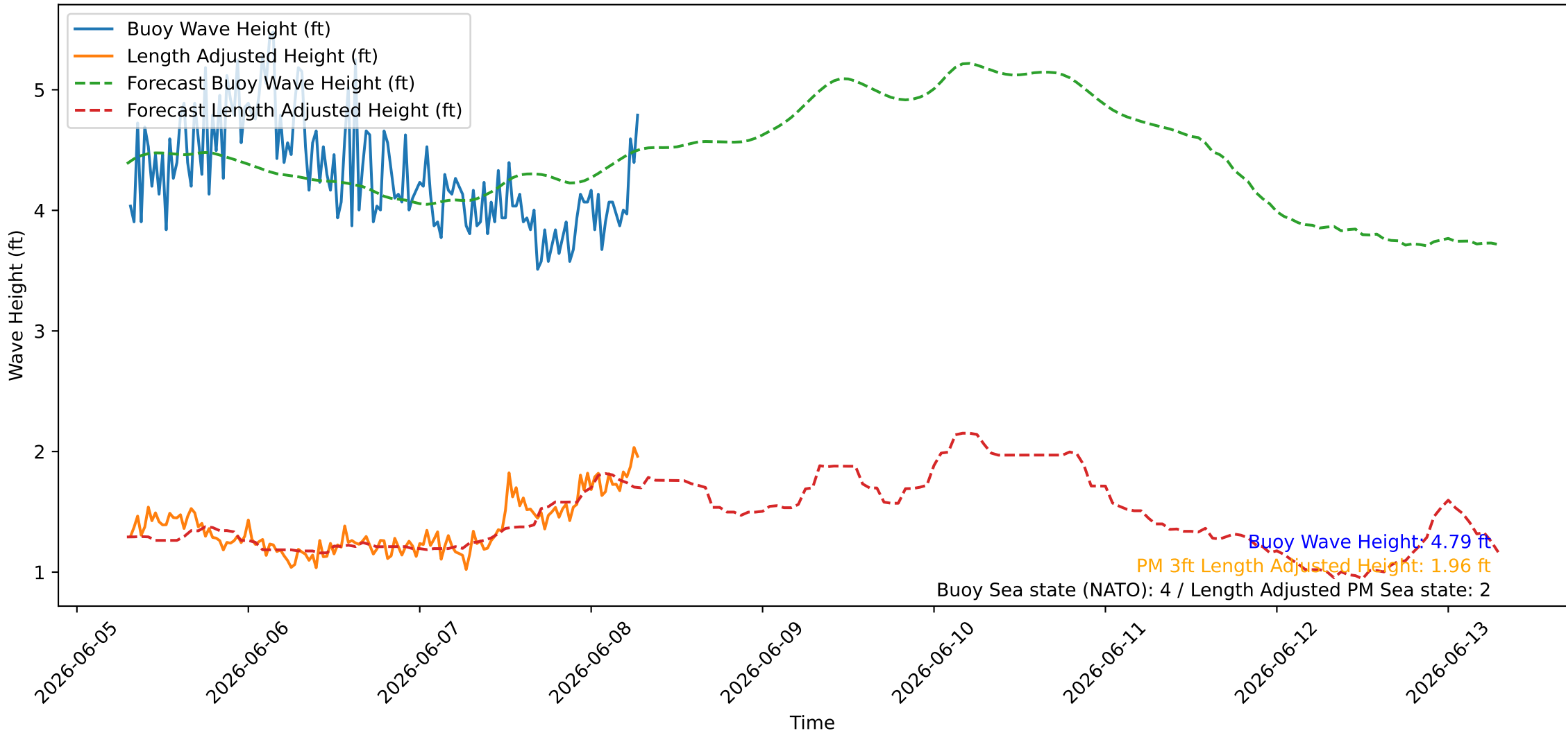
Wave Heights over Time for Oceanside Harbor at 2026-06-08 07:20:25
