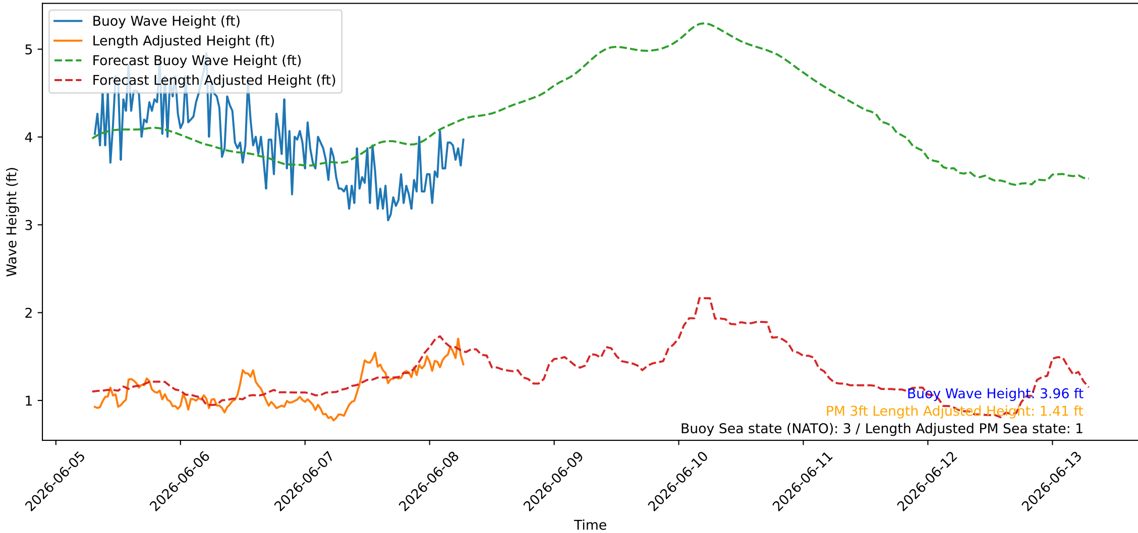
Wave Heights over Time for Red Beach at 2026-06-08 07:20:46
