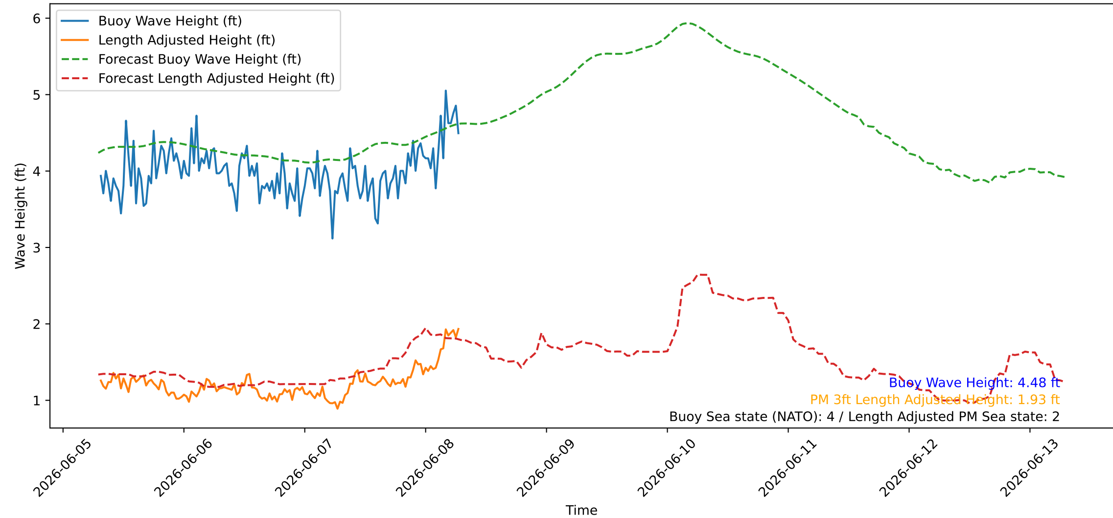
Wave Heights over Time for Green Beach at 2026-06-08 07:21:09
