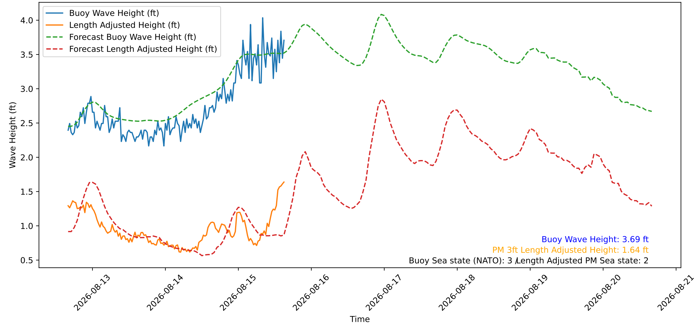
Wave Heights over Time for Red Beach at 2026-08-15 15:40:46
