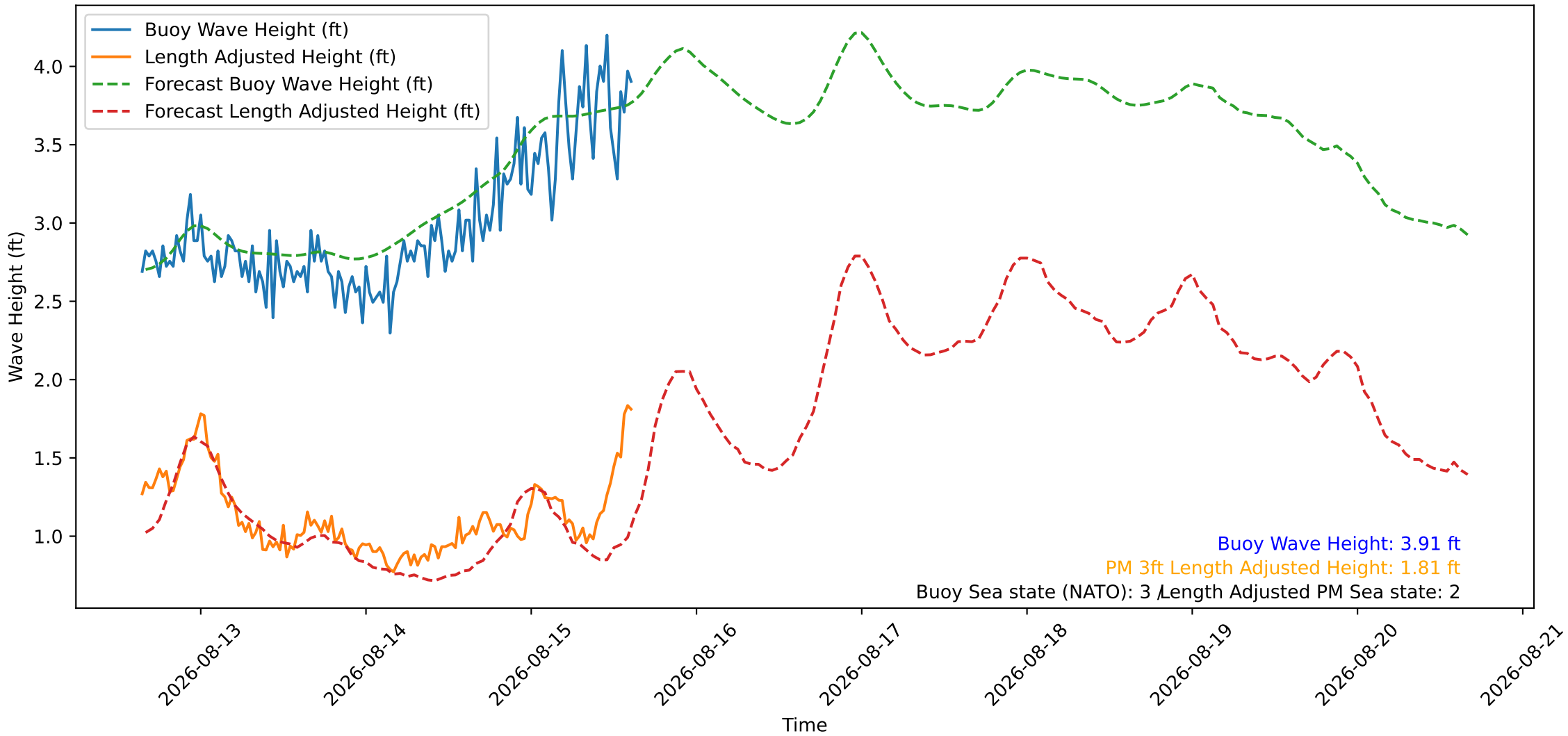
Wave Heights over Time for Oceanside Harbor at 2026-08-15 15:40:26
