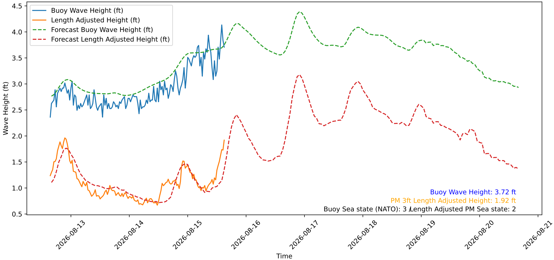
Wave Heights over Time for Green Beach at 2026-08-15 15:41:08
