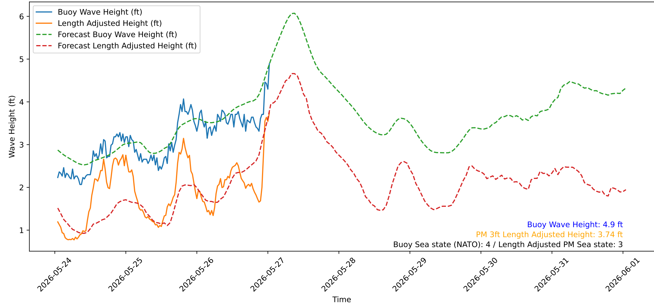
Wave Heights over Time for Green Beach at 2026-05-27 01:11:17
