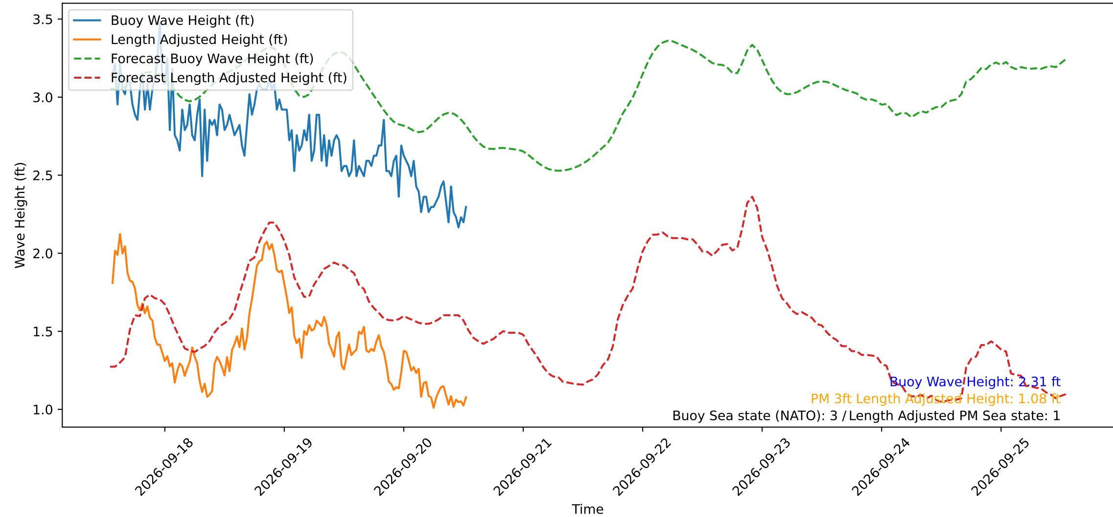
Wave Heights over Time for Green Beach at 2026-09-20 13:11:12
