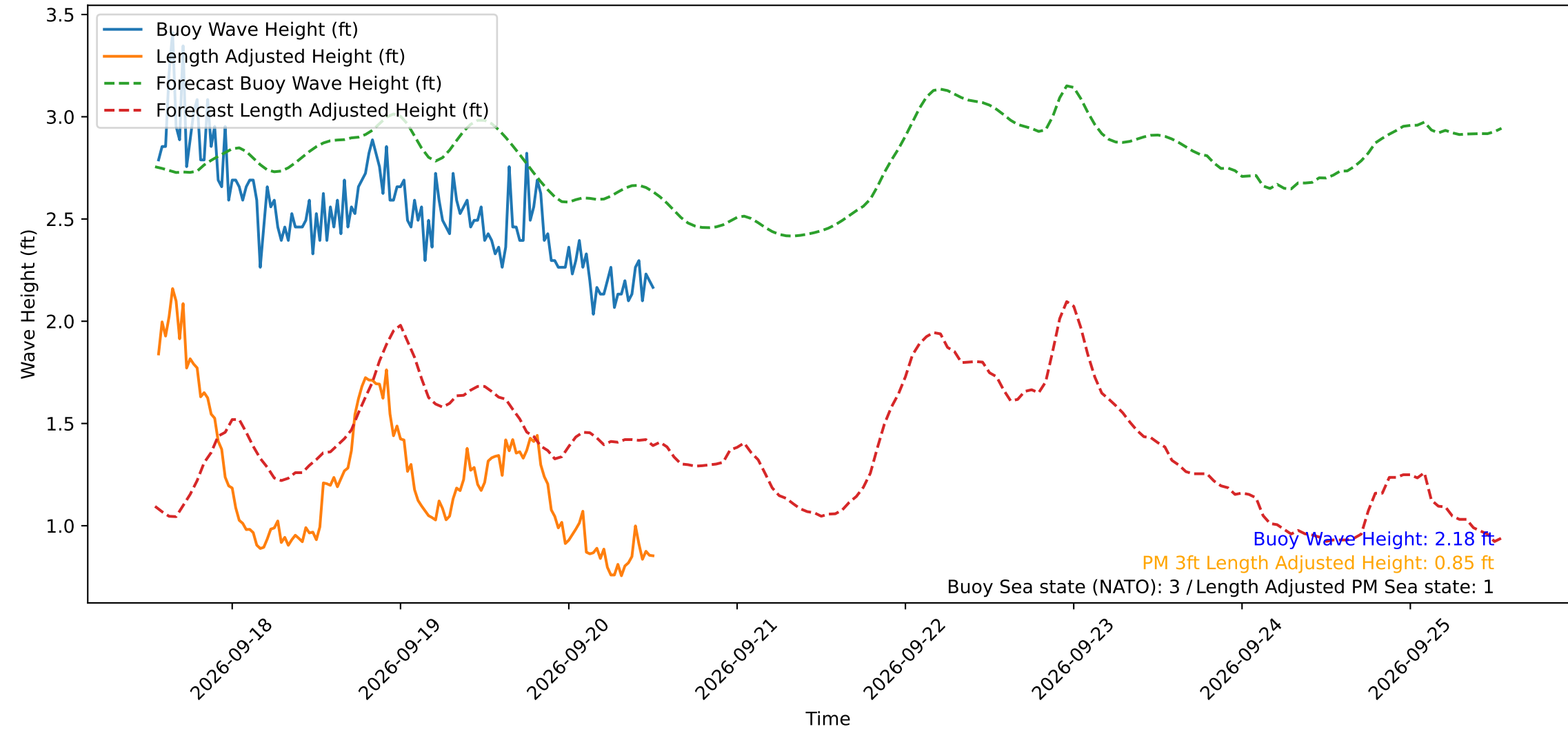
Wave Heights over Time for Red Beach at 2026-09-20 13:10:50
