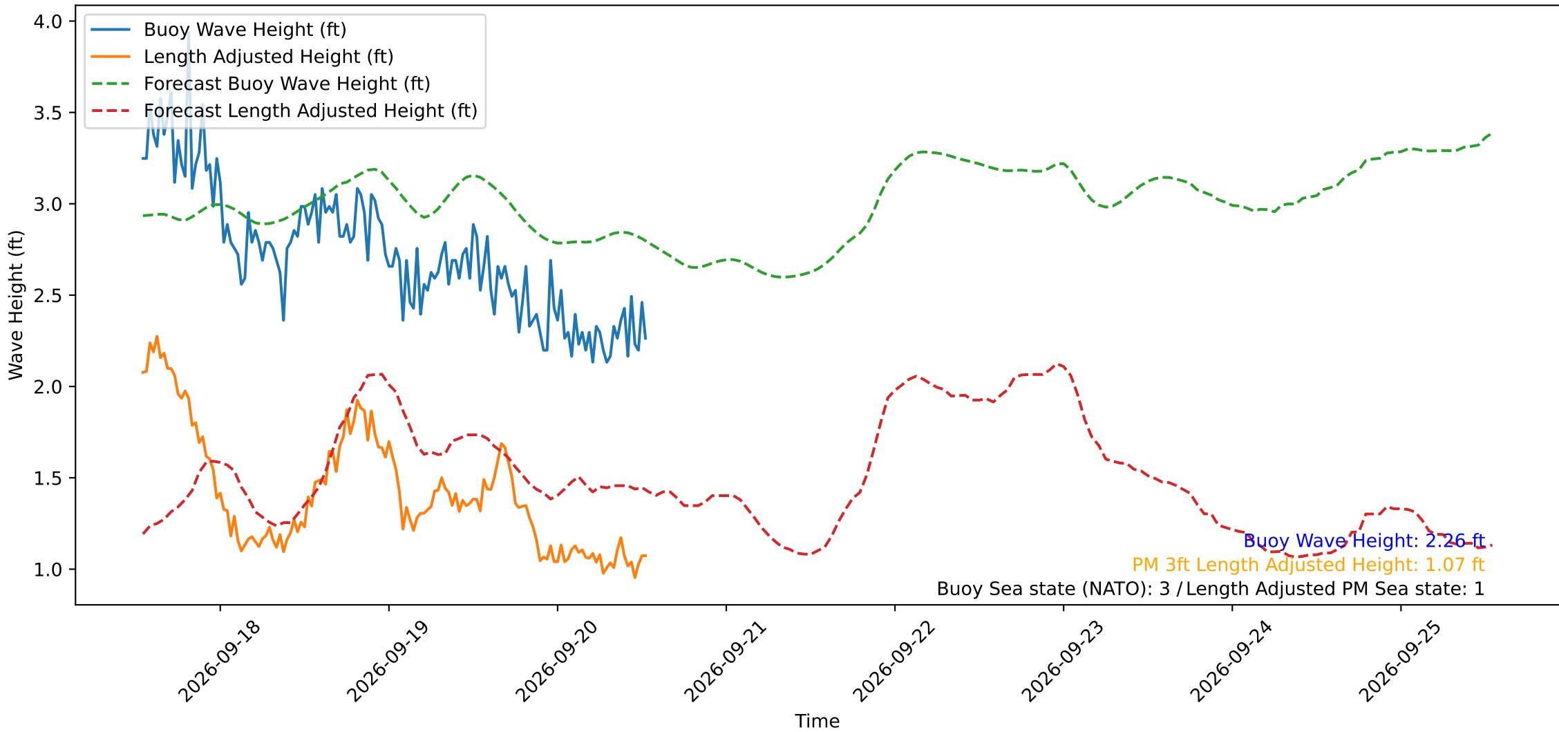
Wave Heights over Time for Oceanside Harbor at 2026-09-20 13:10:30
