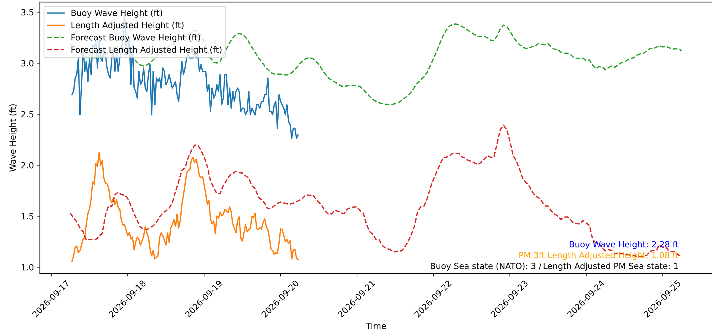
Wave Heights over Time for Green Beach at 2026-09-20 06:11:11
