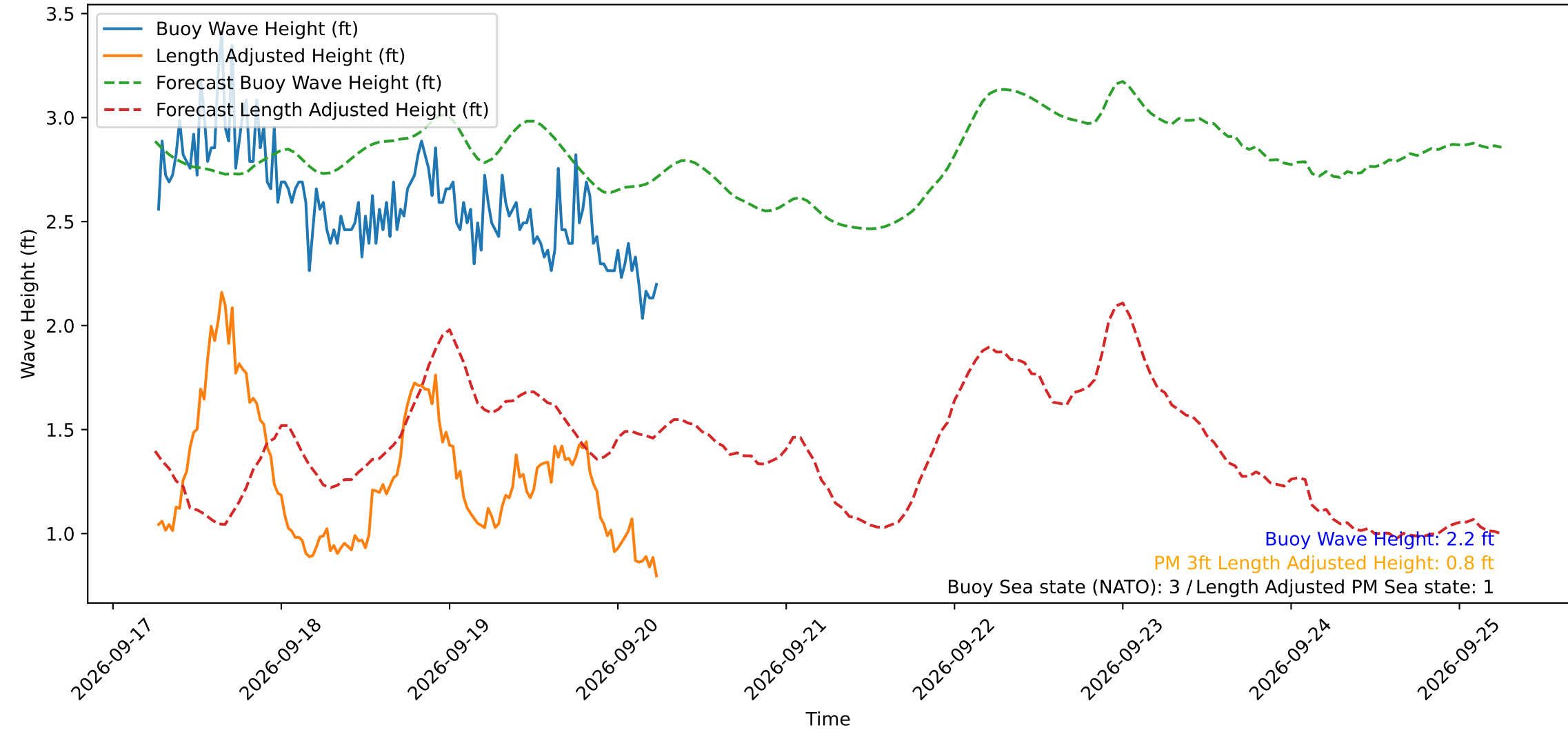
Wave Heights over Time for Red Beach at 2026-09-20 06:10:49
