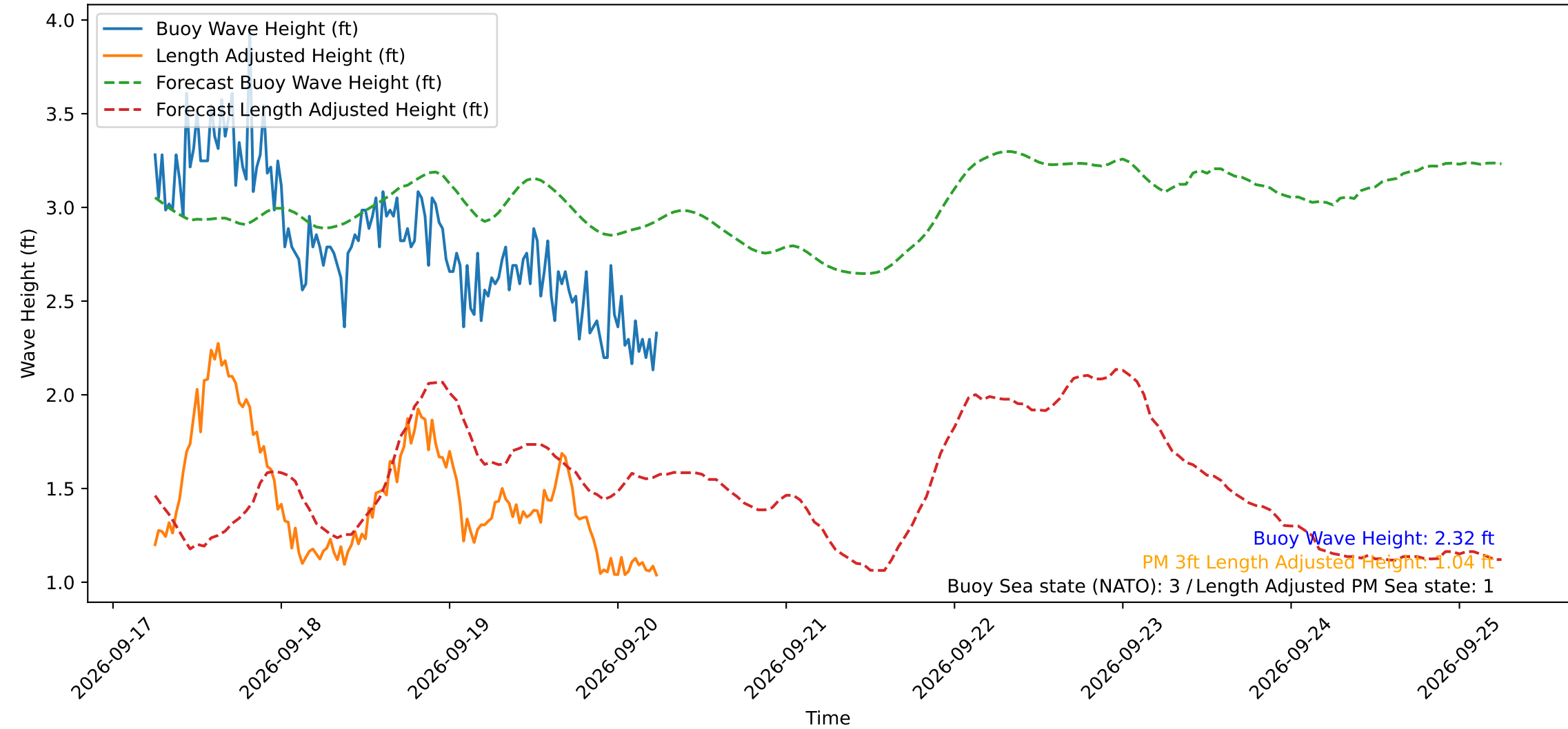
Wave Heights over Time for Oceanside Harbor at 2026-09-20 06:10:29
