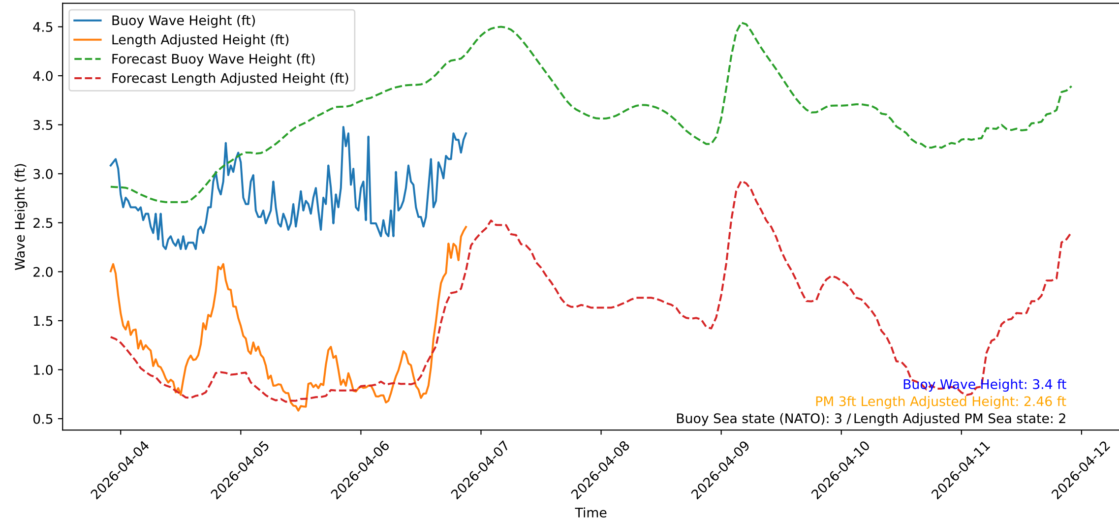
Wave Heights over Time for Green Beach at 2026-04-06 22:01:12
