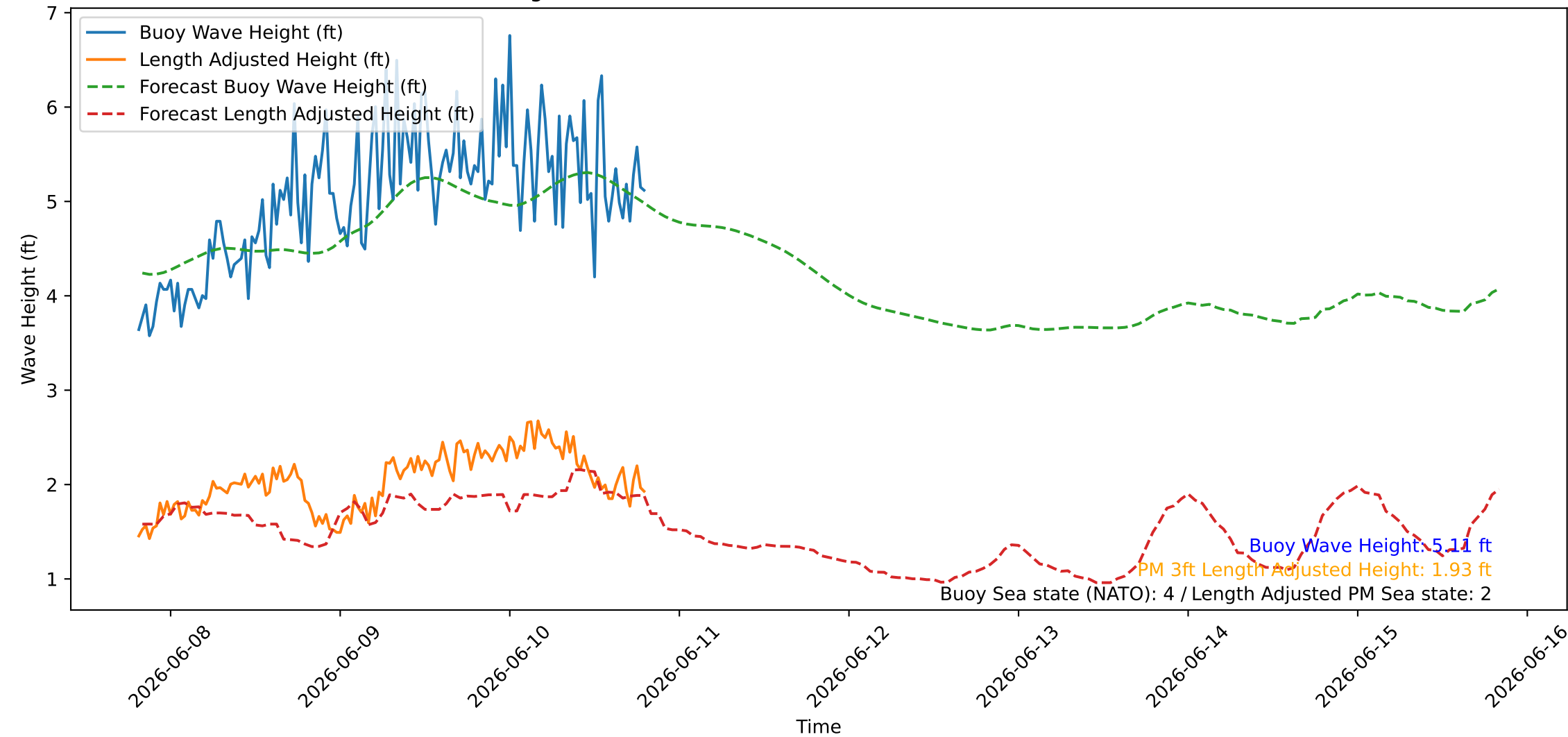
Wave Heights over Time for Oceanside Harbor at 2026-06-10 19:30:27
