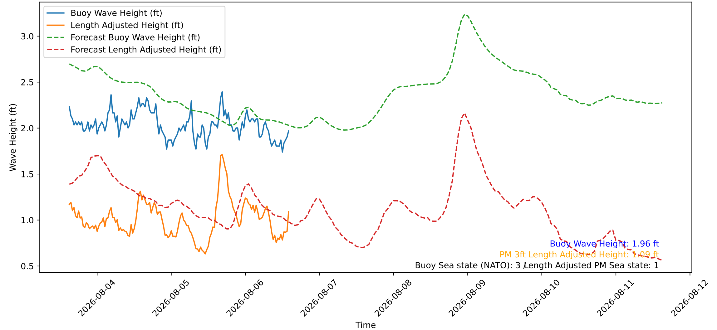
Wave Heights over Time for Red Beach at 2026-08-06 14:40:46
