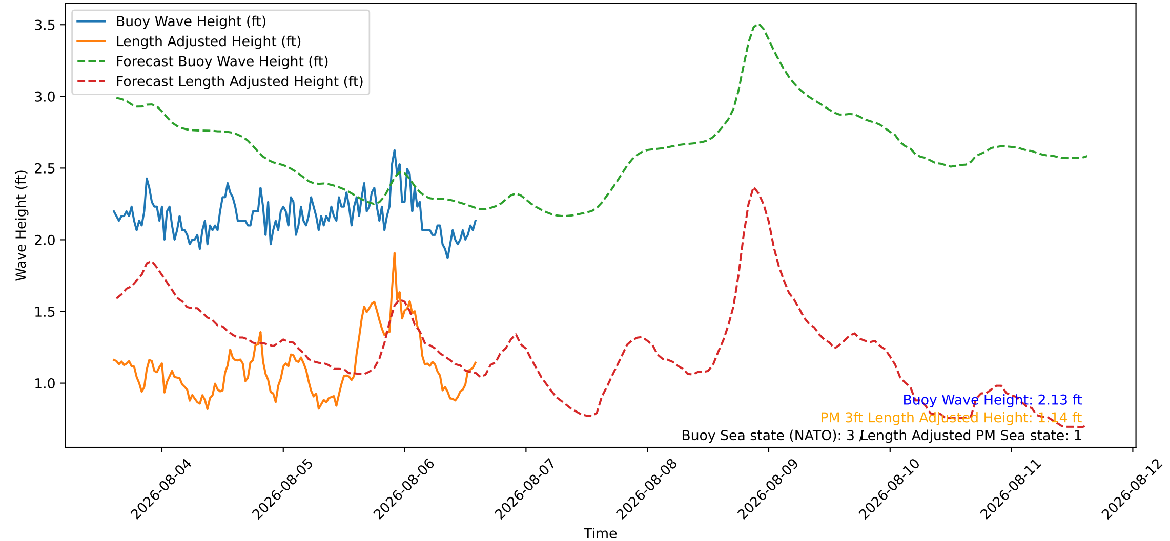
Wave Heights over Time for Green Beach at 2026-08-06 14:41:09
