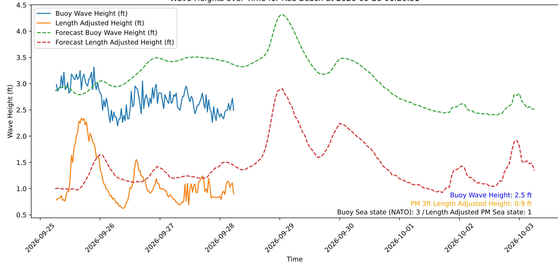
Wave Heights over Time for Red Beach at 2026-09-28 06:20:51
