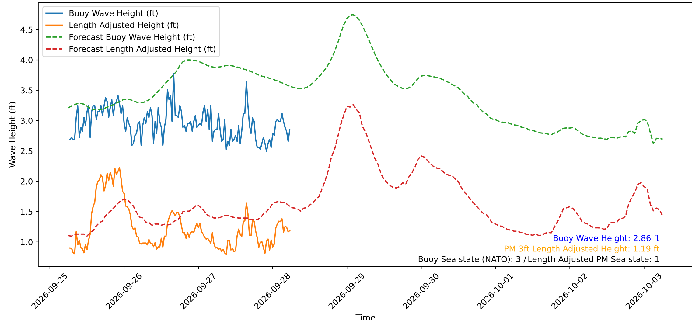
Wave Heights over Time for Oceanside Harbor at 2026-09-28 06:20:29
