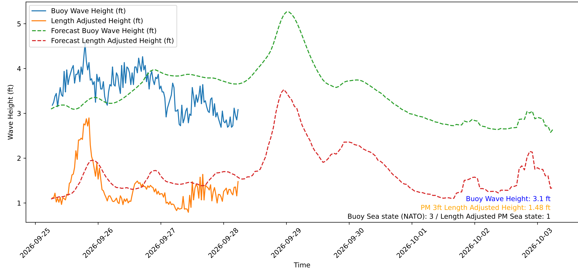
Wave Heights over Time for Green Beach at 2026-09-28 06:21:14
