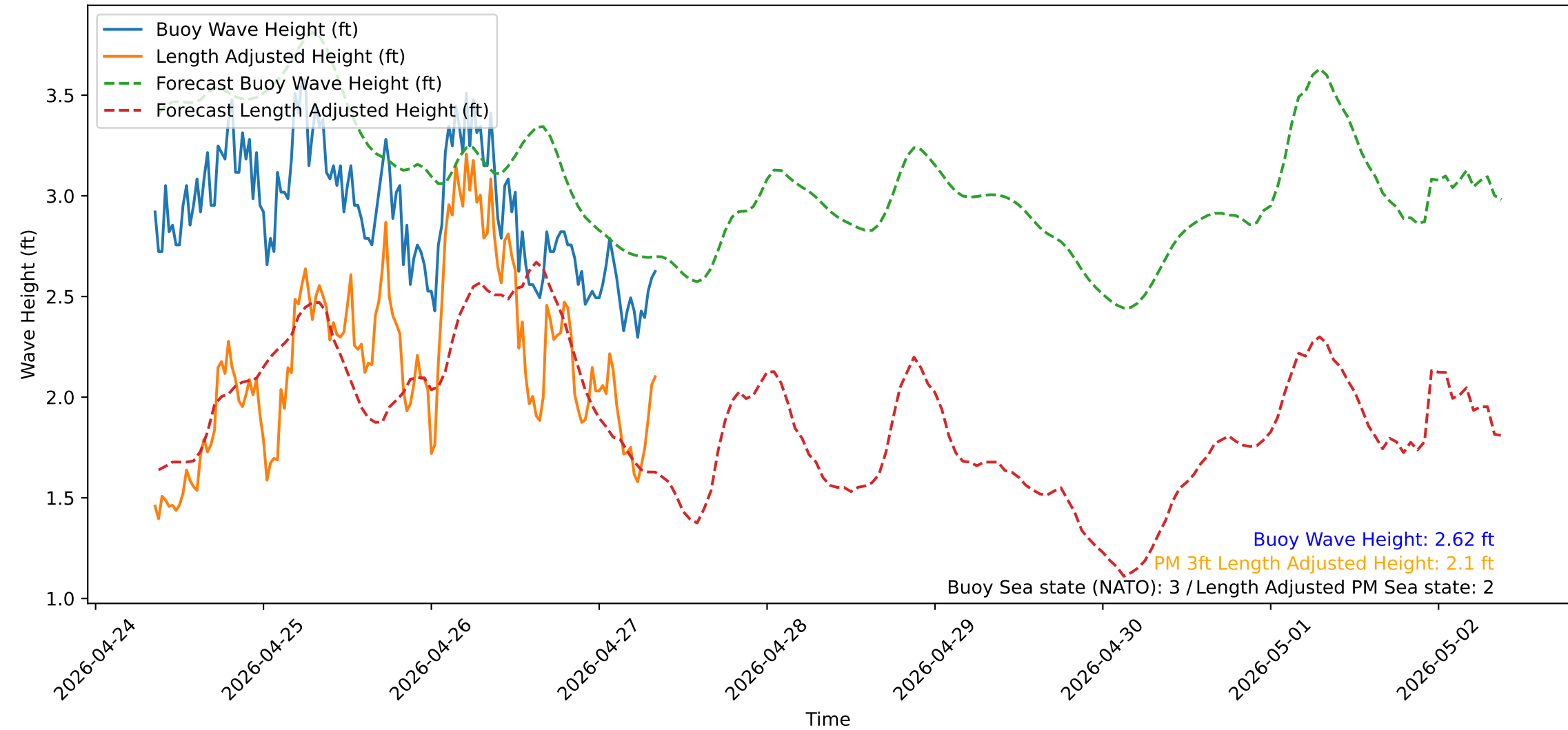
Wave Heights over Time for Green Beach at 2026-04-27 08:41:13
