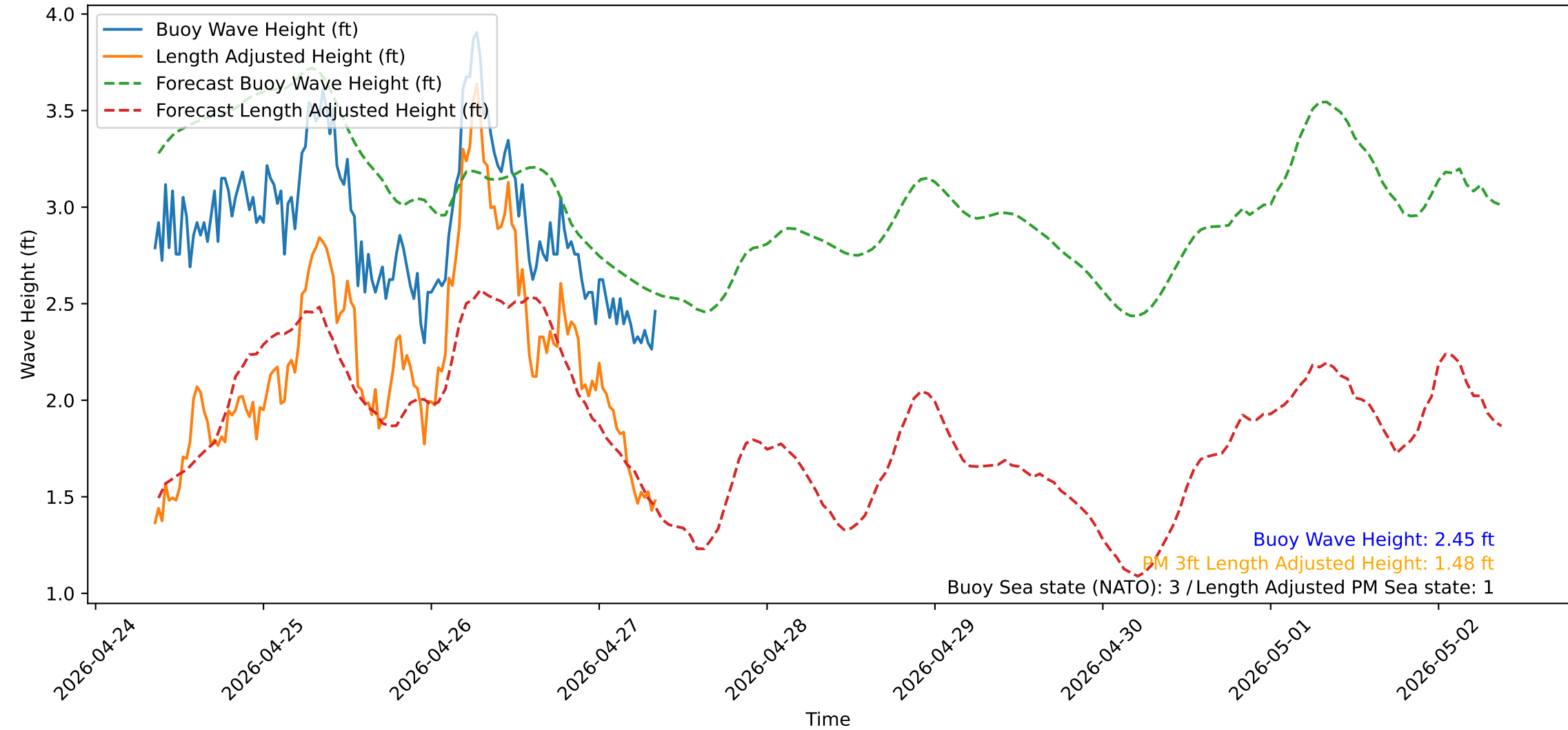
Wave Heights over Time for Oceanside Harbor at 2026-04-27 08:40:31
