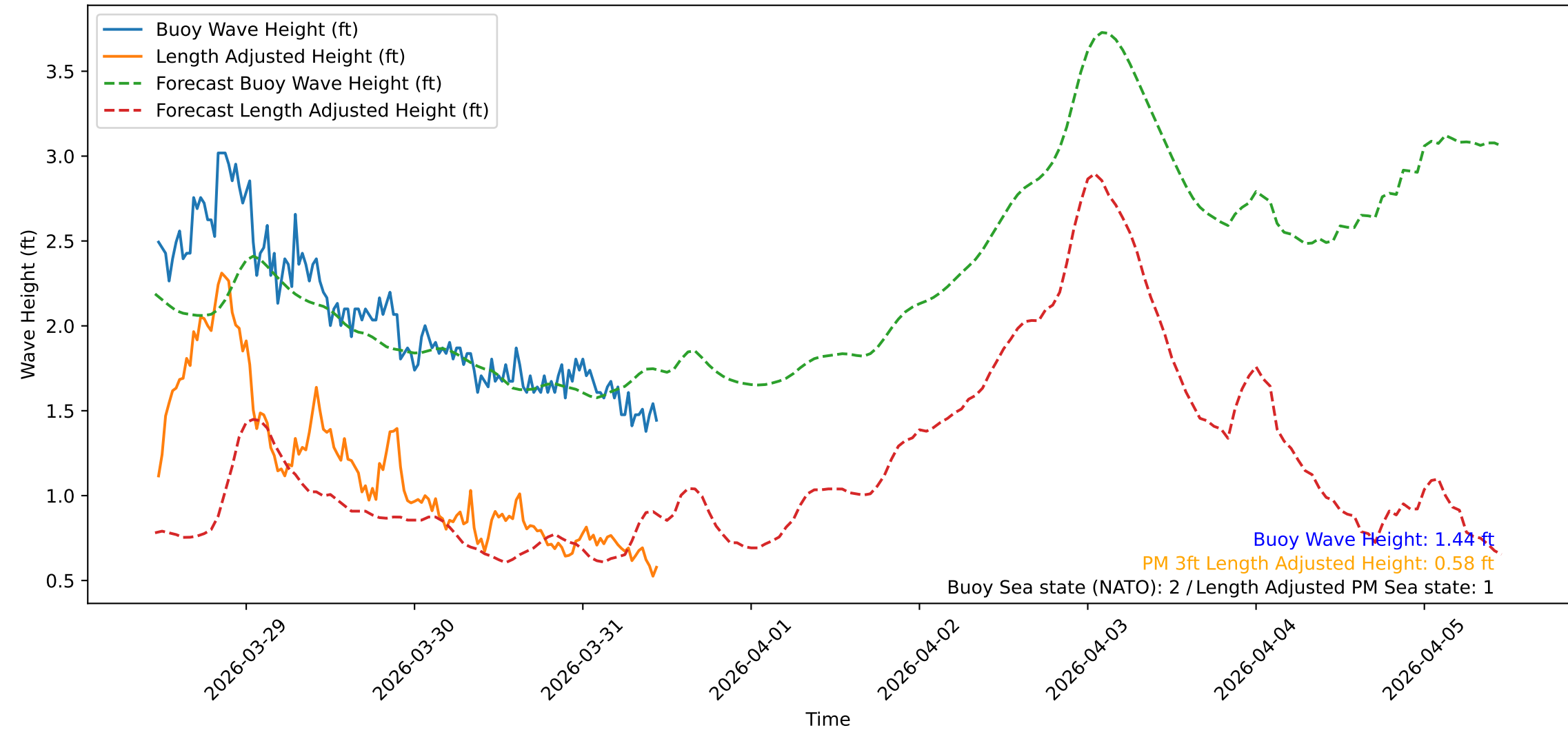
Wave Heights over Time for Red Beach at 2026-03-31 11:10:47
