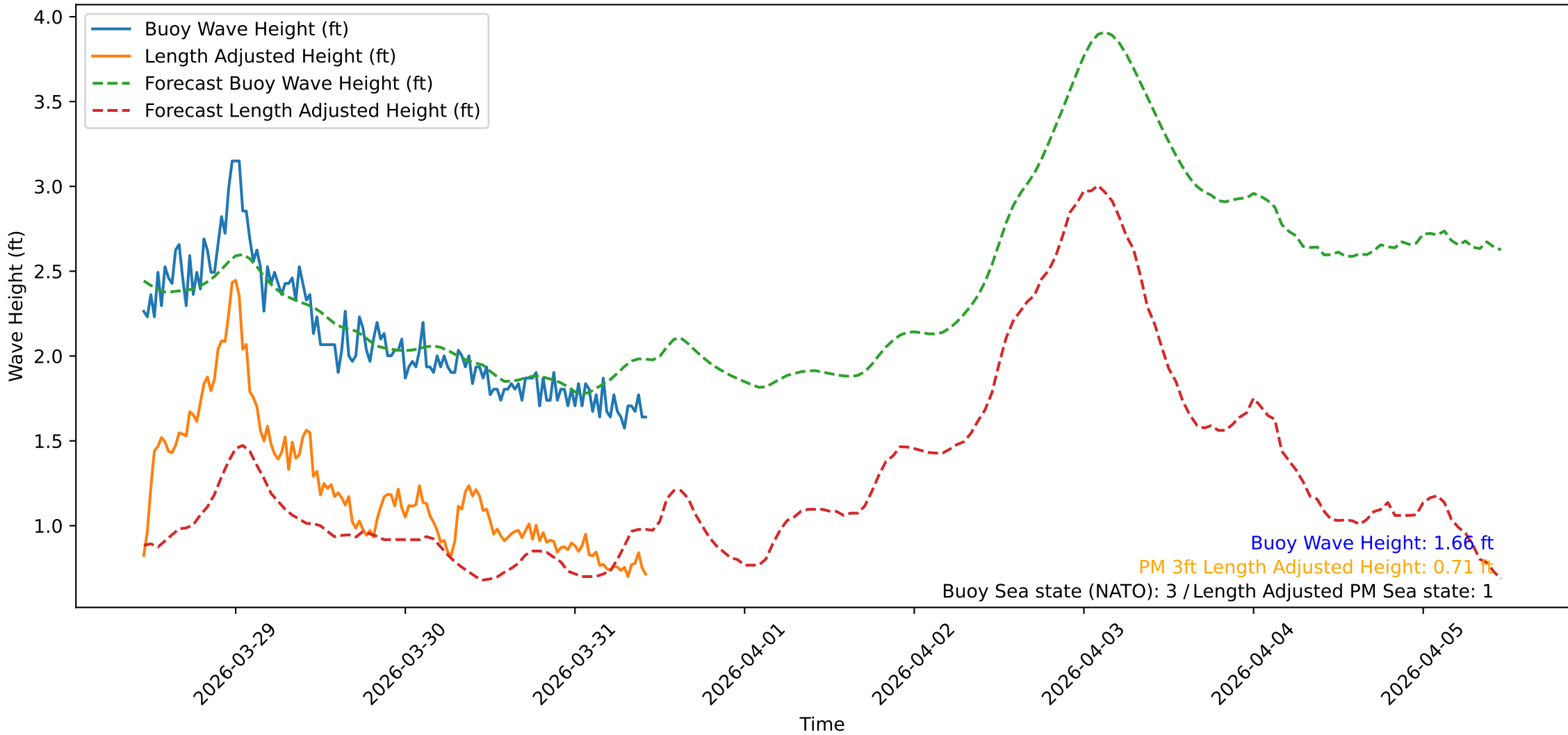
Wave Heights over Time for Oceanside Harbor at 2026-03-31 11:10:31
