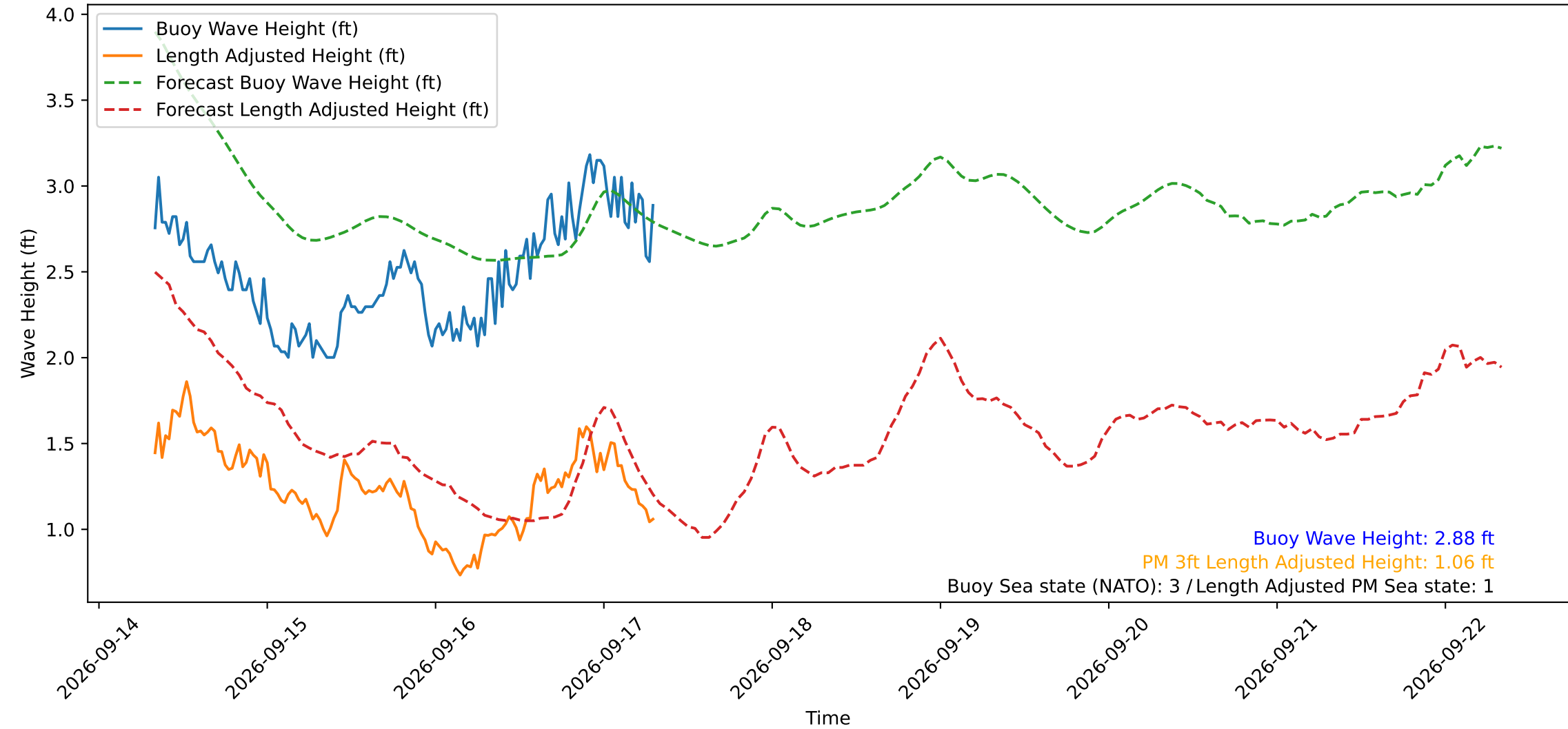
Wave Heights over Time for Red Beach at 2026-09-17 07:40:51
