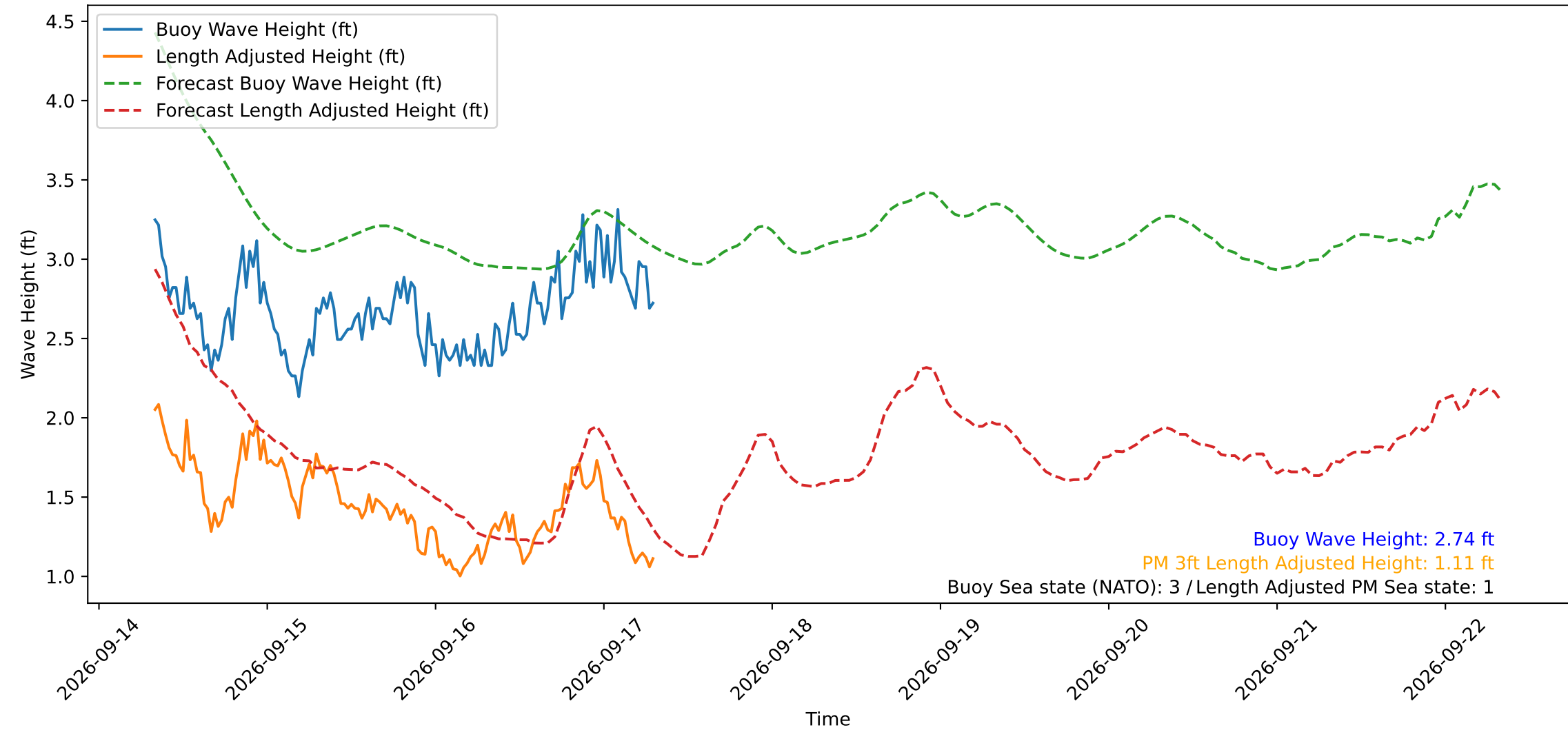
Wave Heights over Time for Green Beach at 2026-09-17 07:41:14
