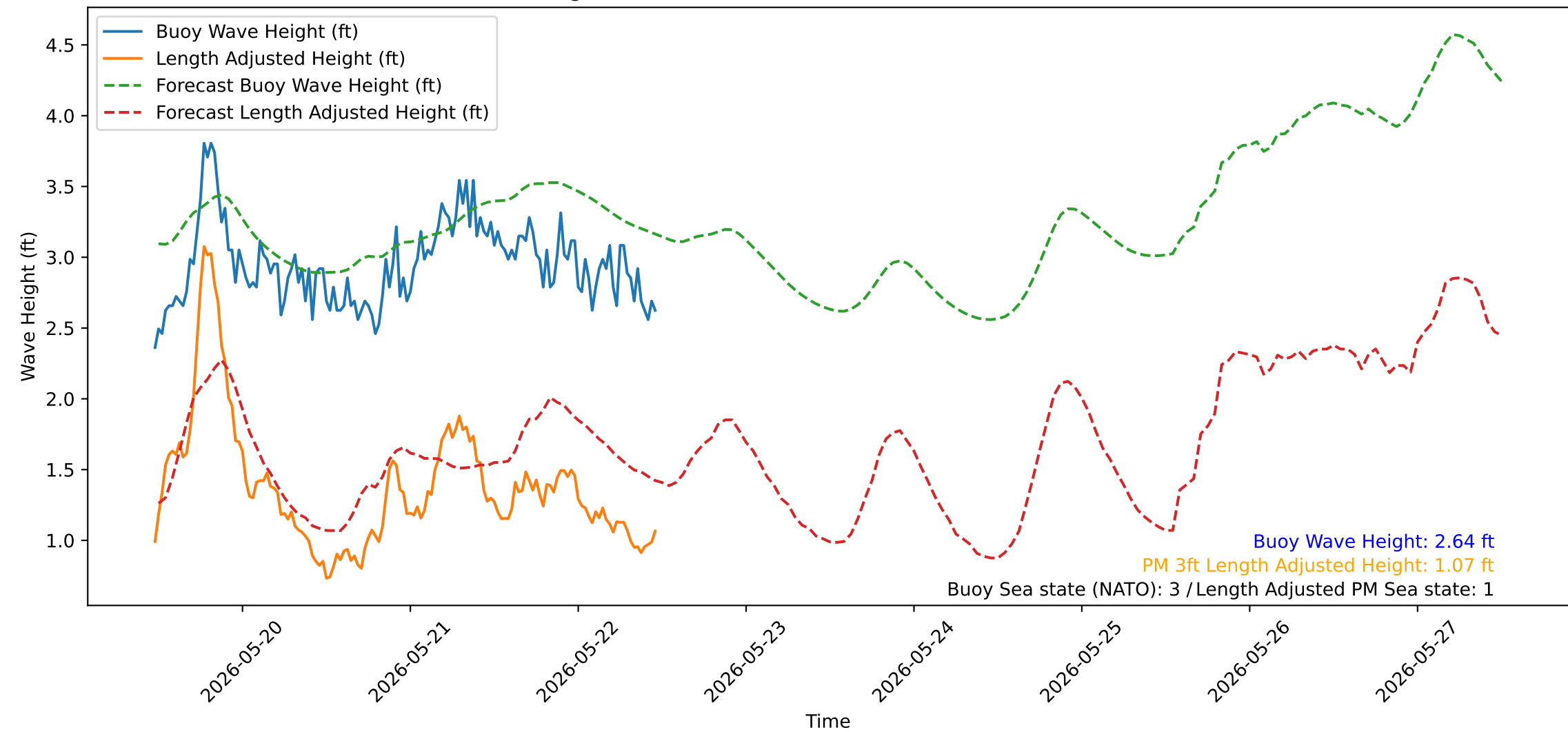
Wave Heights over Time for Green Beach at 2026-05-22 11:41:12
