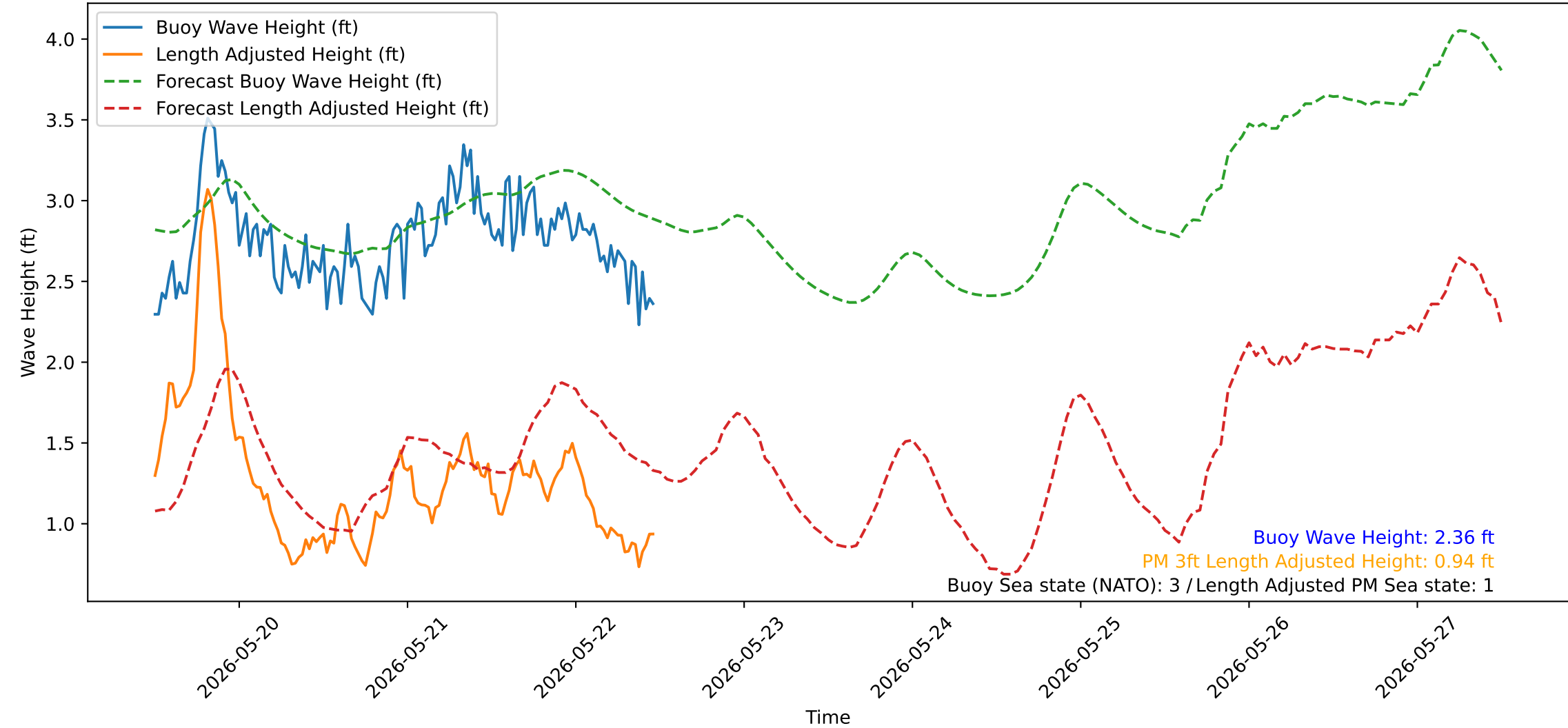
Wave Heights over Time for Red Beach at 2026-05-22 11:40:50
