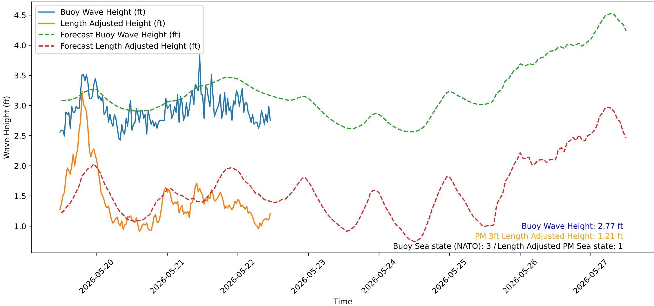
Wave Heights over Time for Oceanside Harbor at 2026-05-22 11:40:31
