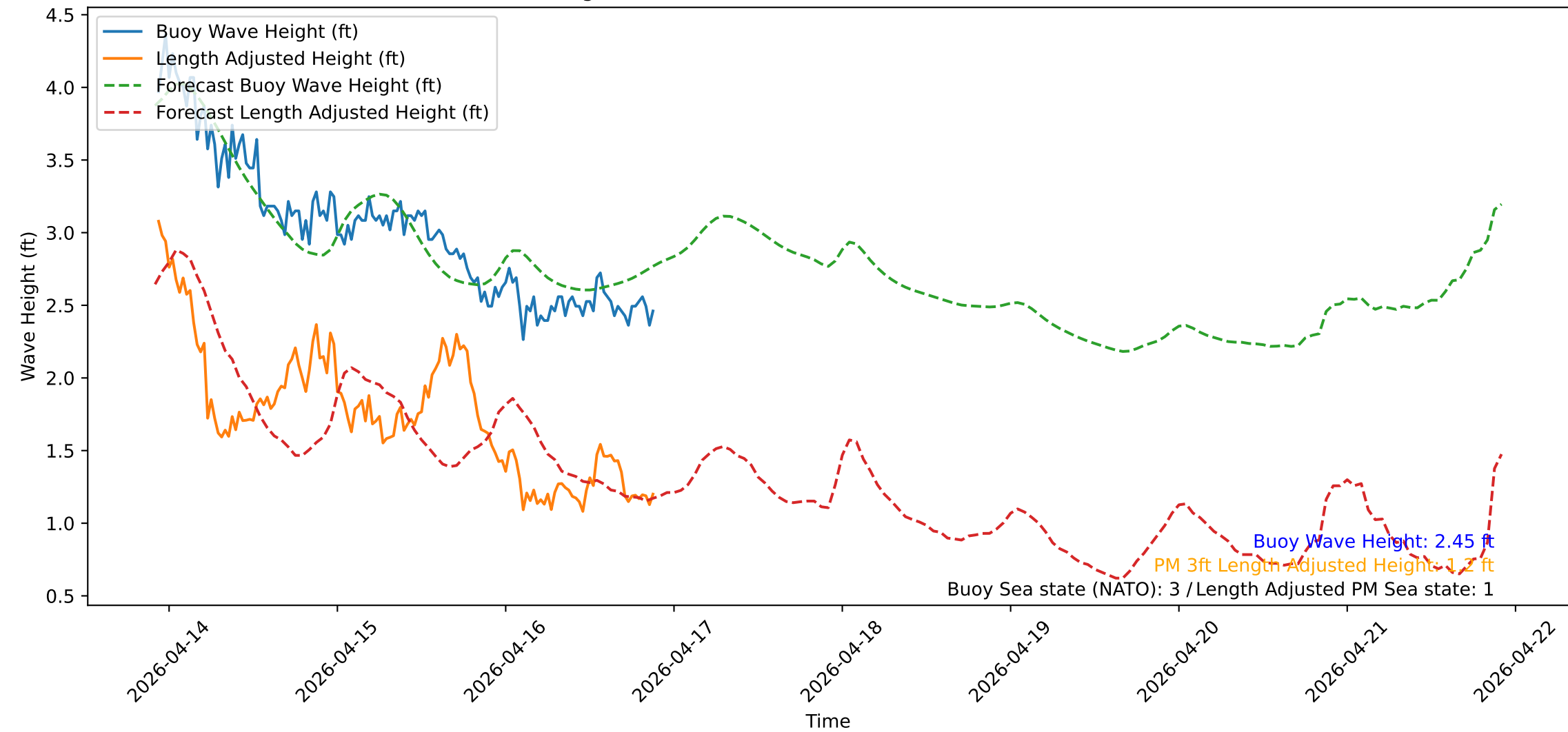
Wave Heights over Time for Red Beach at 2026-04-16 22:00:50
