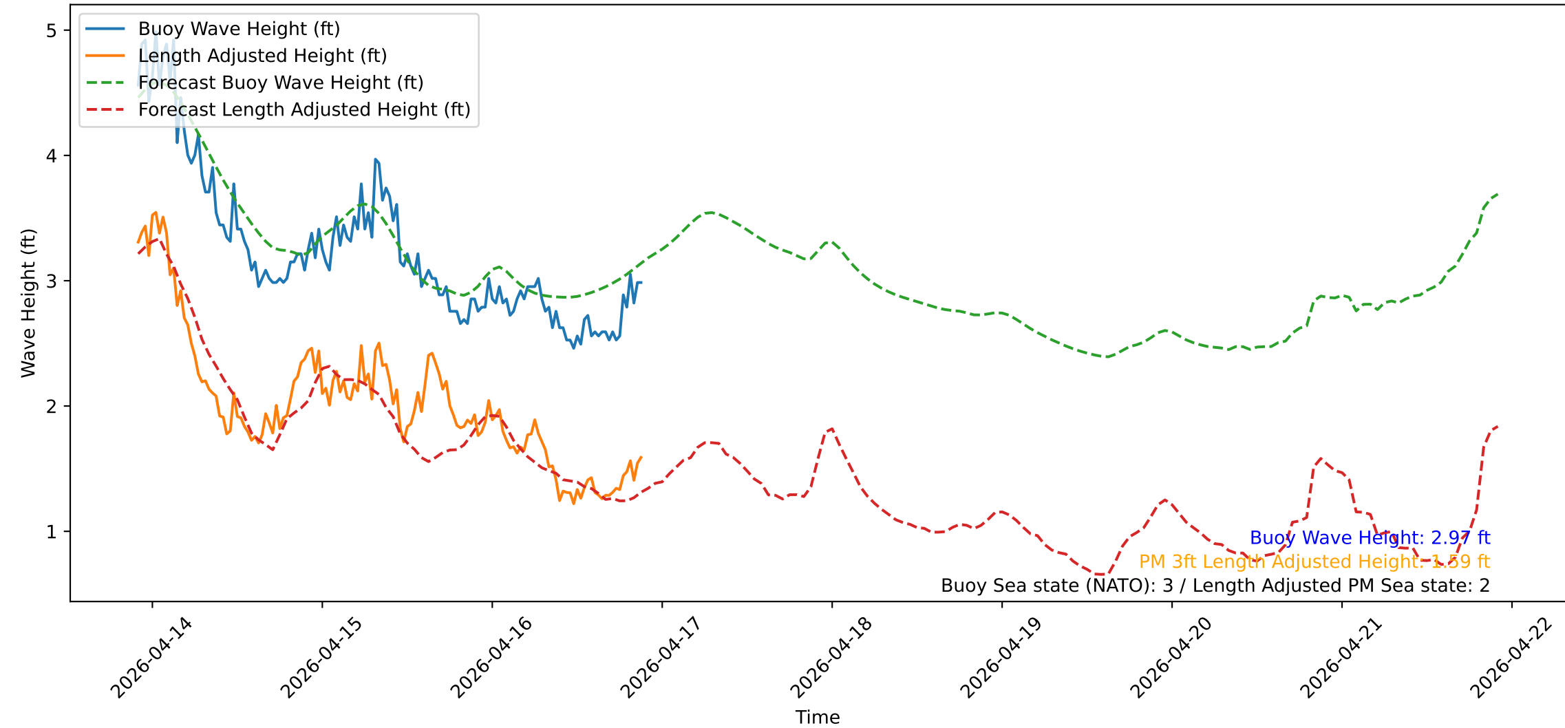
Wave Heights over Time for Green Beach at 2026-04-16 22:01:13
