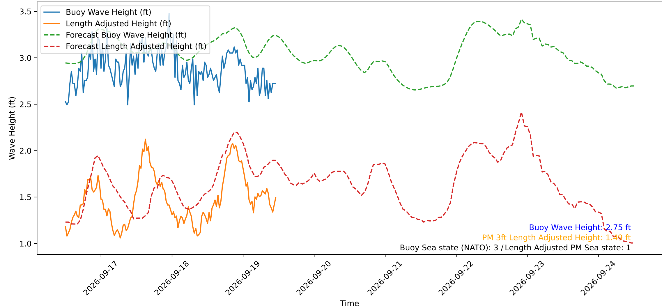
Wave Heights over Time for Green Beach at 2026-09-19 11:41:11
