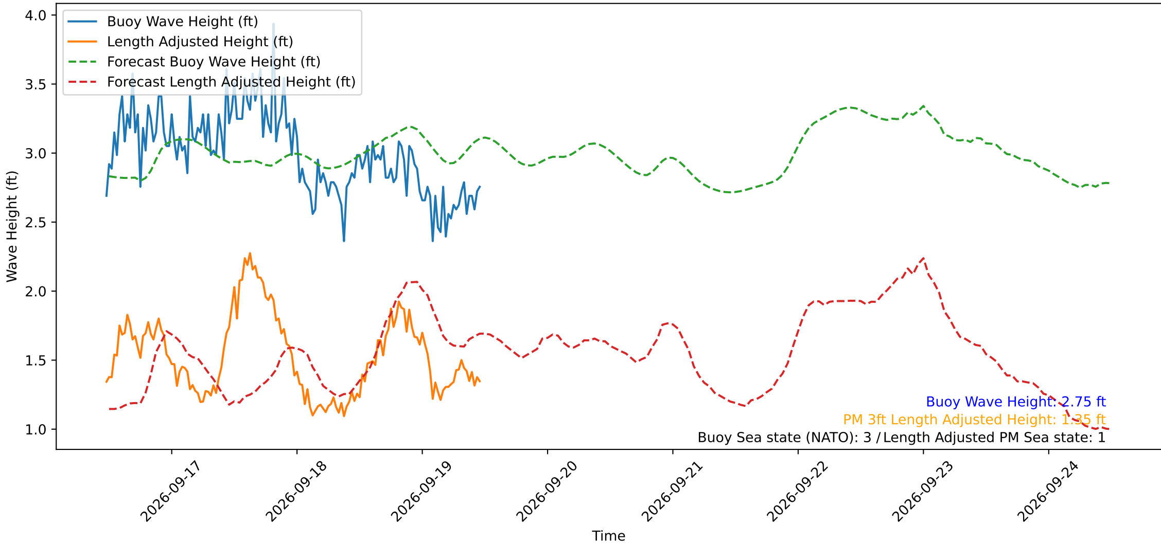
Wave Heights over Time for Oceanside Harbor at 2026-09-19 11:40:29
