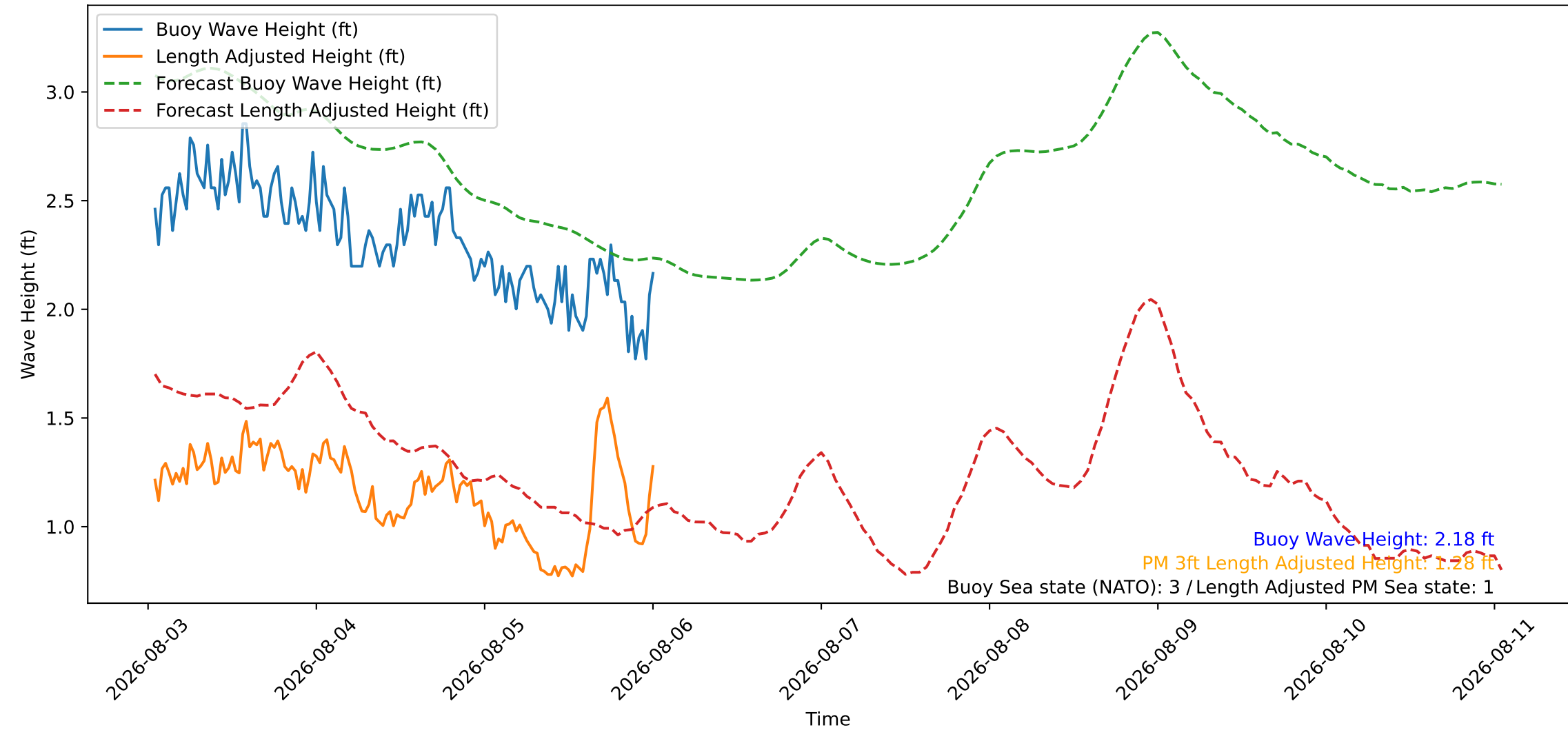
Wave Heights over Time for Oceanside Harbor at 2026-08-06 00:50:26
