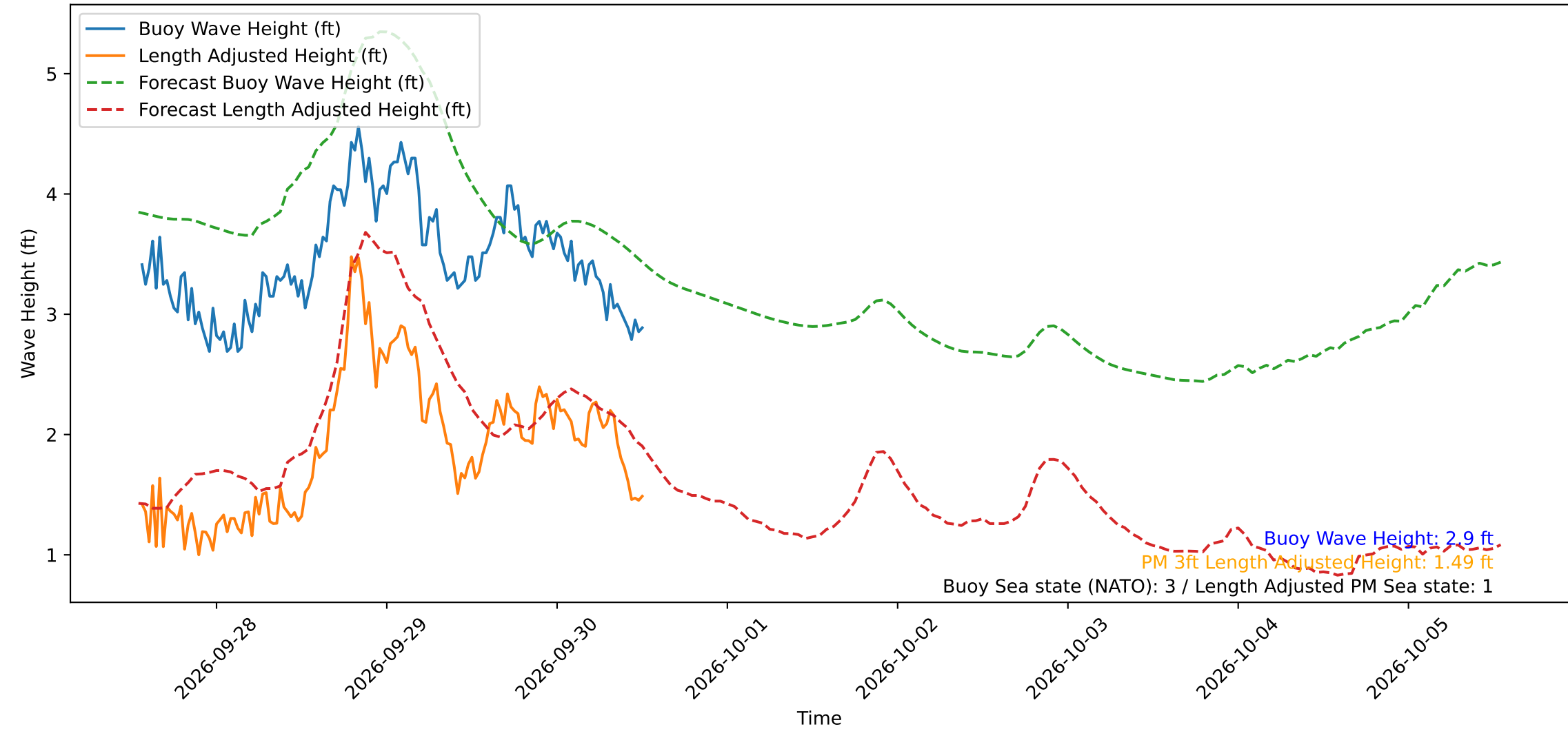
Wave Heights over Time for Green Beach at 2026-09-30 13:11:11
