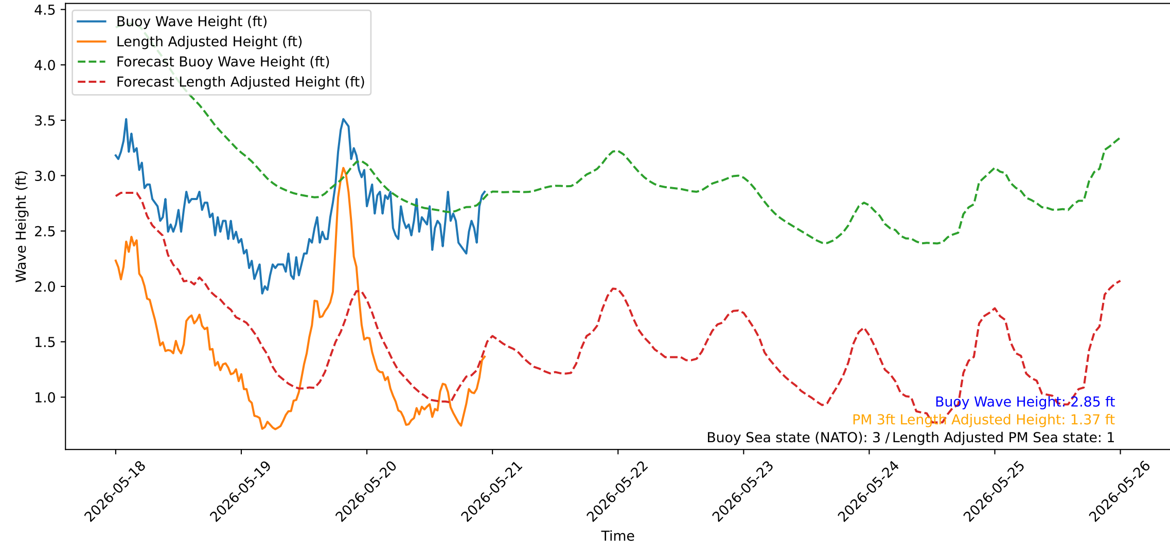
Wave Heights over Time for Red Beach at 2026-05-20 23:30:51
