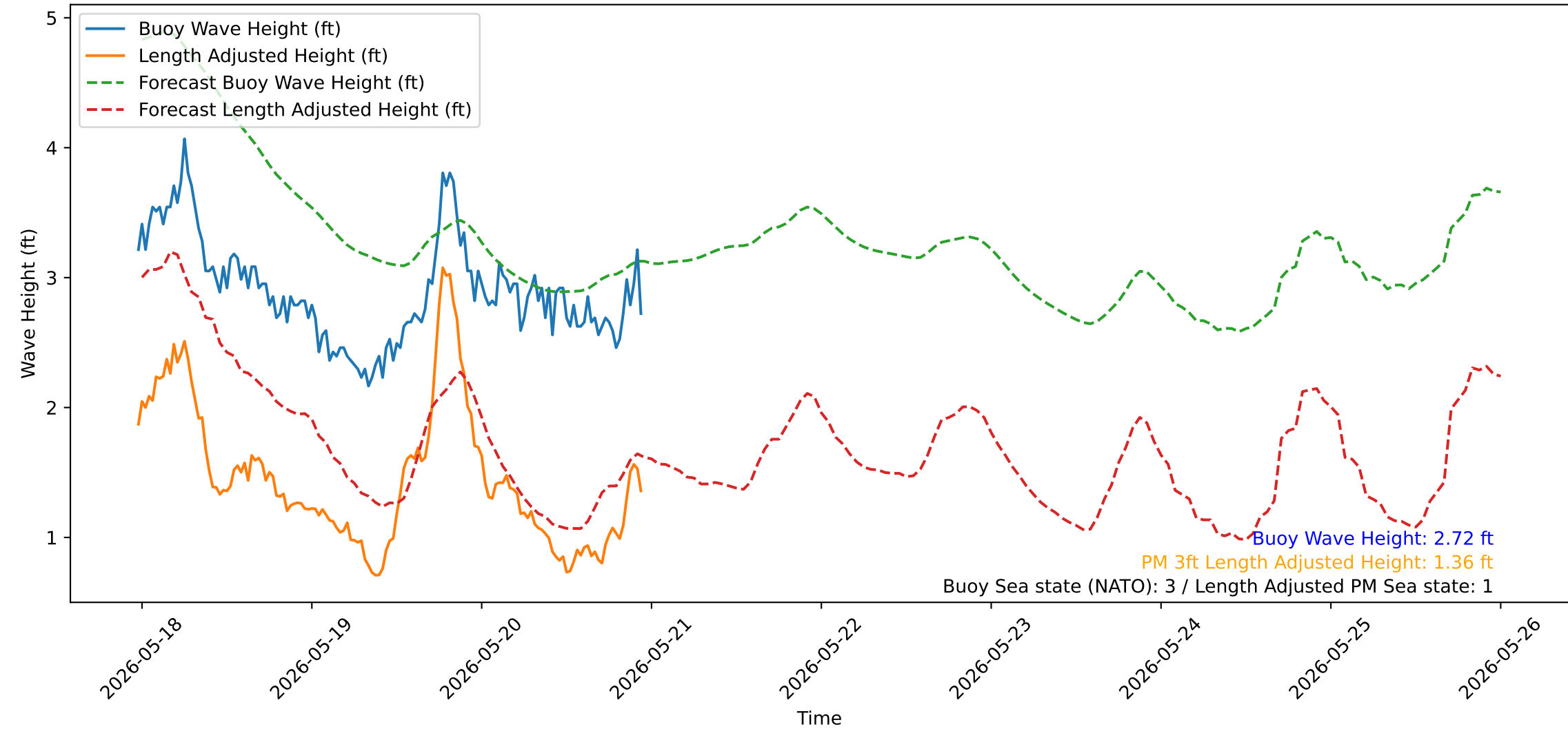
Wave Heights over Time for Green Beach at 2026-05-20 23:31:14
