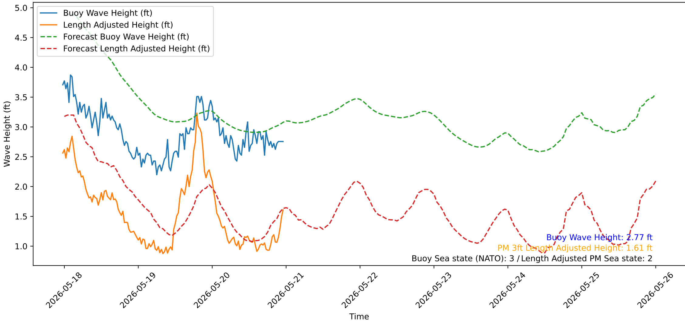
Wave Heights over Time for Oceanside Harbor at 2026-05-20 23:30:32
