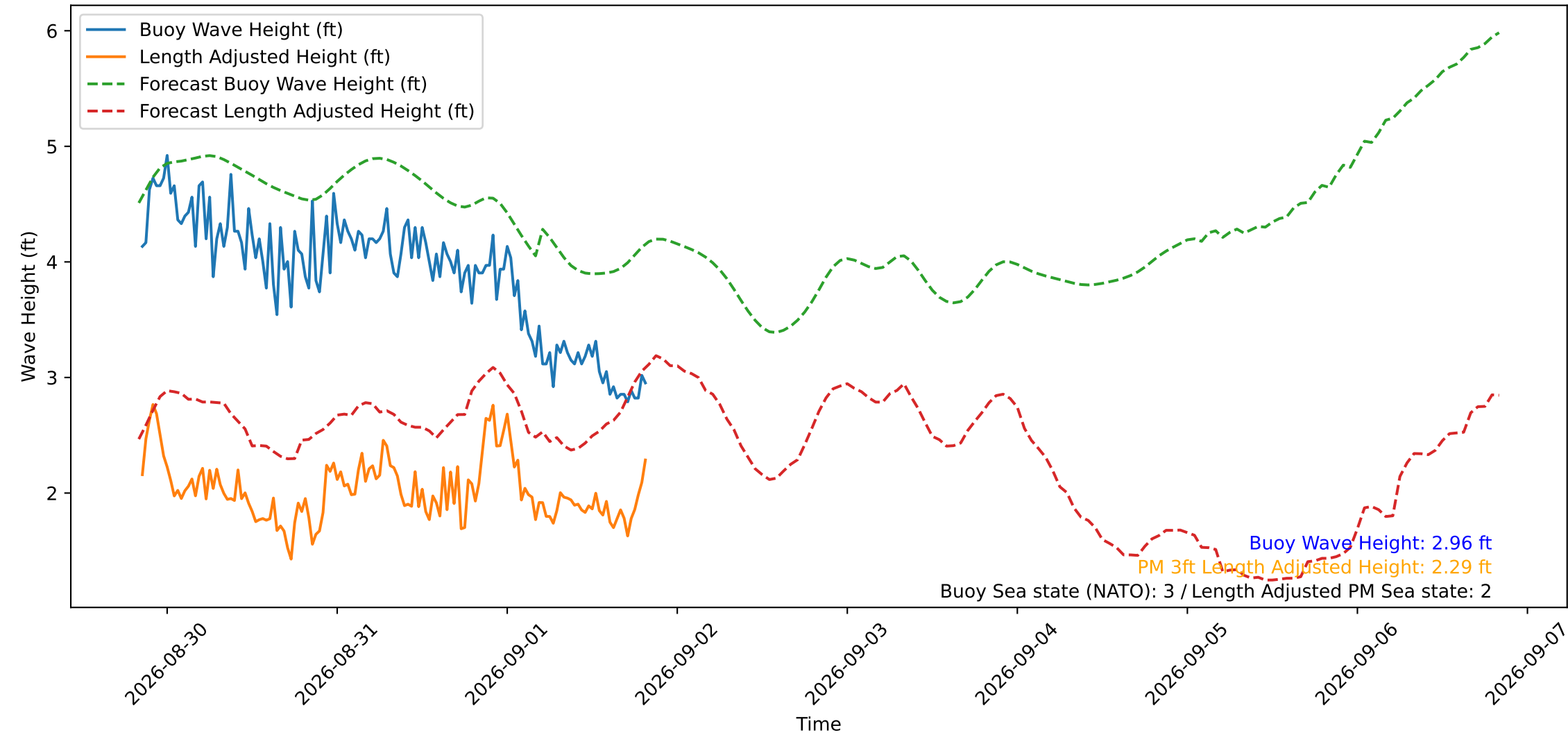
Wave Heights over Time for Green Beach at 2026-09-01 20:21:15
