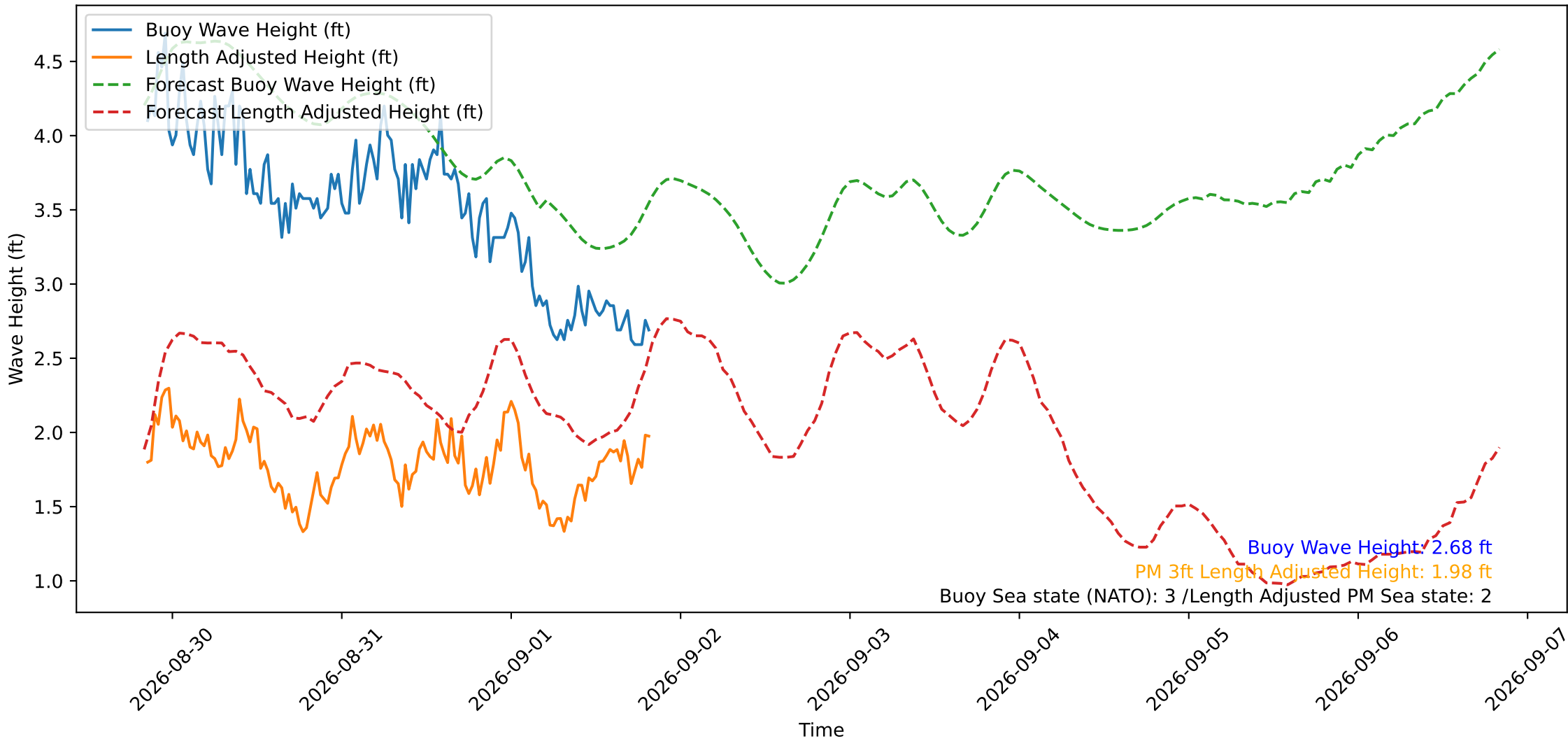
Wave Heights over Time for Red Beach at 2026-09-01 20:20:50
