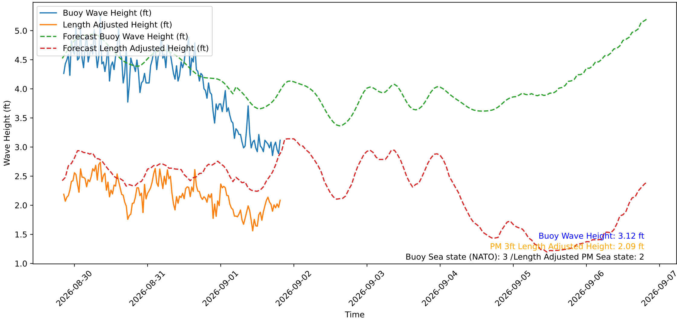
Wave Heights over Time for Oceanside Harbor at 2026-09-01 20:20:29
