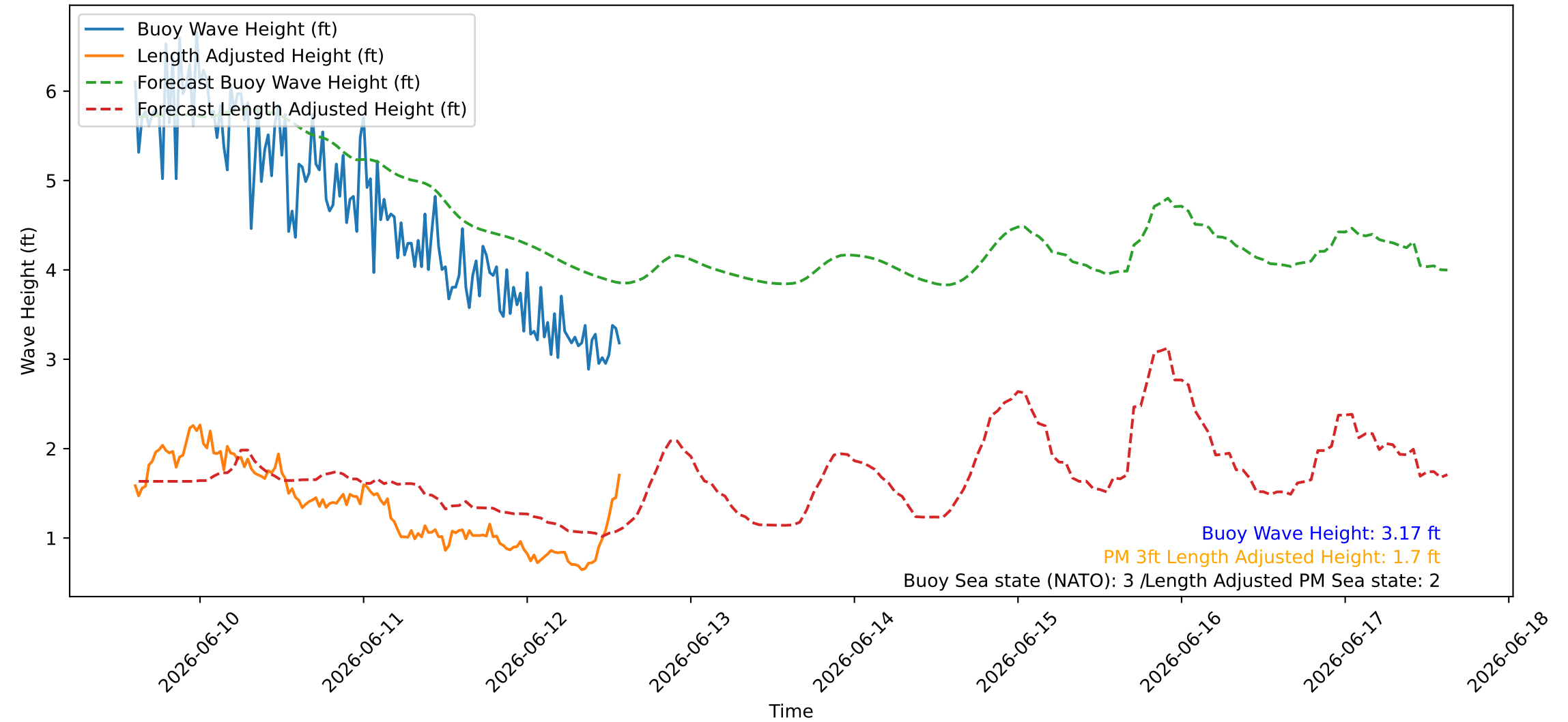
Wave Heights over Time for Green Beach at 2026-06-12 14:31:08
