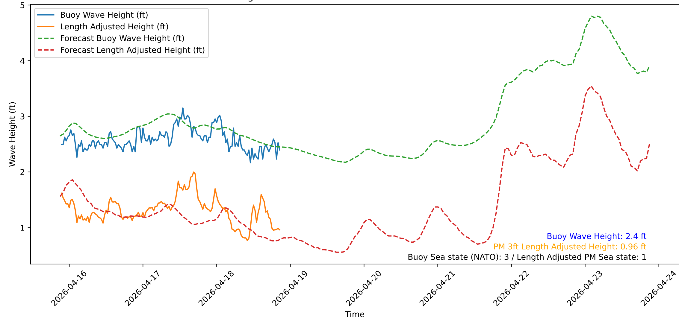
Wave Heights over Time for Red Beach at 2026-04-18 21:20:51
