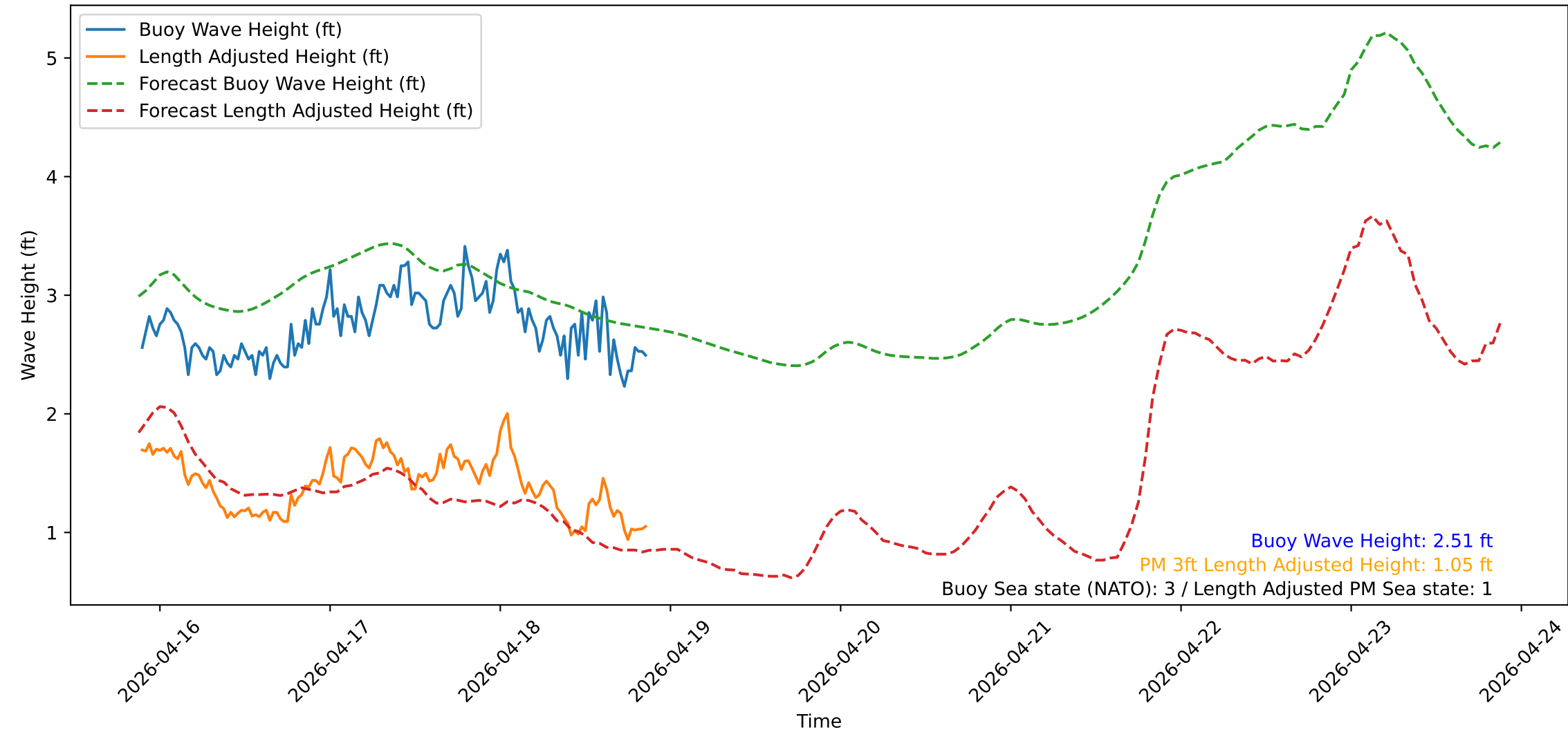
Wave Heights over Time for Oceanside Harbor at 2026-04-18 21:20:31
