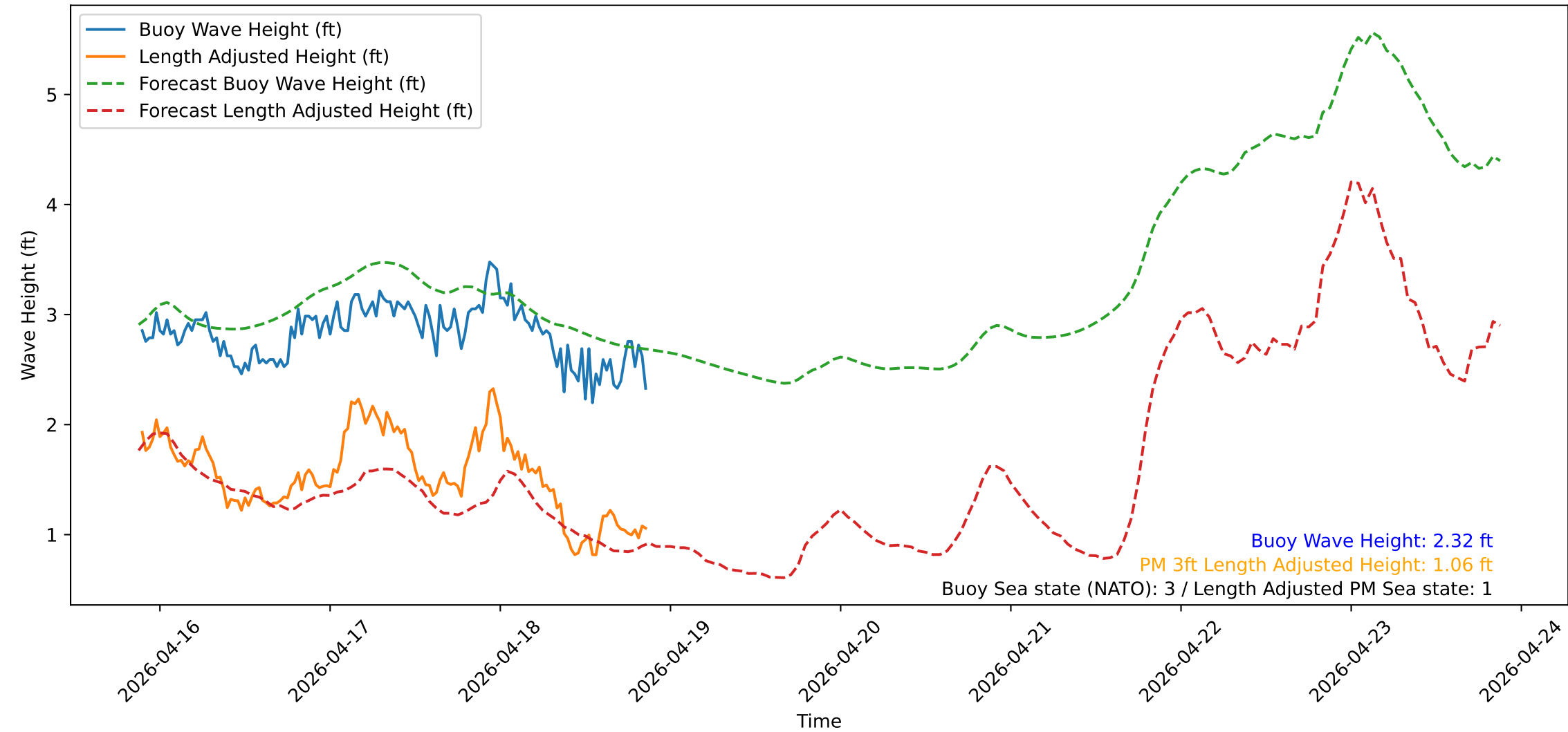
Wave Heights over Time for Green Beach at 2026-04-18 21:21:13
