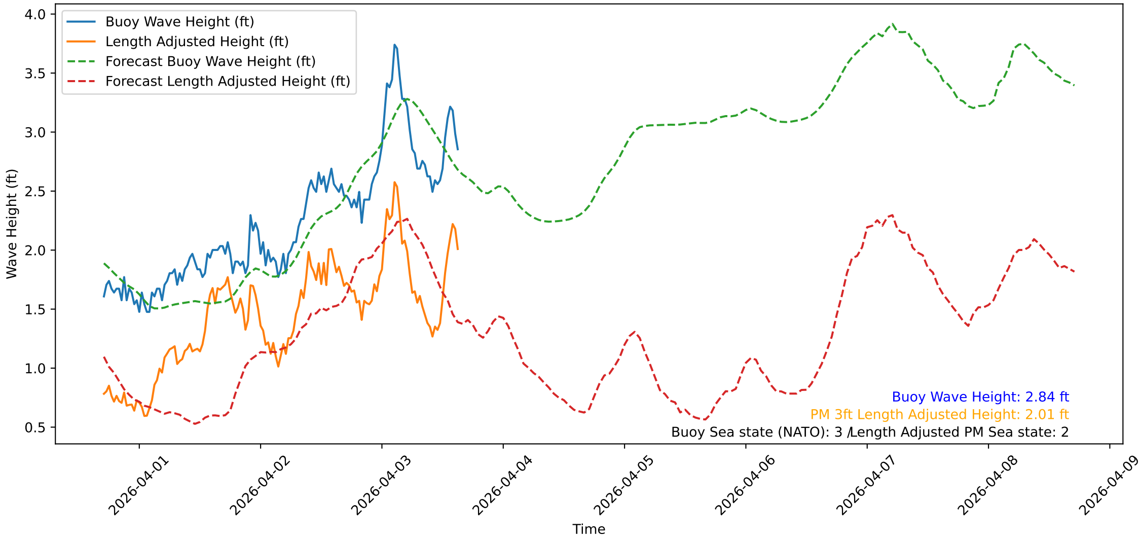
Wave Heights over Time for Red Beach at 2026-04-03 16:30:47
