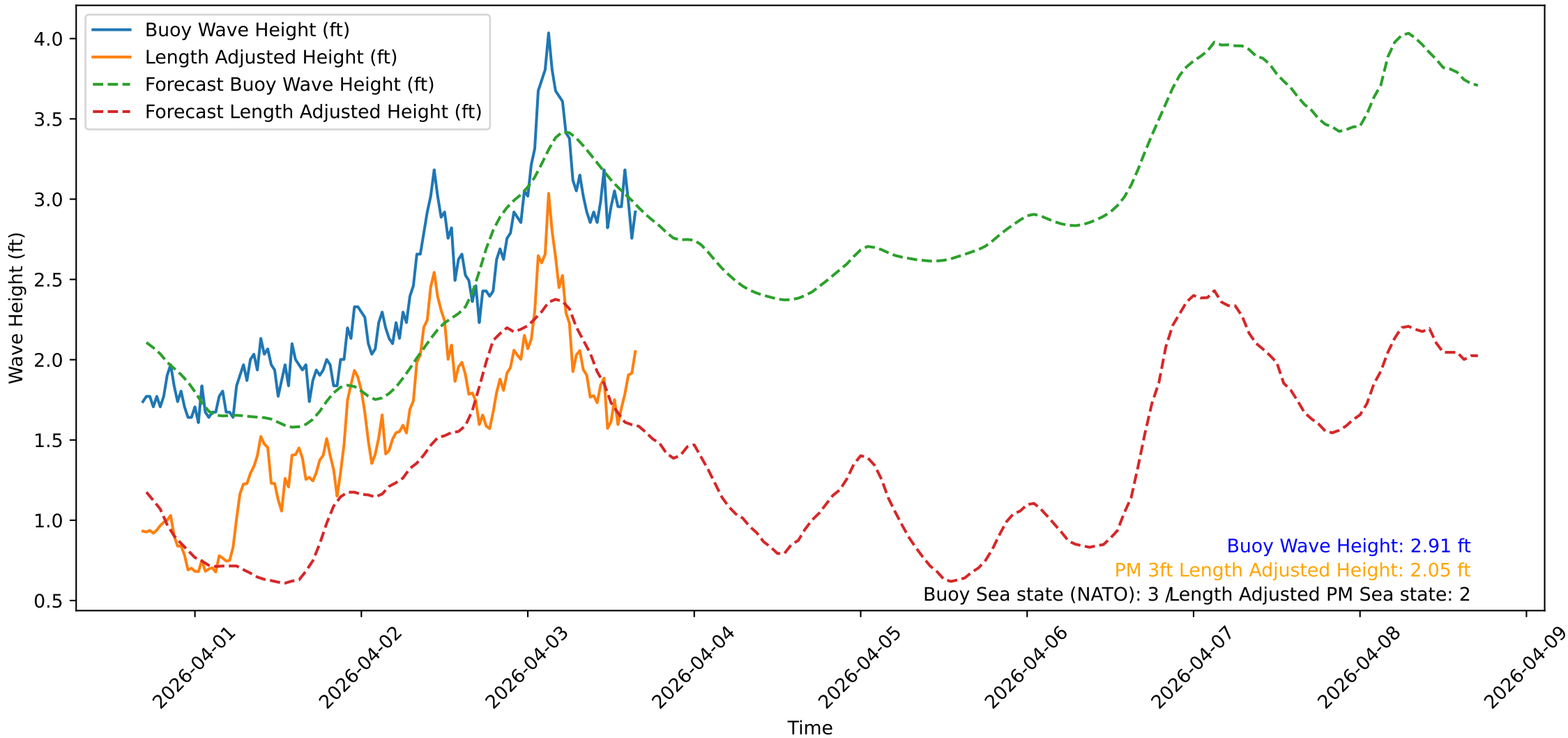
Wave Heights over Time for Oceanside Harbor at 2026-04-03 16:30:31
