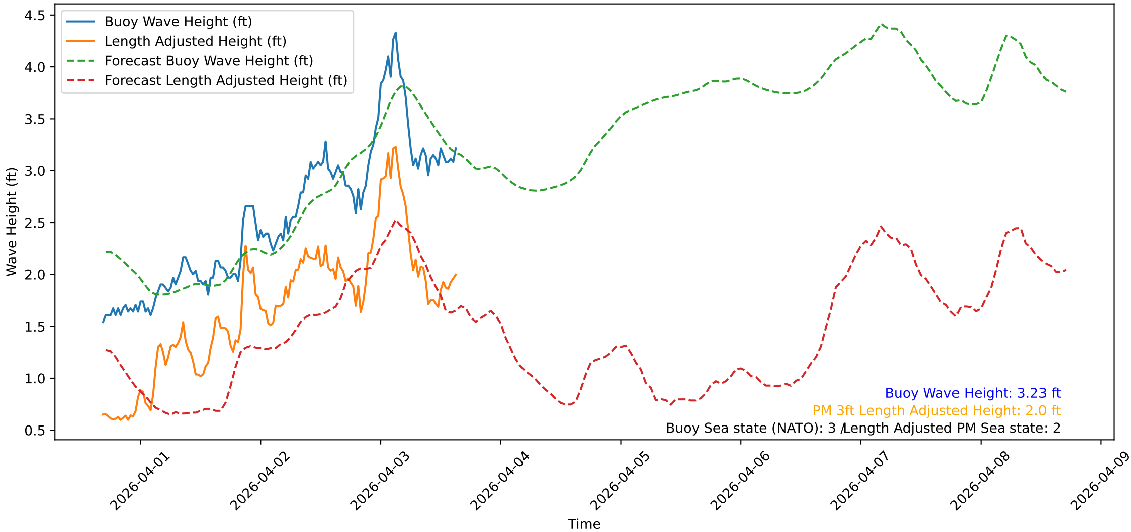
Wave Heights over Time for Green Beach at 2026-04-03 16:31:10
