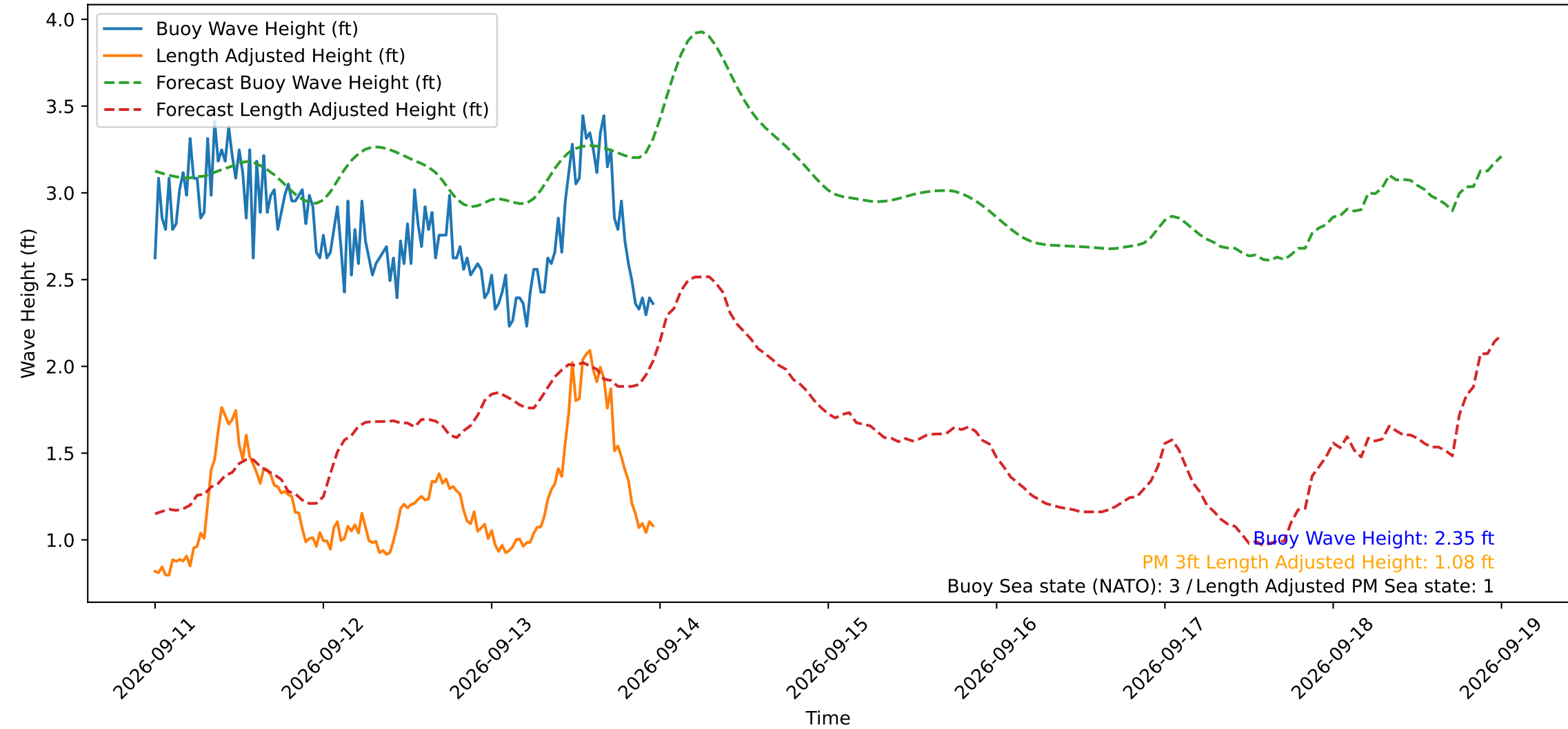
Wave Heights over Time for Red Beach at 2026-09-13 23:50:50
