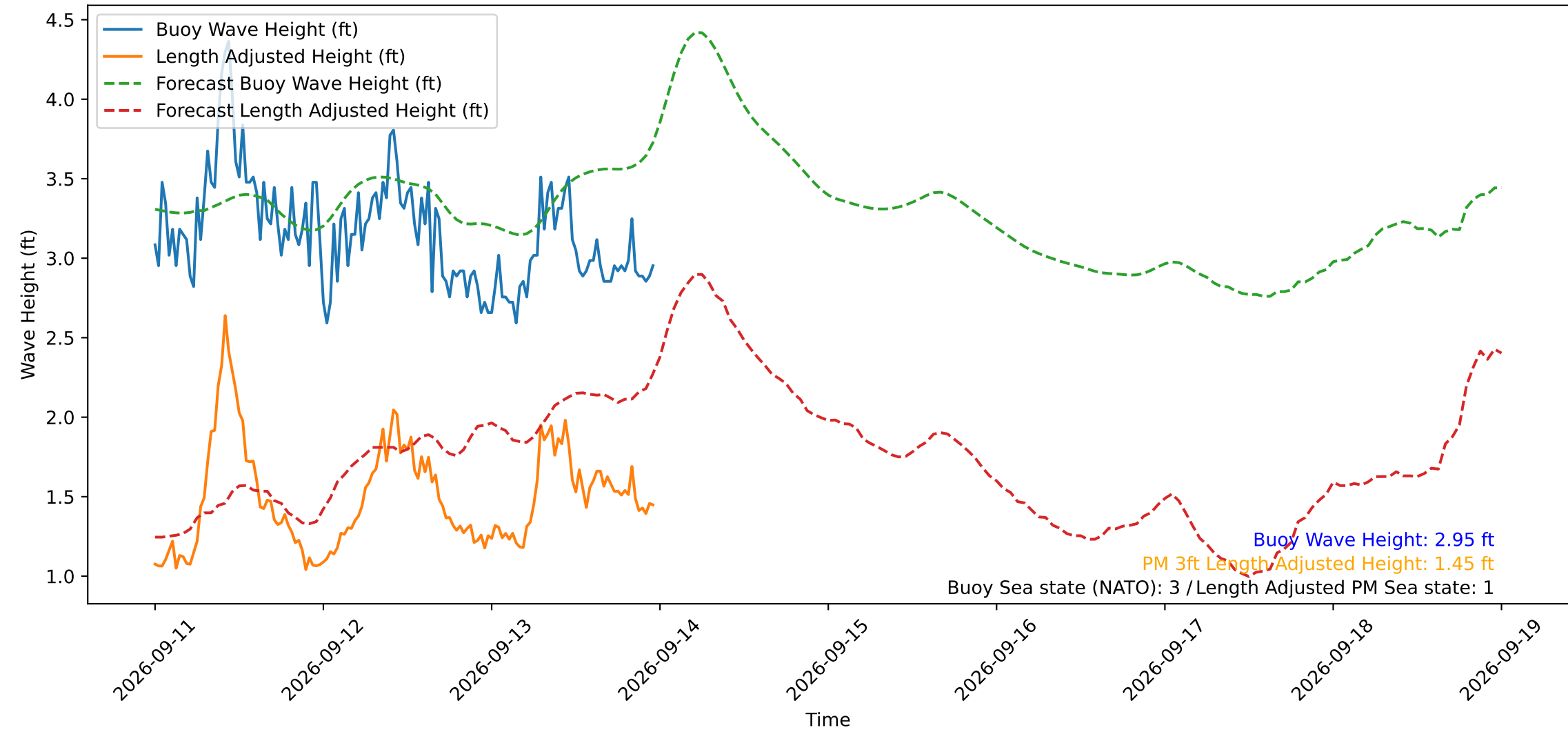
Wave Heights over Time for Oceanside Harbor at 2026-09-13 23:50:30
