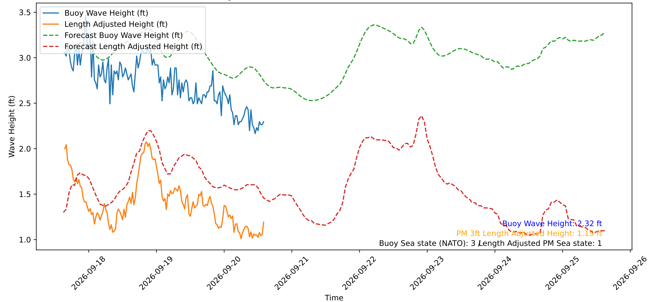
Wave Heights over Time for Green Beach at 2026-09-20 15:01:13
