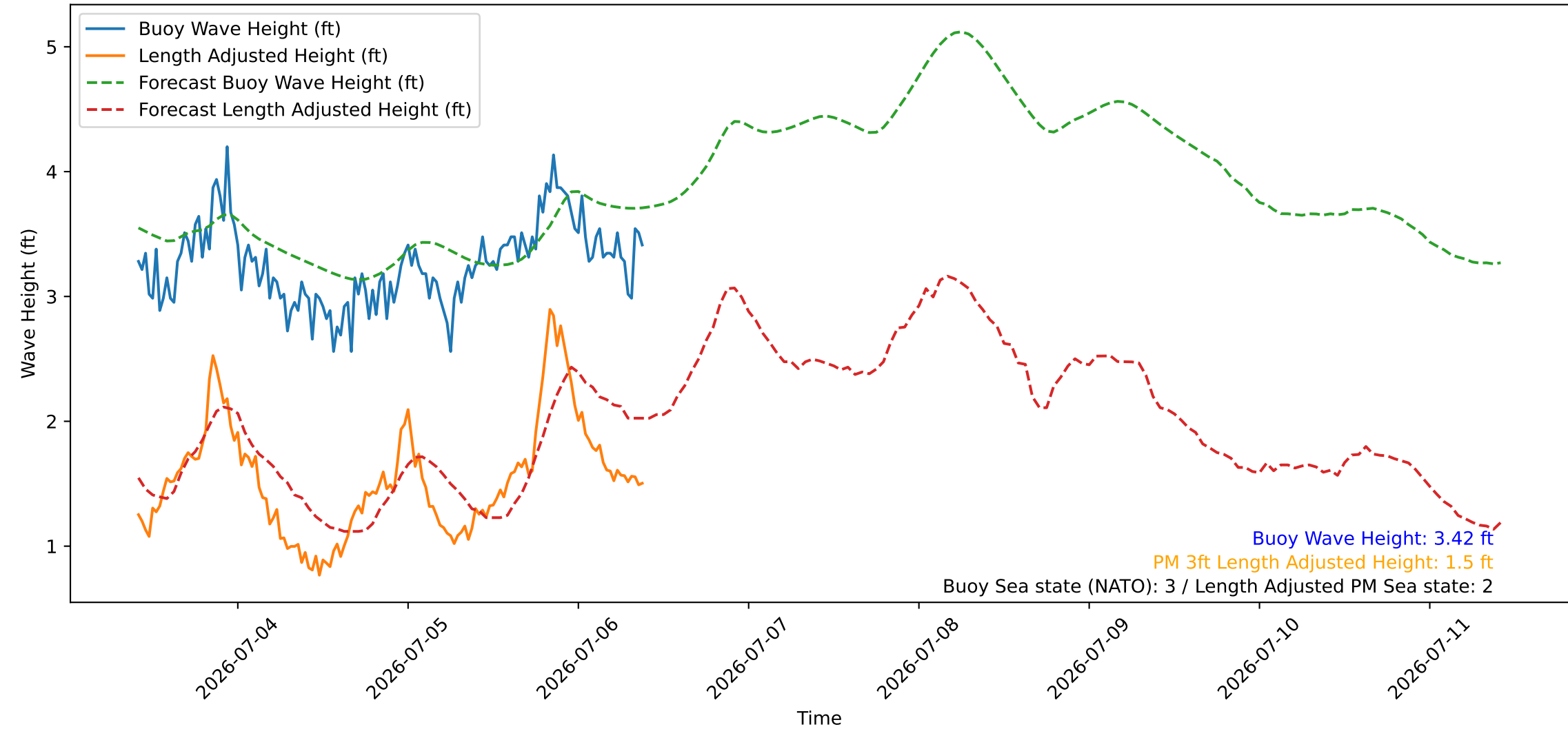
Wave Heights over Time for Green Beach at 2026-07-06 10:01:08
