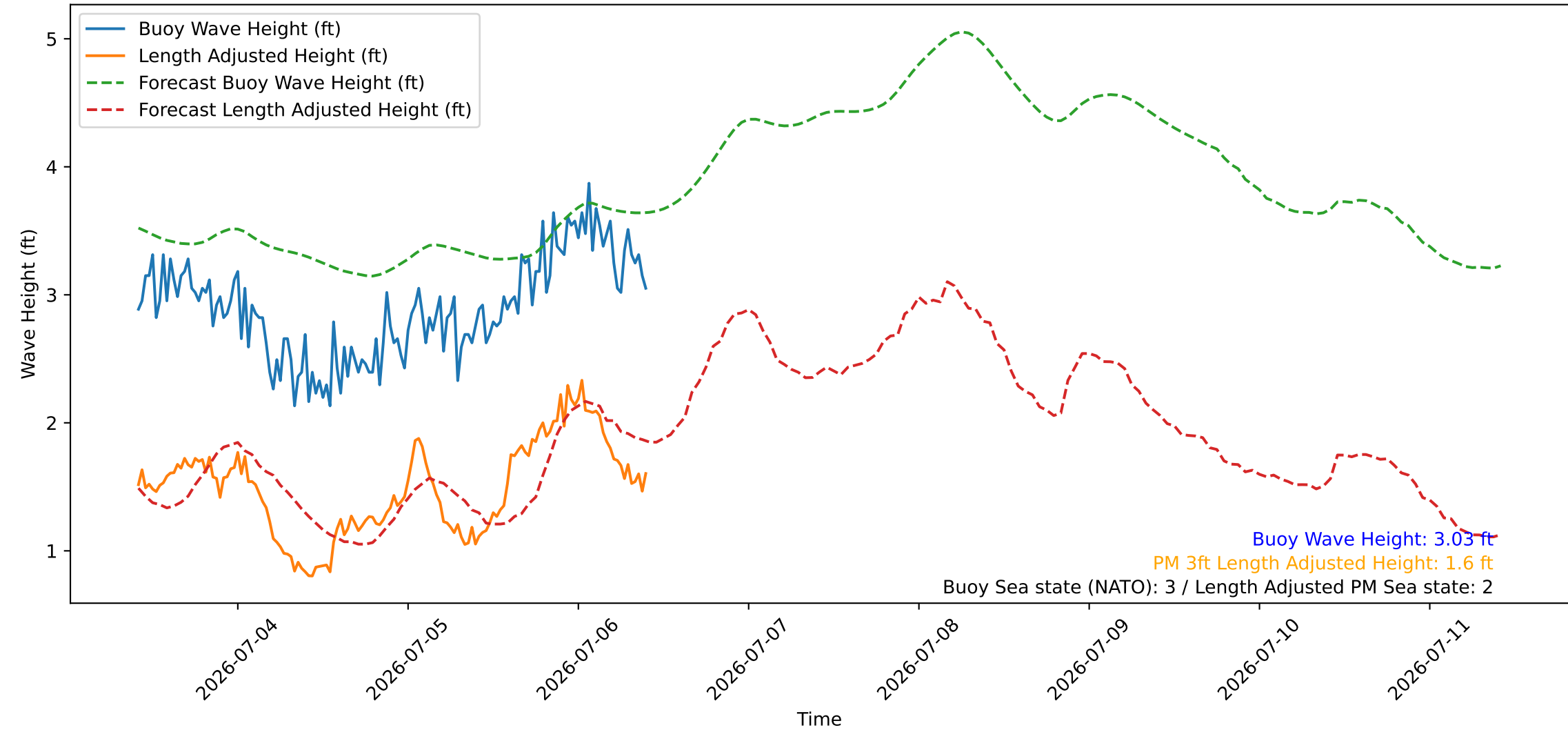
Wave Heights over Time for Oceanside Harbor at 2026-07-06 10:00:26
