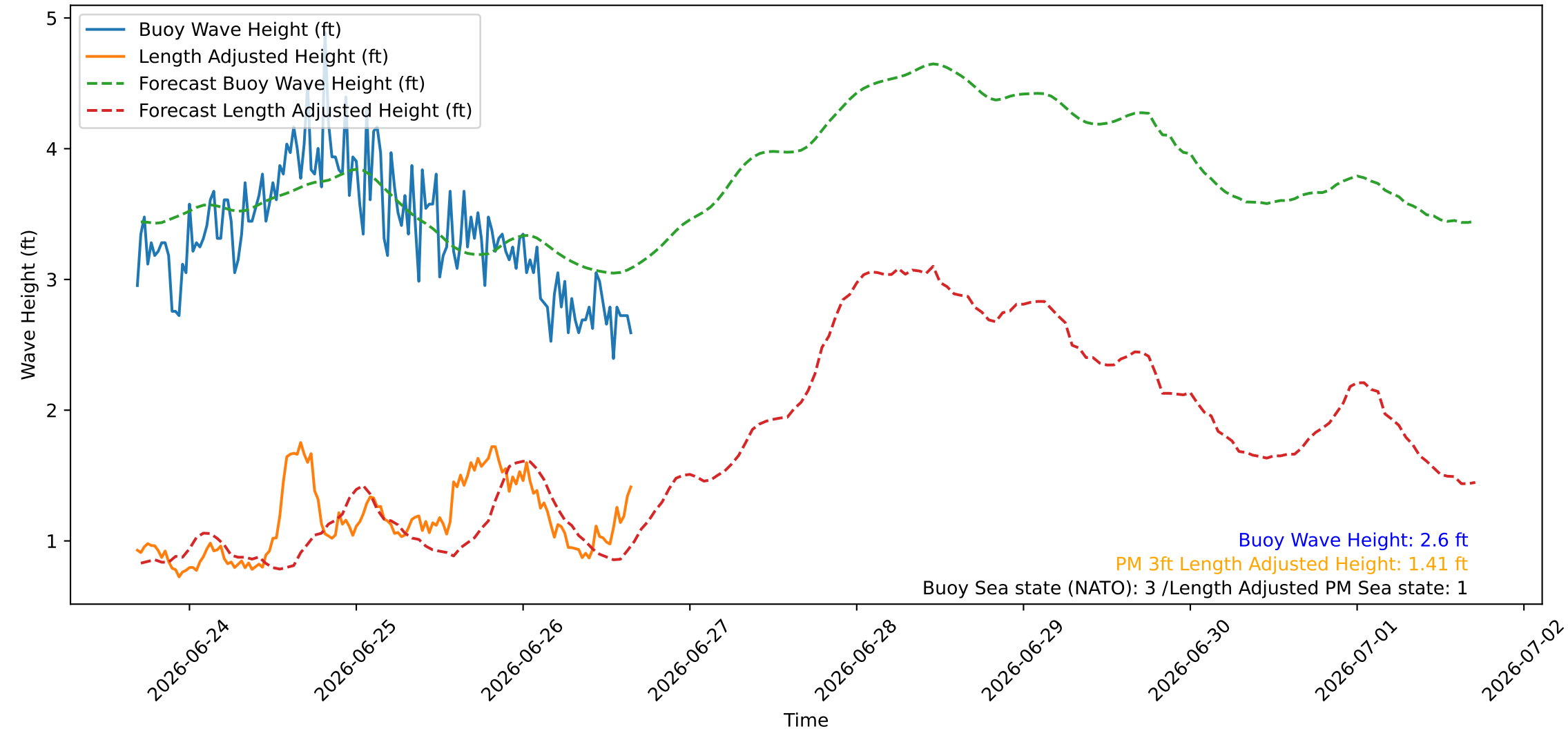
Wave Heights over Time for Oceanside Harbor at 2026-06-26 16:30:26
