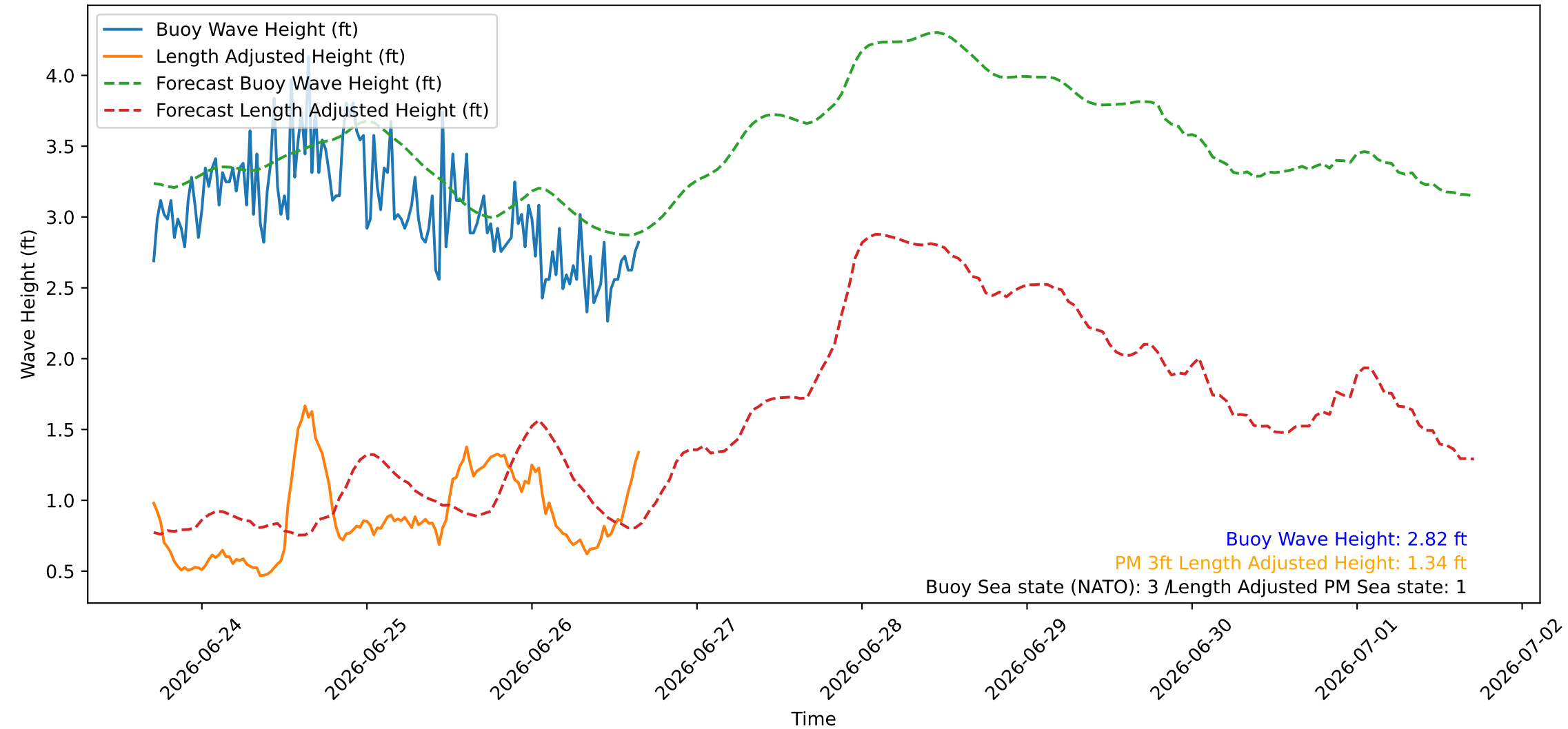
Wave Heights over Time for Red Beach at 2026-06-26 16:30:45
