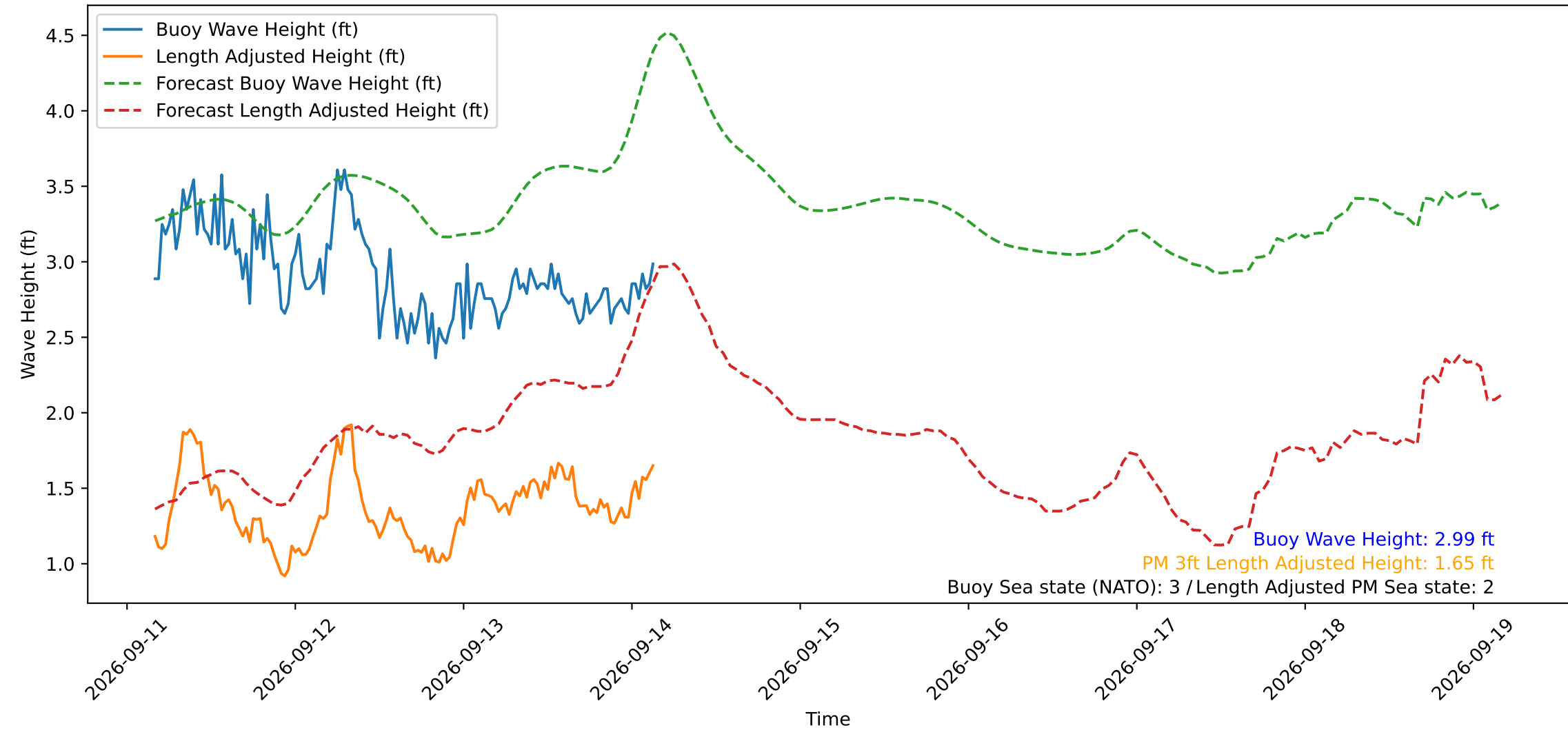
Wave Heights over Time for Green Beach at 2026-09-14 03:41:13
