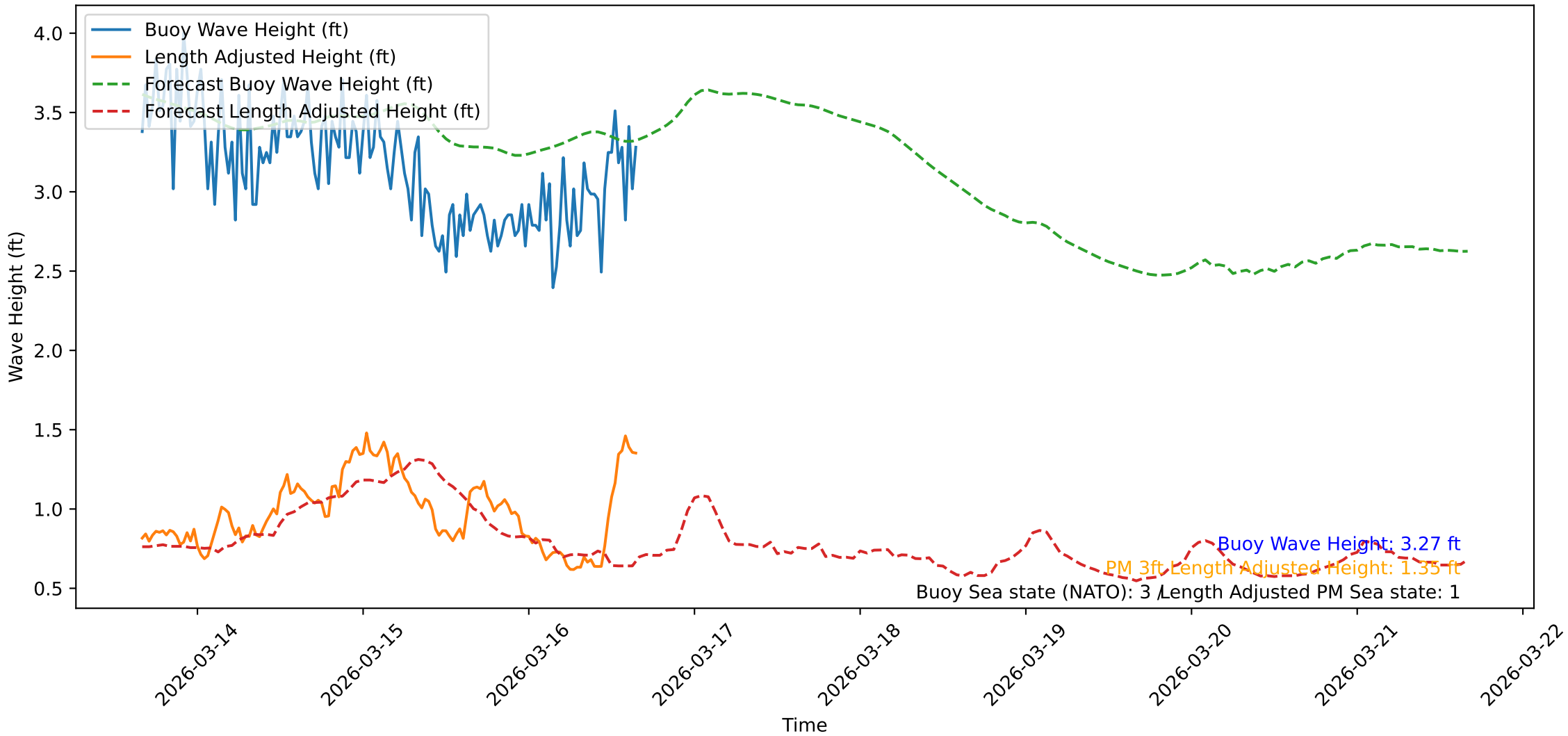
Wave Heights over Time for Oceanside Harbor at 2026-03-16 16:10:42
