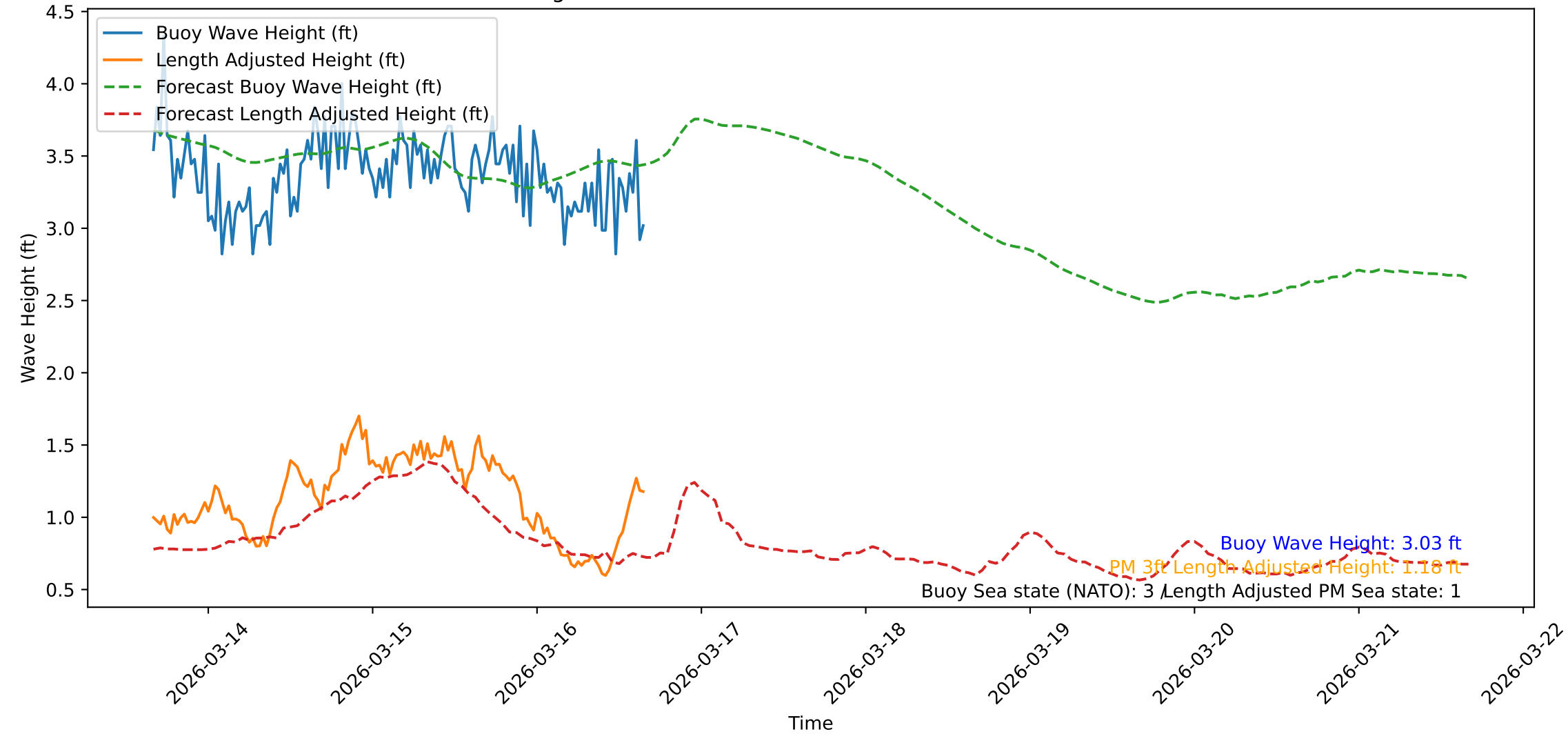
Wave Heights over Time for Green Beach at 2026-03-16 16:11:48
