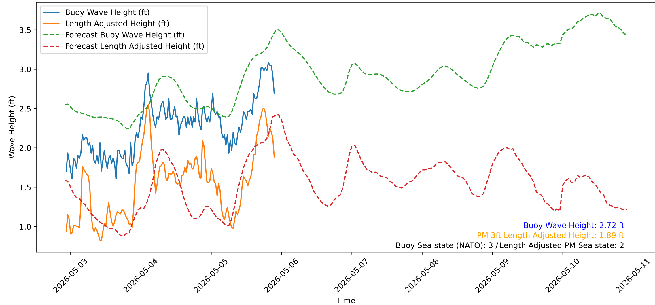
Wave Heights over Time for Red Beach at 2026-05-05 22:10:50
