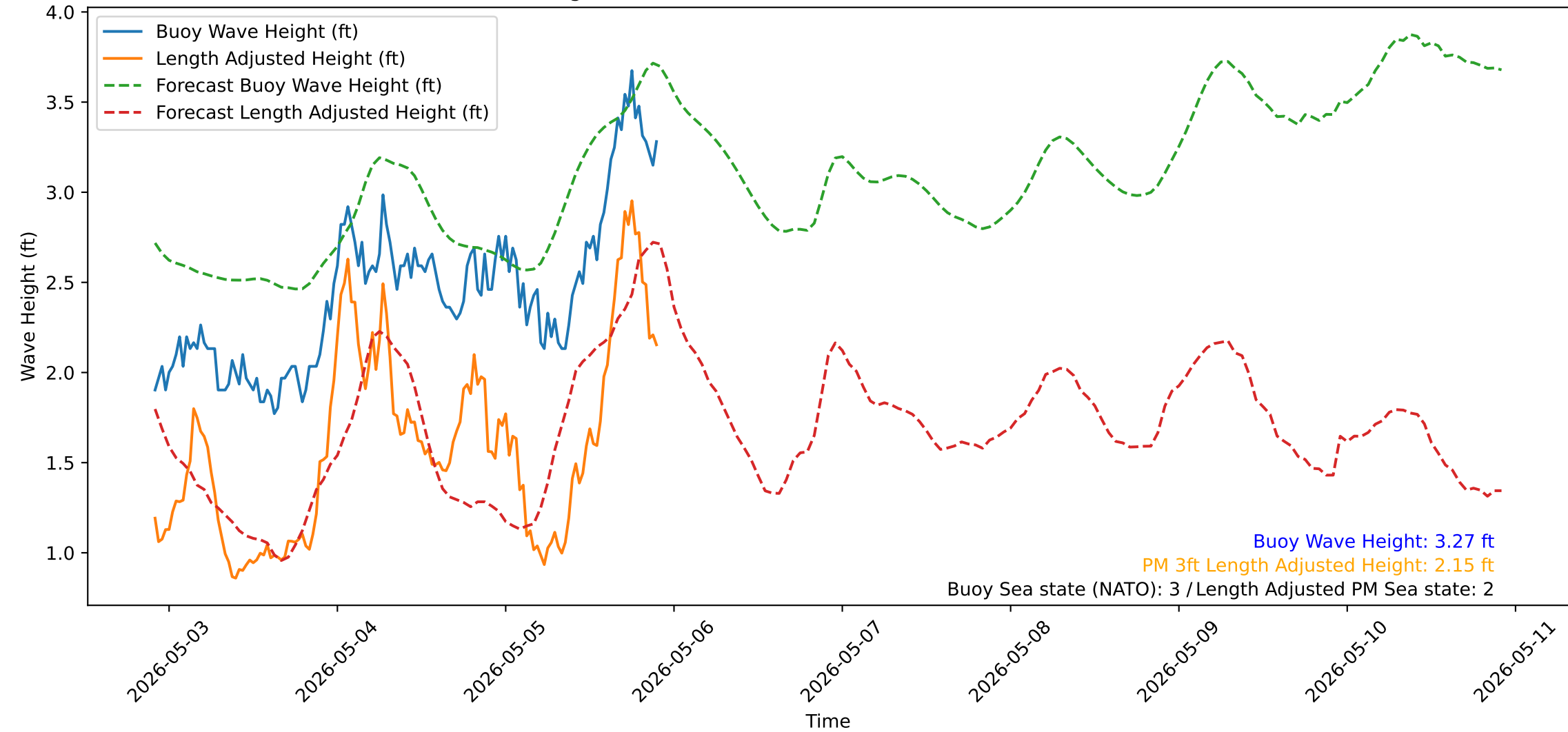
Wave Heights over Time for Green Beach at 2026-05-05 22:11:13
