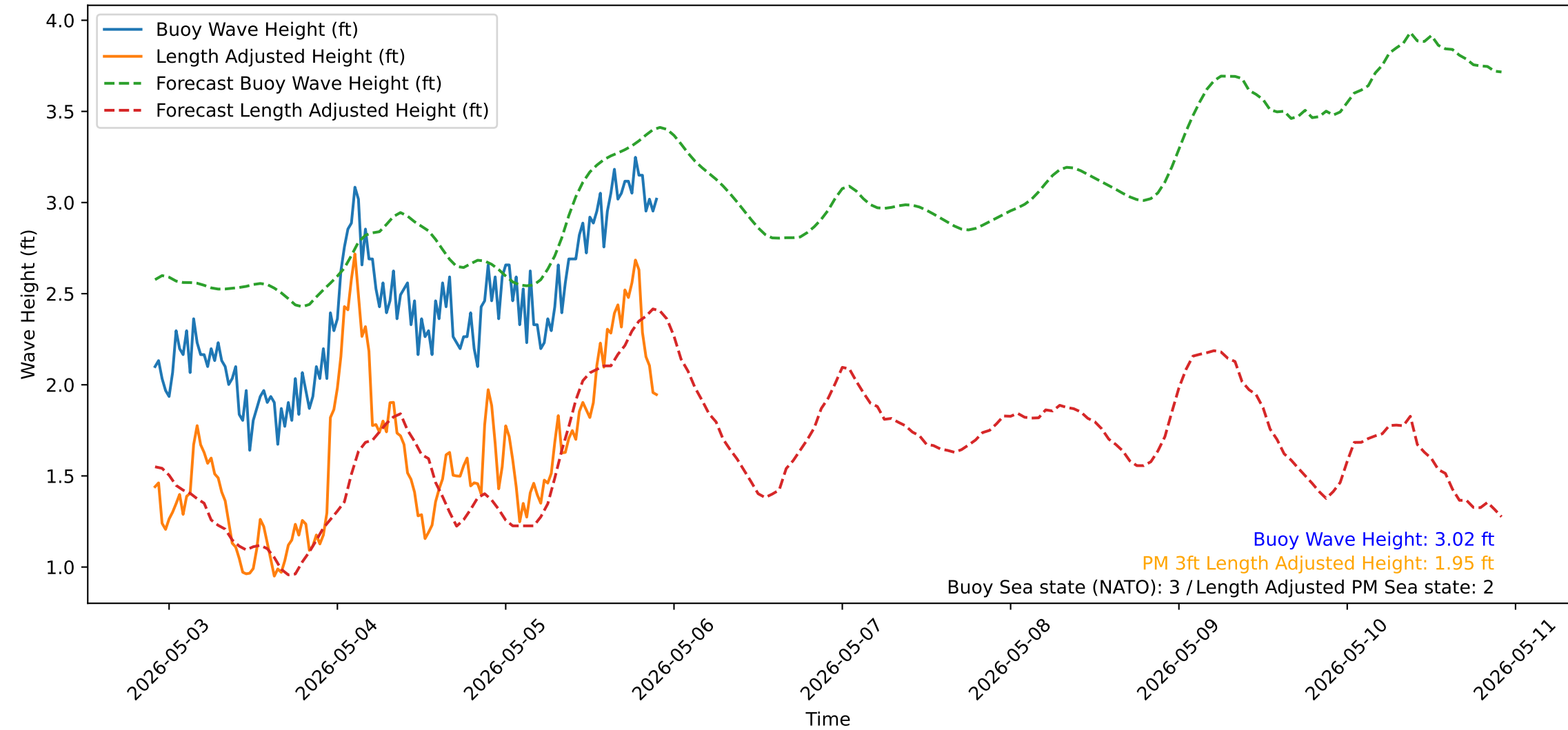
Wave Heights over Time for Oceanside Harbor at 2026-05-05 22:10:31
