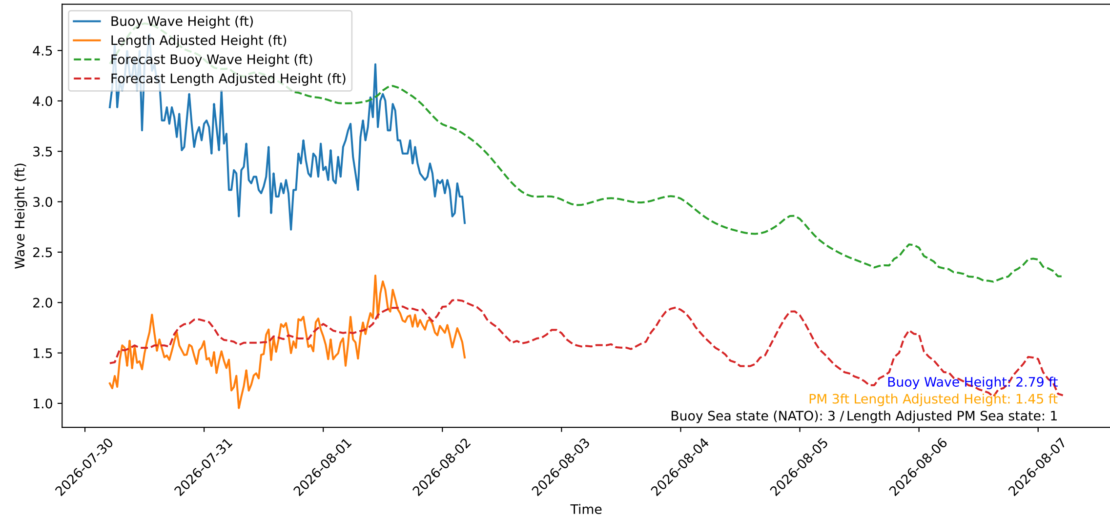
Wave Heights over Time for Oceanside Harbor at 2026-08-02 05:10:26
