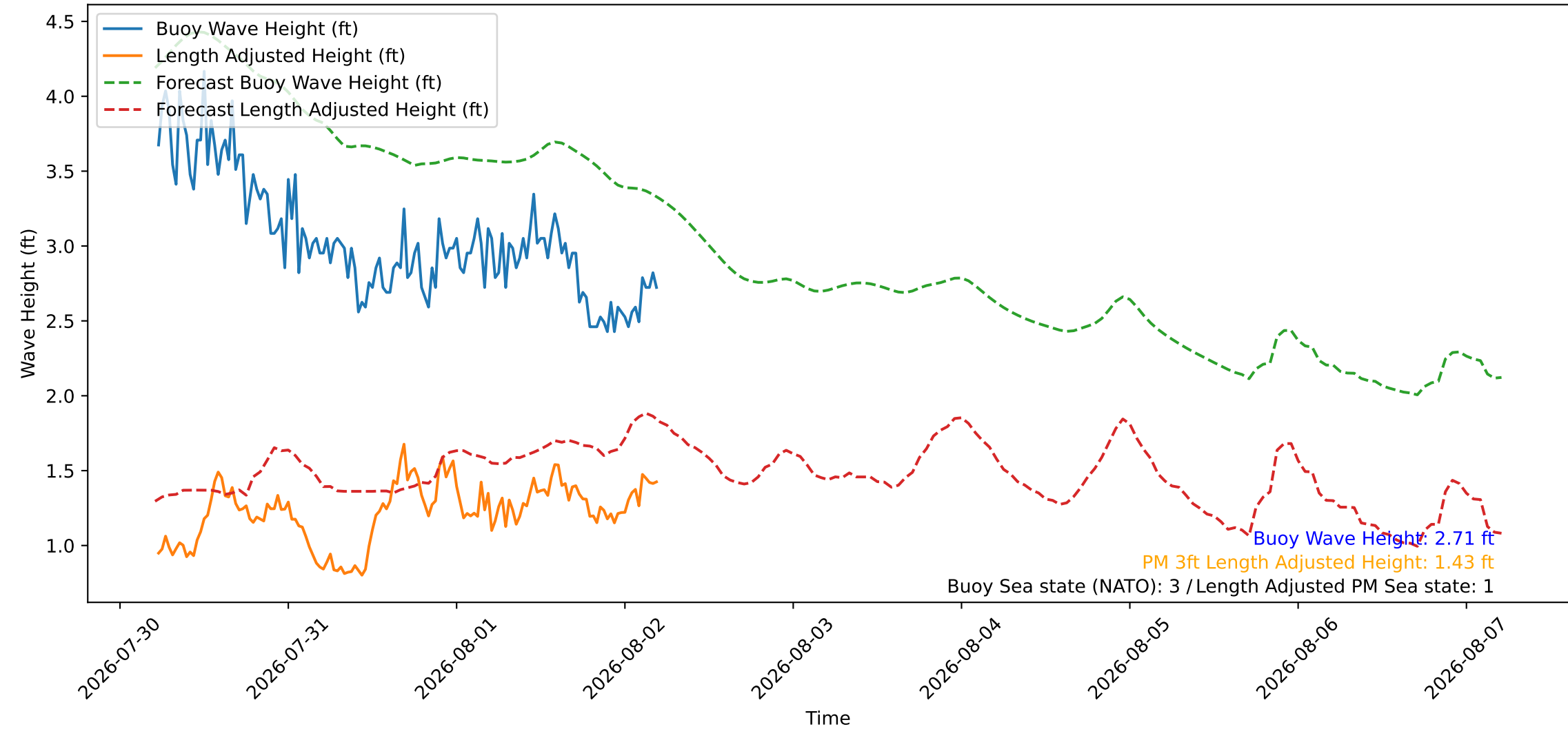
Wave Heights over Time for Red Beach at 2026-08-02 05:10:46
