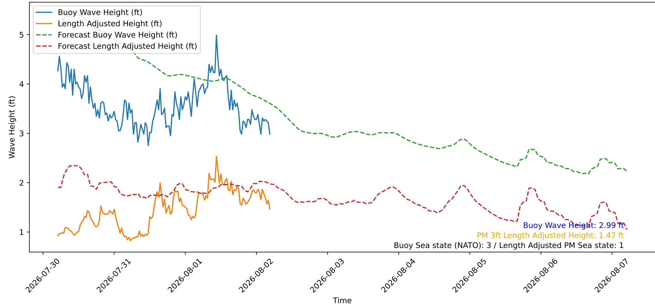
Wave Heights over Time for Green Beach at 2026-08-02 05:11:08
