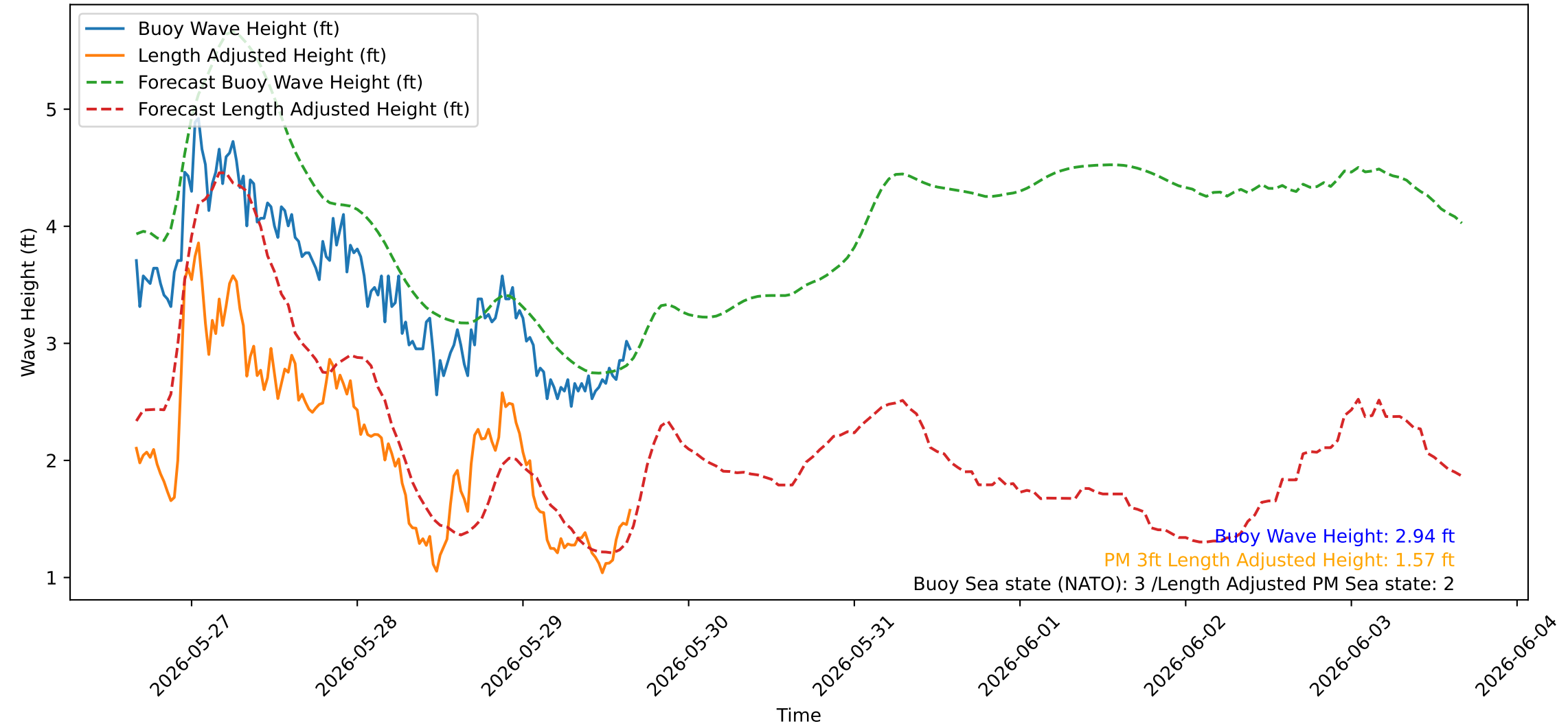
Wave Heights over Time for Green Beach at 2026-05-29 16:11:03
