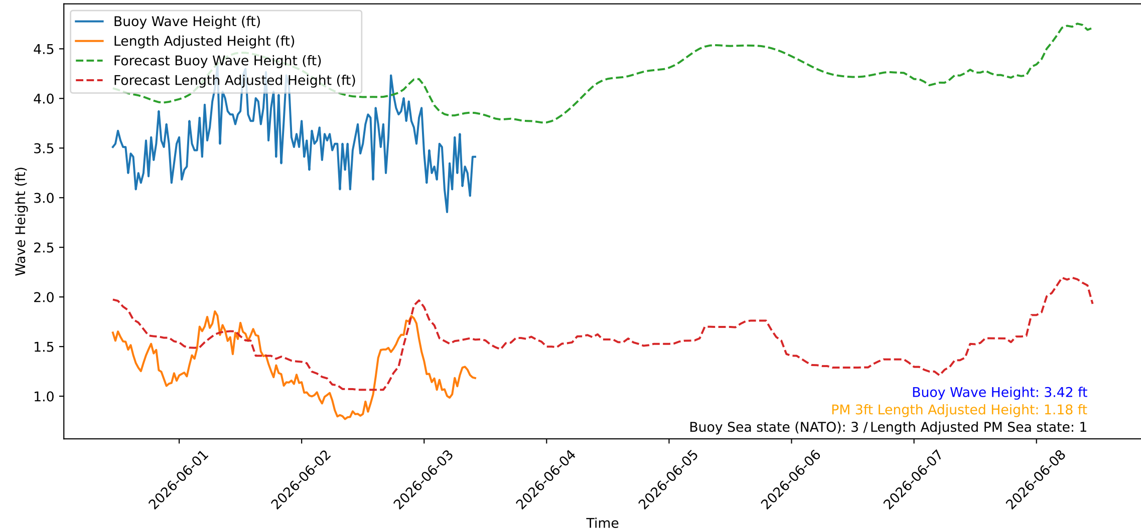
Wave Heights over Time for Green Beach at 2026-06-03 11:01:07
