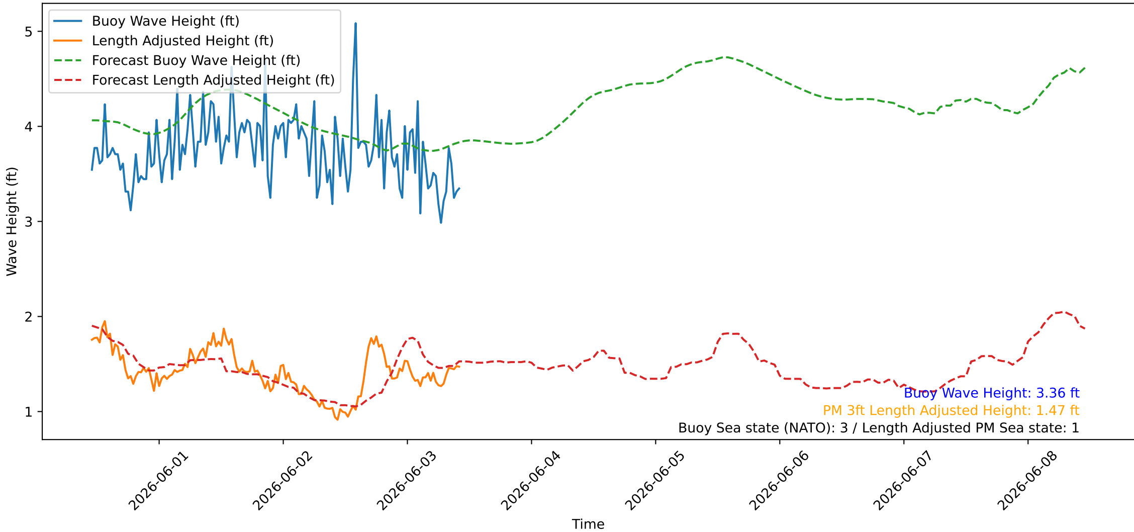
Wave Heights over Time for Oceanside Harbor at 2026-06-03 11:00:25
