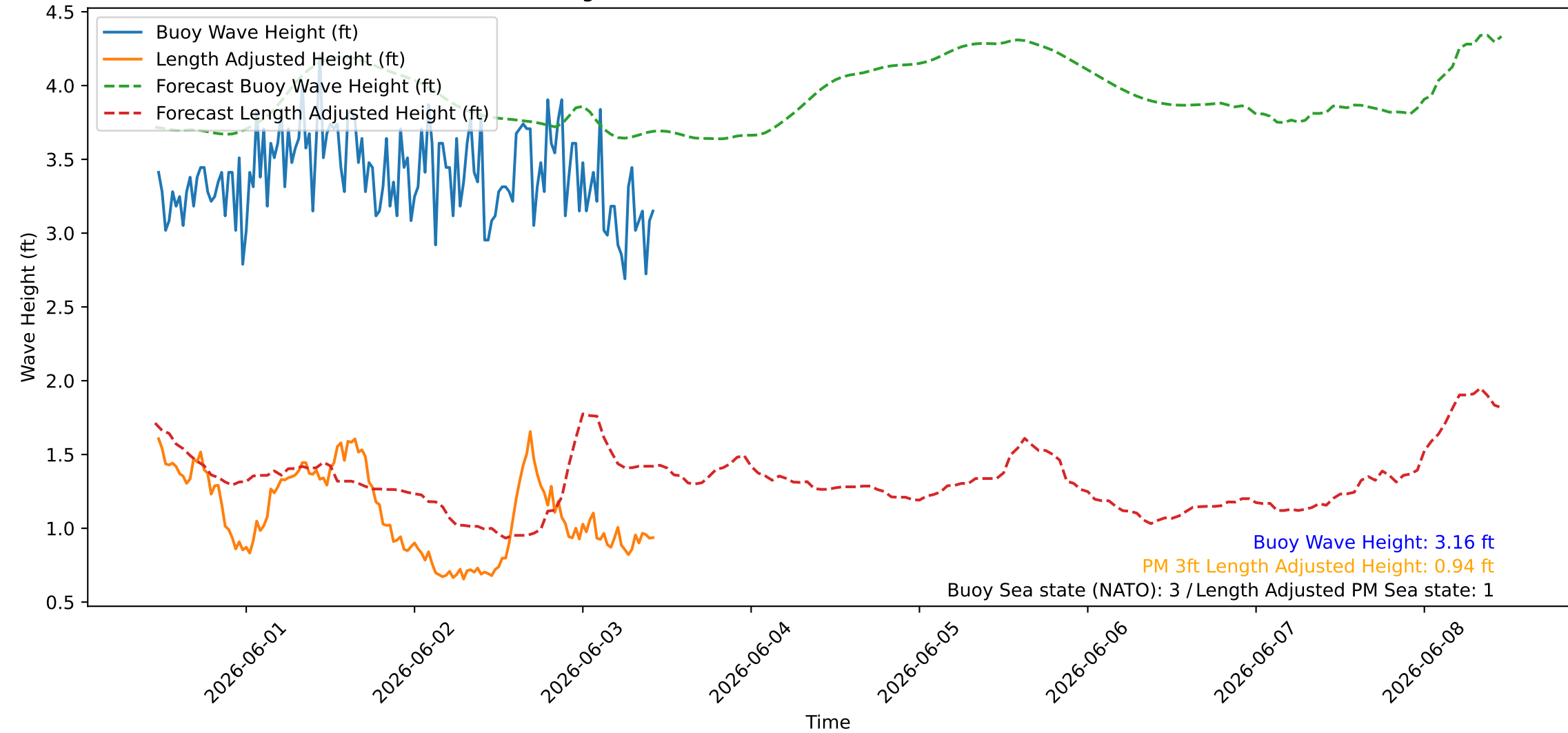
Wave Heights over Time for Red Beach at 2026-06-03 11:00:44
