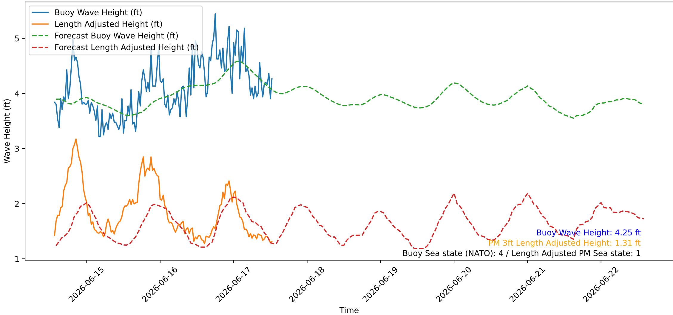
Wave Heights over Time for Oceanside Harbor at 2026-06-17 13:30:26
