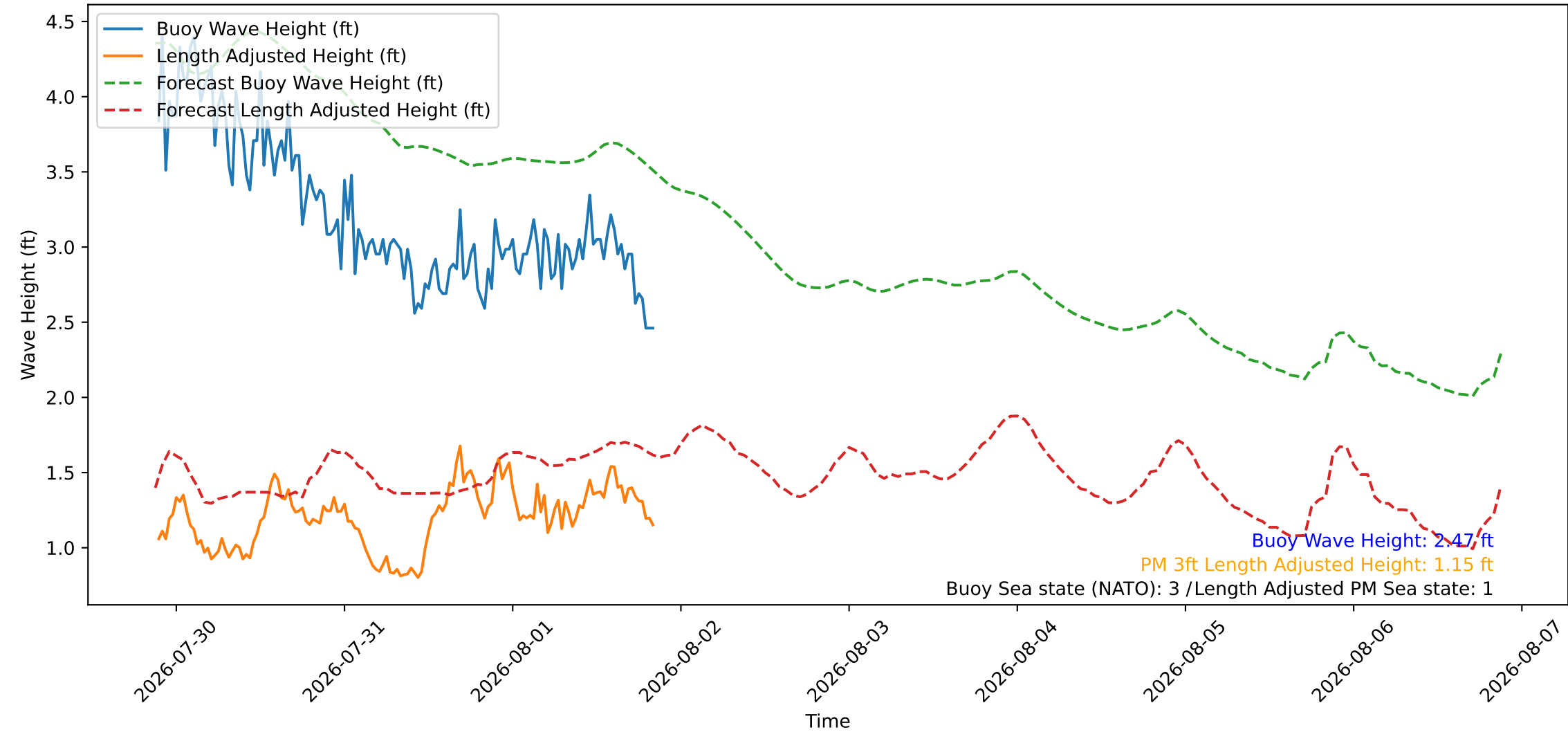
Wave Heights over Time for Red Beach at 2026-08-01 21:00:45
