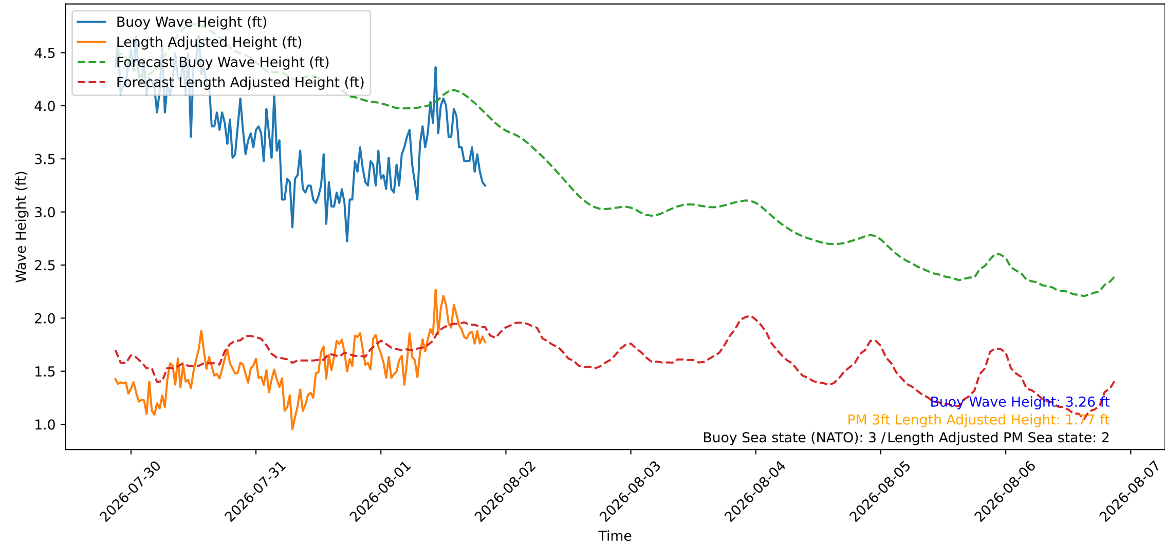
Wave Heights over Time for Oceanside Harbor at 2026-08-01 21:00:25
