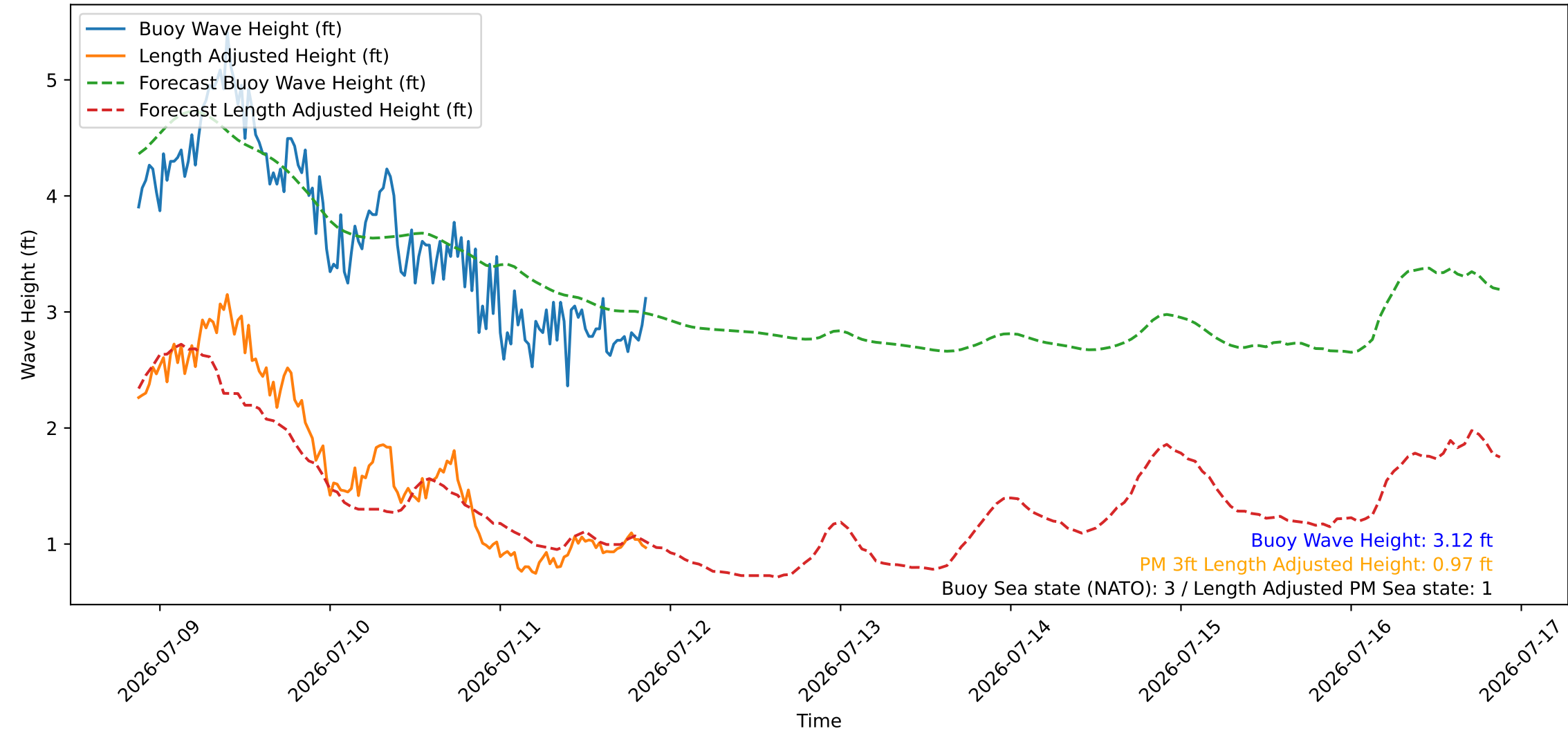
Wave Heights over Time for Oceanside Harbor at 2026-07-11 21:10:26
