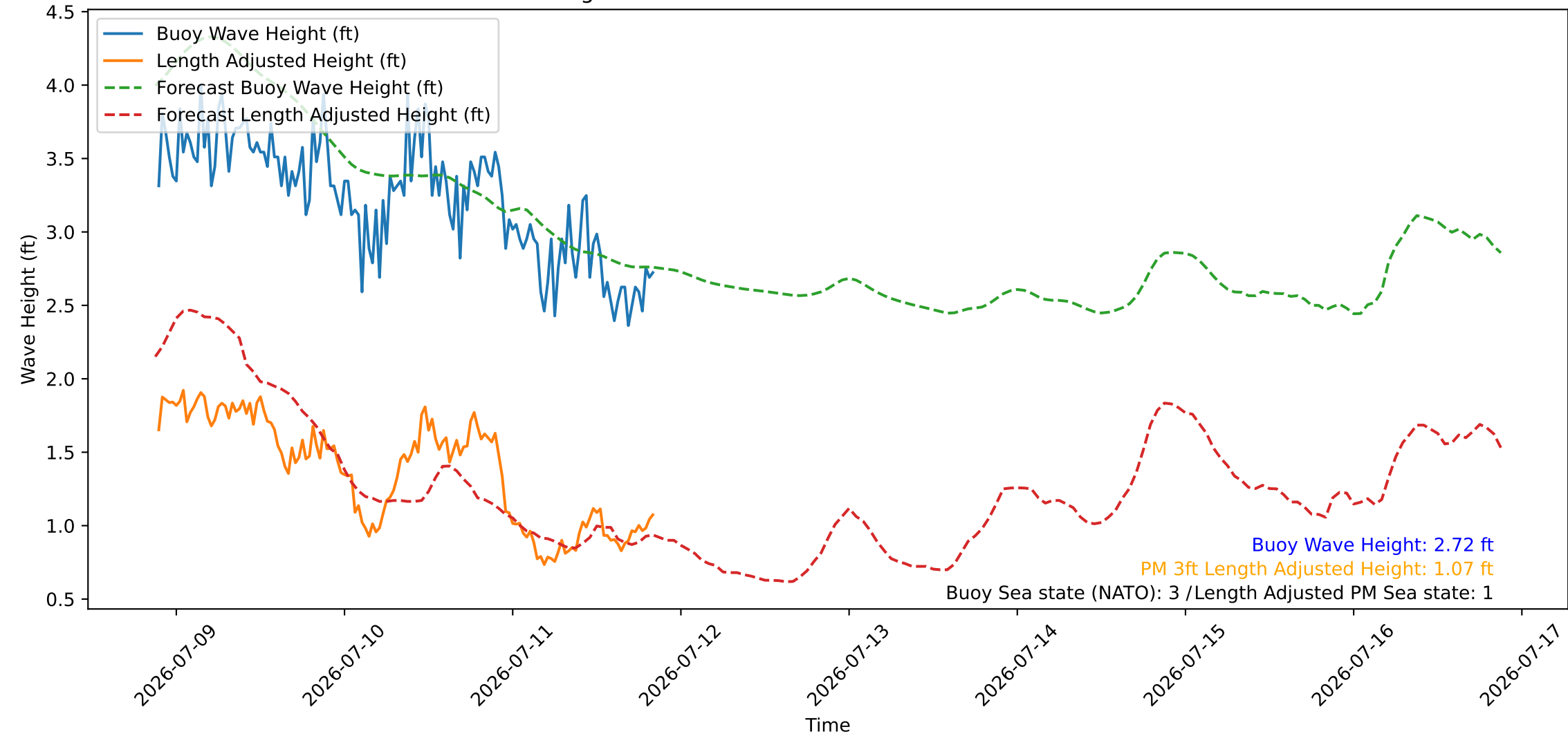
Wave Heights over Time for Red Beach at 2026-07-11 21:10:45
