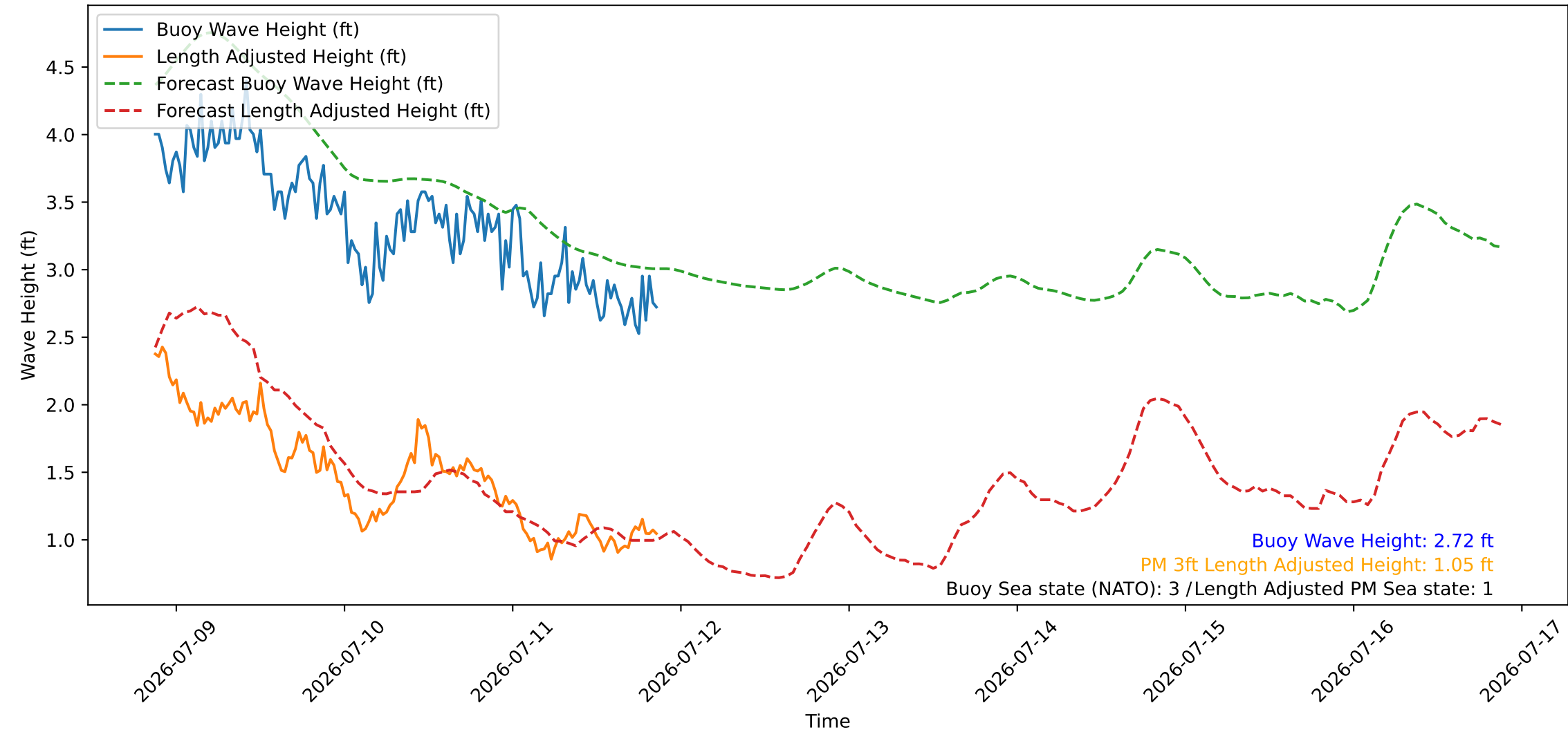
Wave Heights over Time for Green Beach at 2026-07-11 21:11:07
