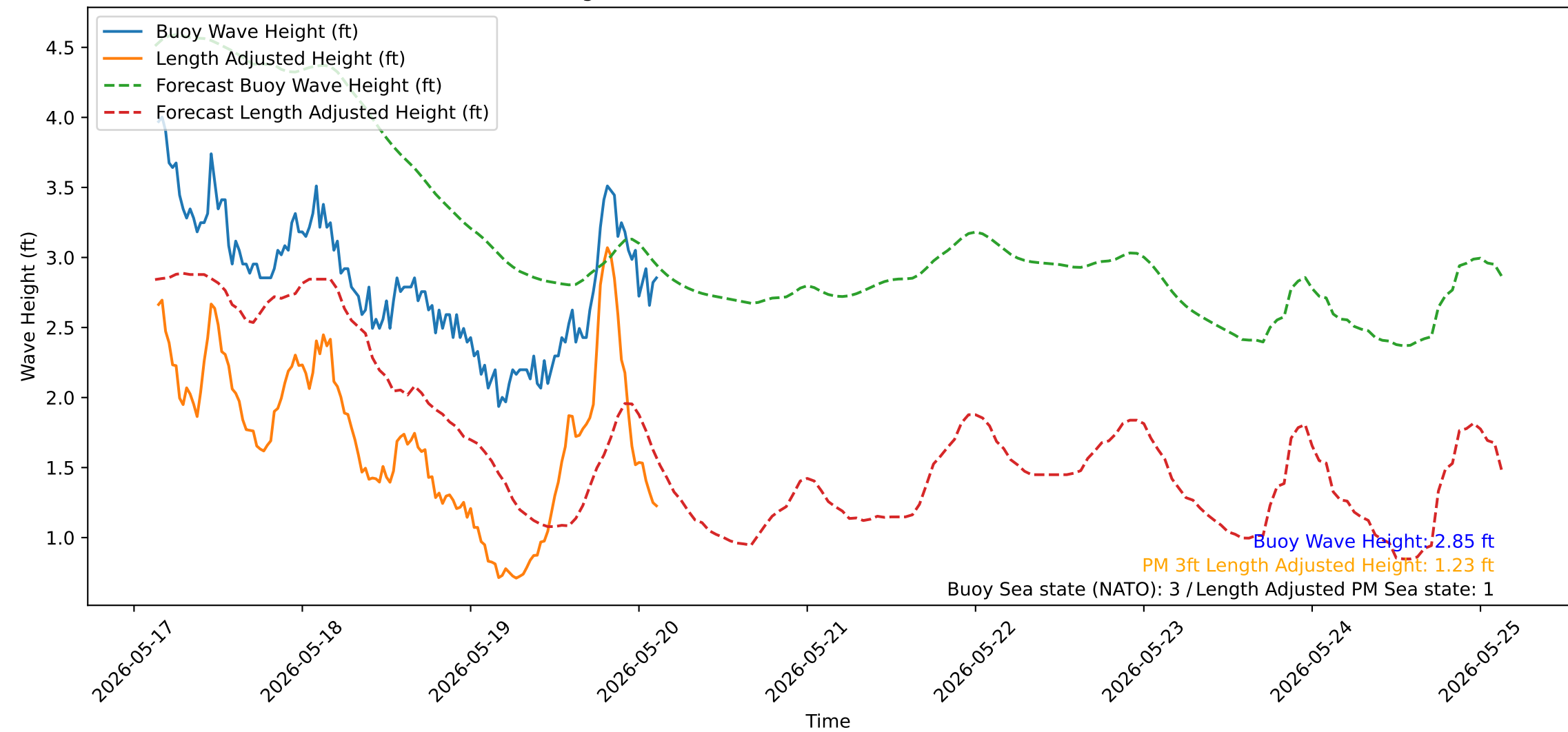
Wave Heights over Time for Red Beach at 2026-05-20 03:20:51
