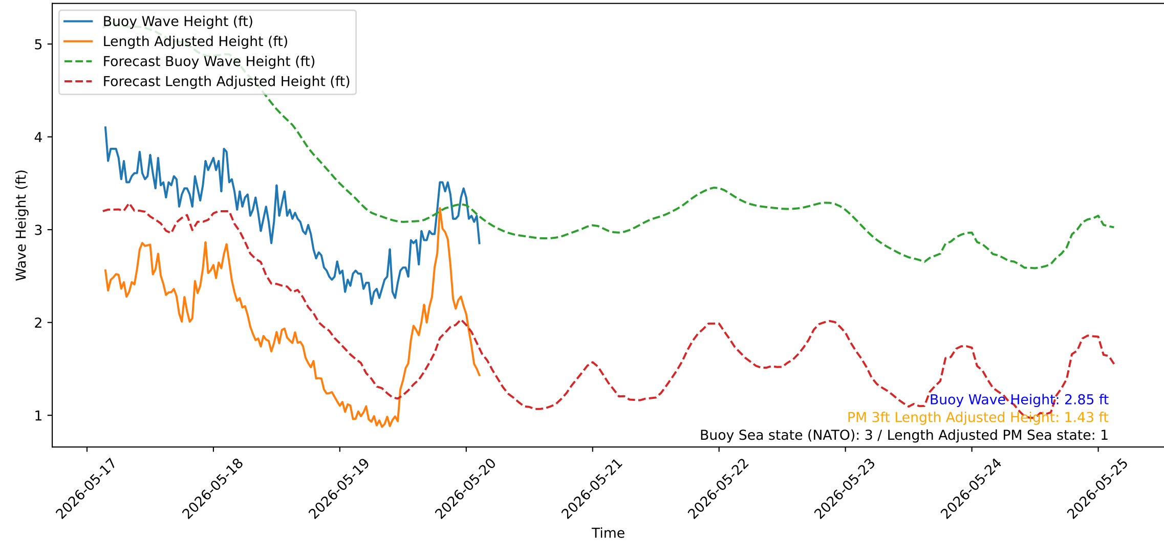
Wave Heights over Time for Oceanside Harbor at 2026-05-20 03:20:30
