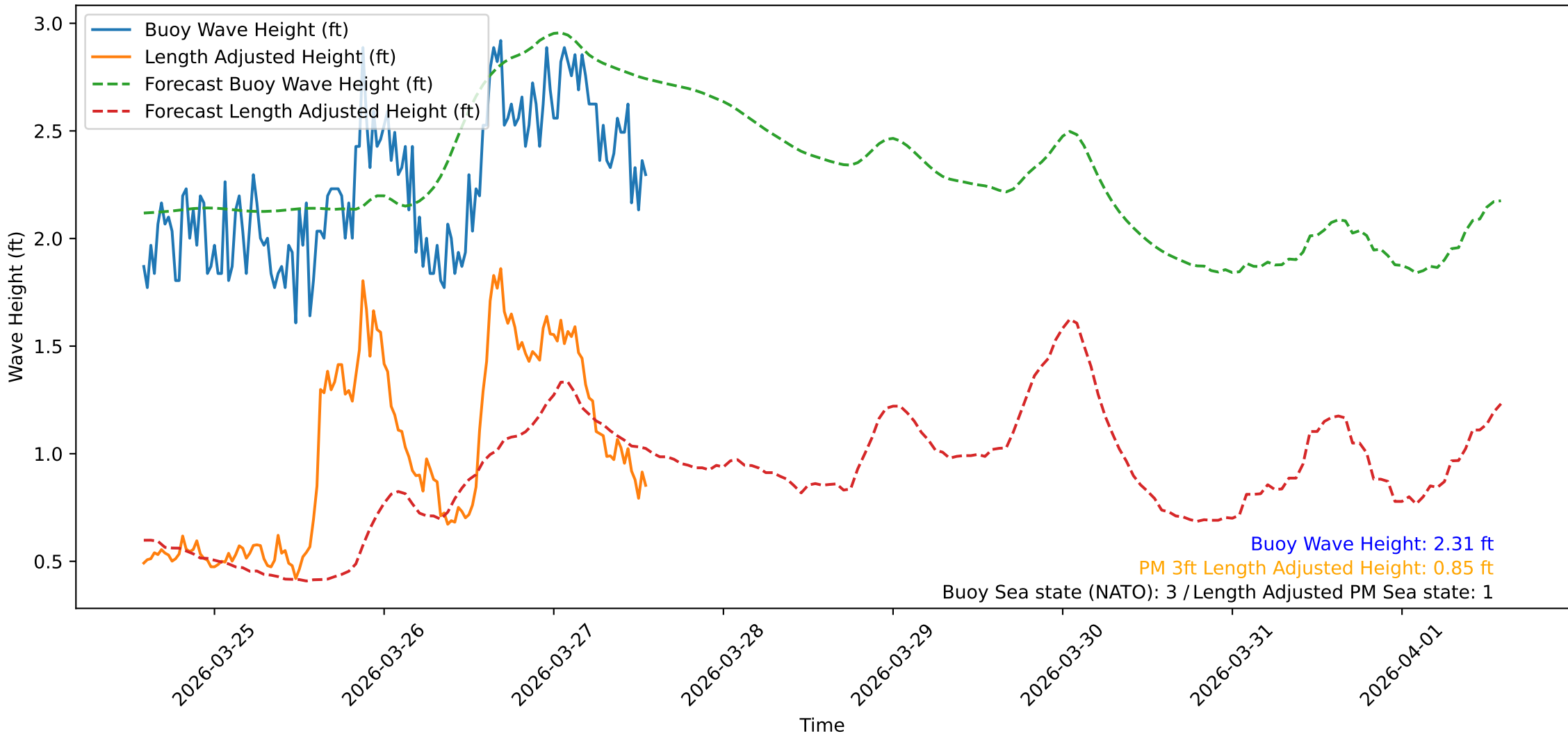
Wave Heights over Time for Oceanside Harbor at 2026-03-27 13:50:31
