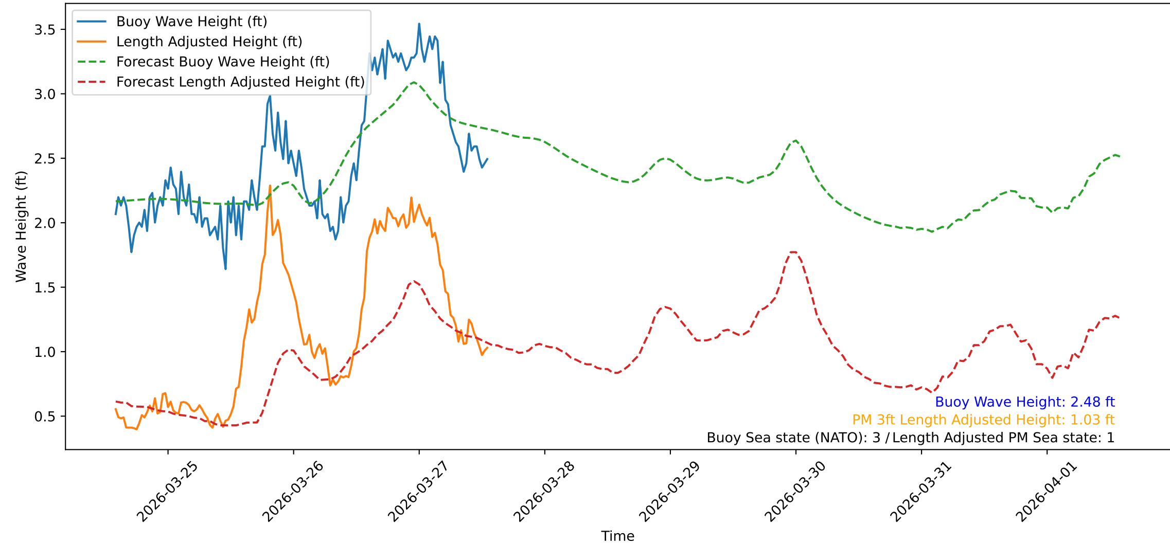
Wave Heights over Time for Green Beach at 2026-03-27 13:51:09
