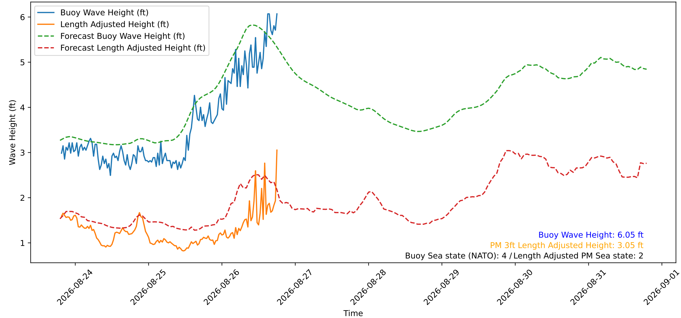
Wave Heights over Time for Green Beach at 2026-08-26 19:01:12
