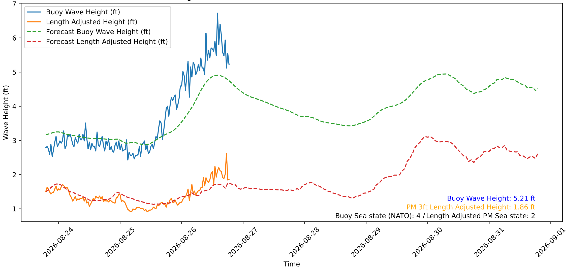
Wave Heights over Time for Oceanside Harbor at 2026-08-26 19:00:30
