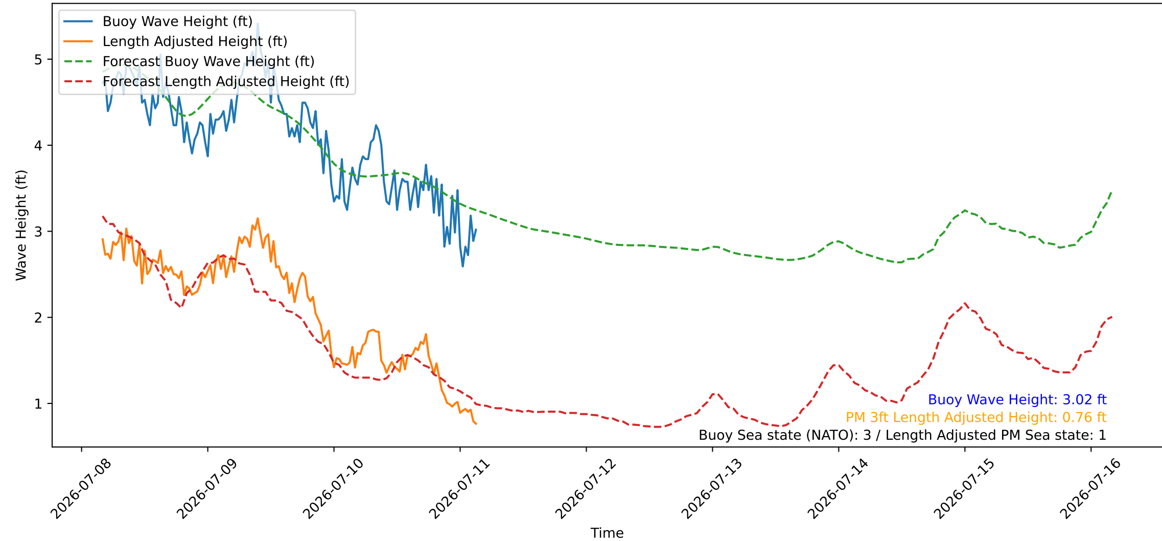
Wave Heights over Time for Oceanside Harbor at 2026-07-11 04:00:26
