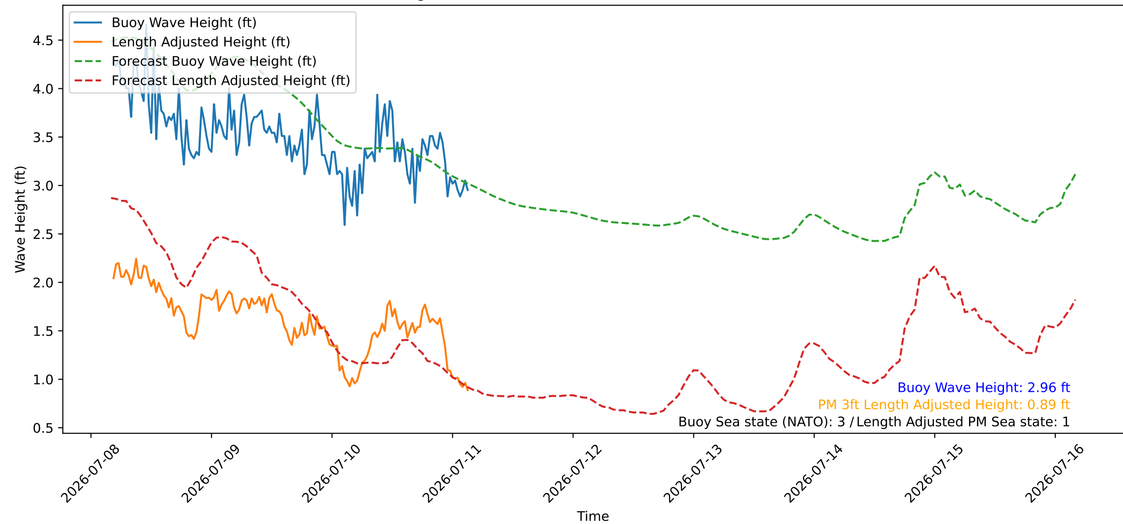
Wave Heights over Time for Red Beach at 2026-07-11 04:00:45
