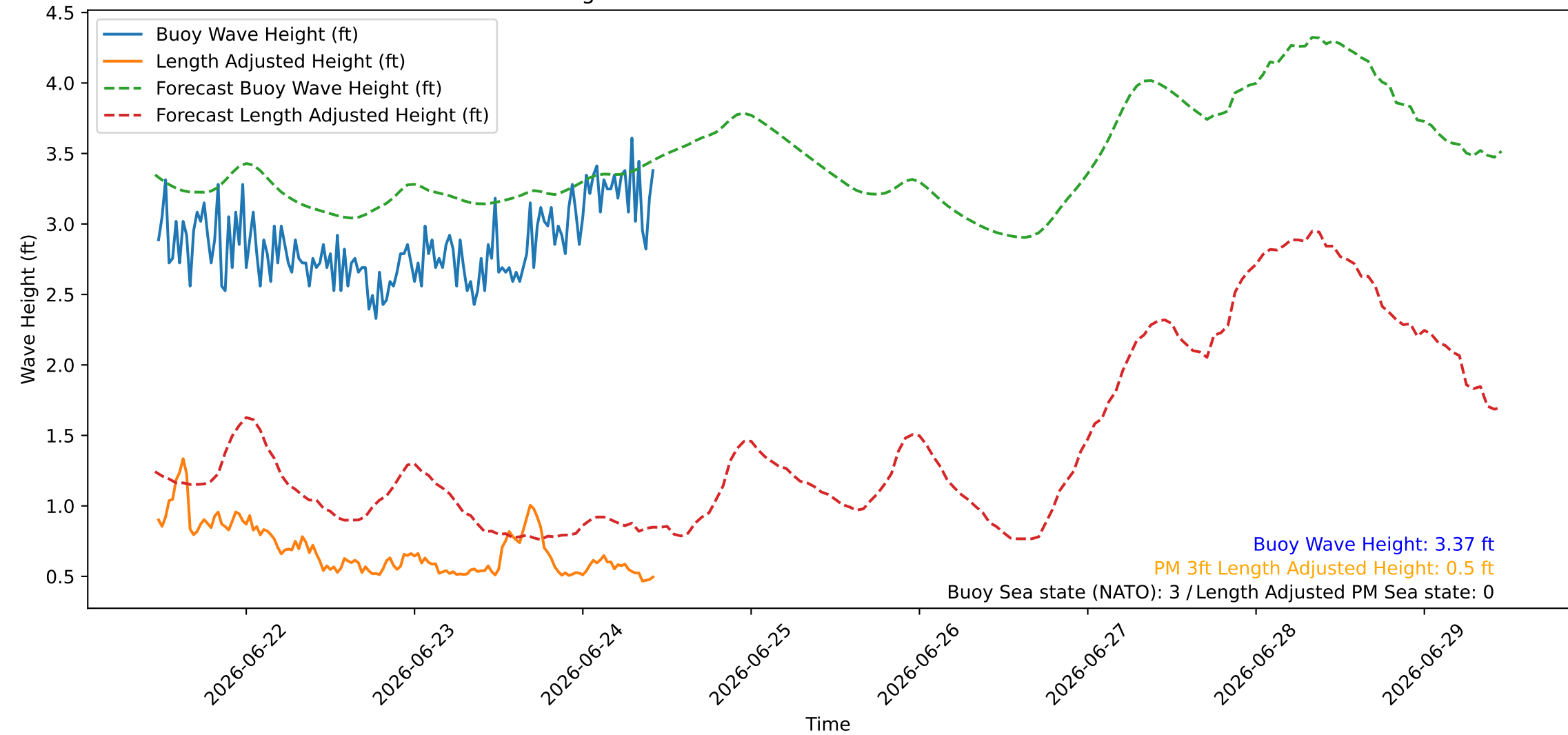
Wave Heights over Time for Red Beach at 2026-06-24 11:10:45
