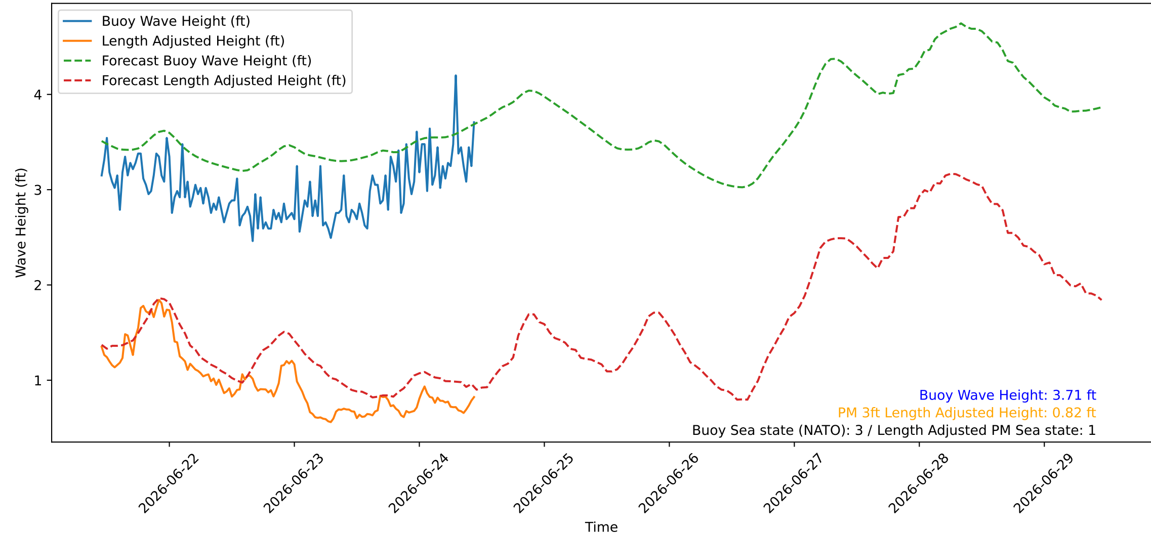
Wave Heights over Time for Green Beach at 2026-06-24 11:11:07
