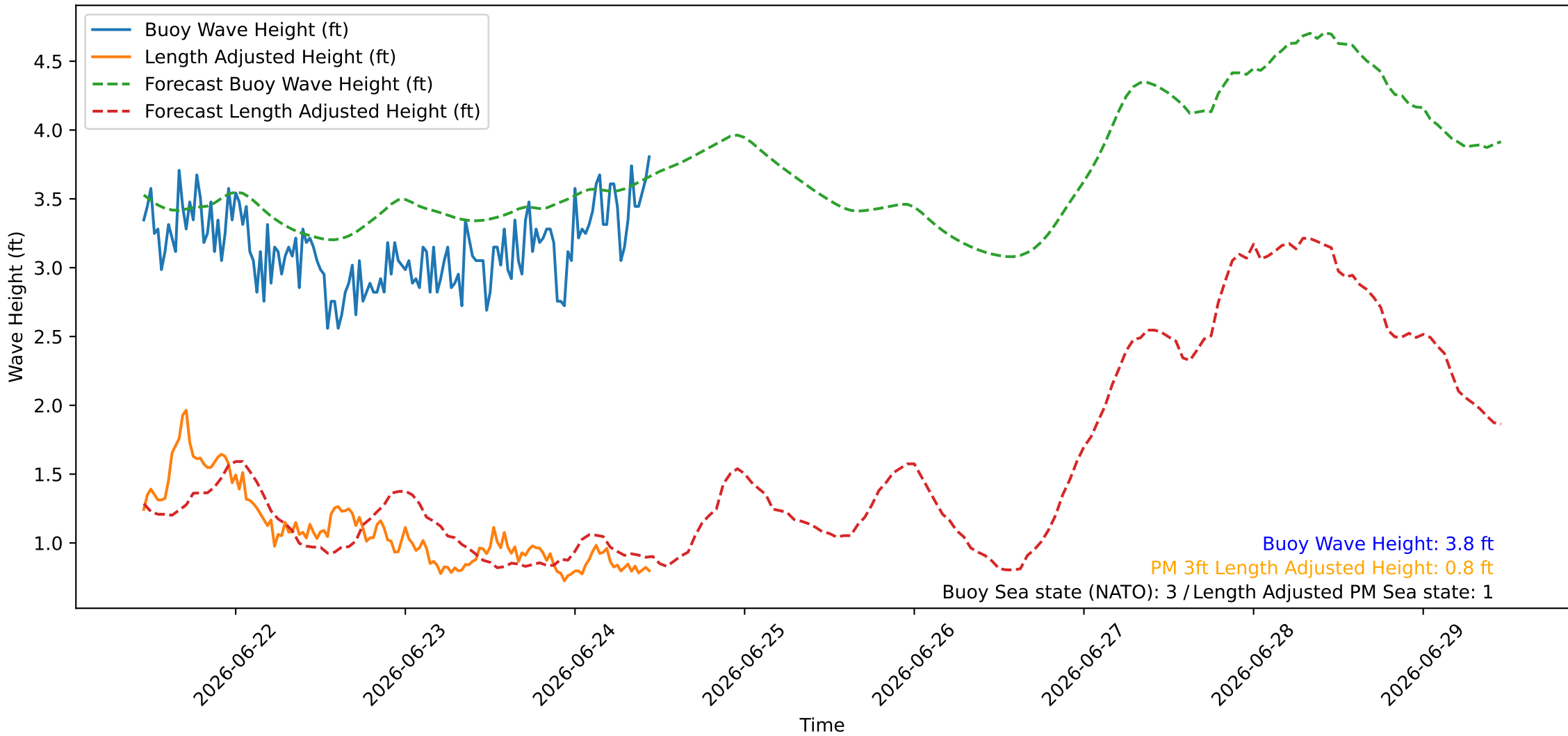
Wave Heights over Time for Oceanside Harbor at 2026-06-24 11:10:26
