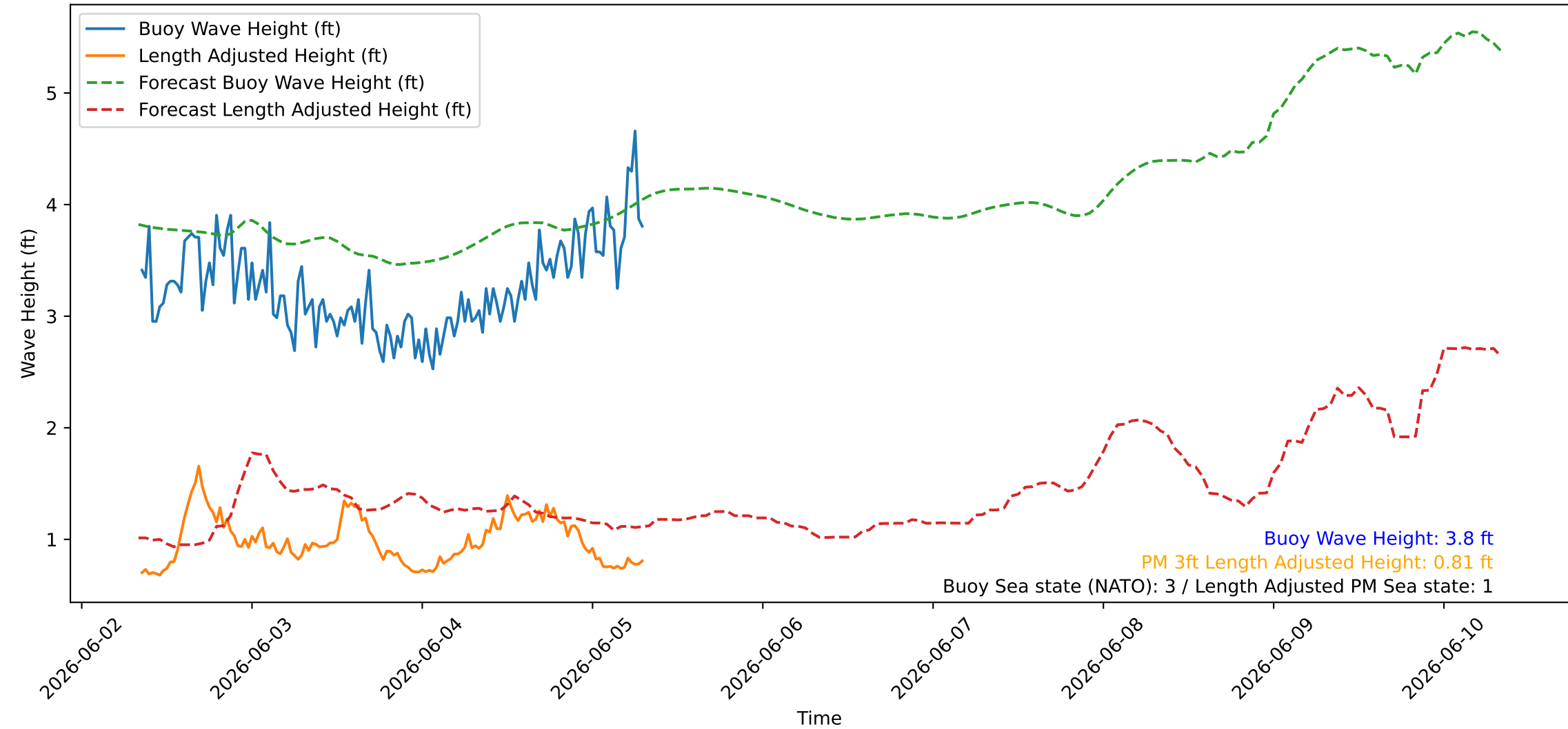
Wave Heights over Time for Red Beach at 2026-06-05 08:00:45
