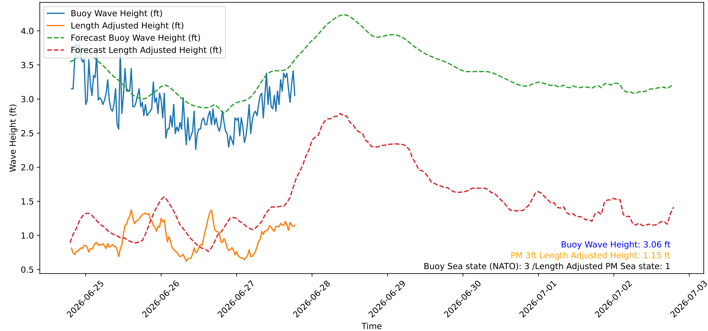
Wave Heights over Time for Red Beach at 2026-06-27 19:10:46
