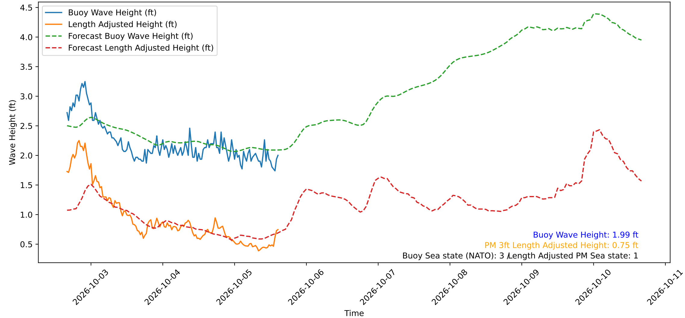
Wave Heights over Time for Red Beach at 2026-10-05 15:30:49
