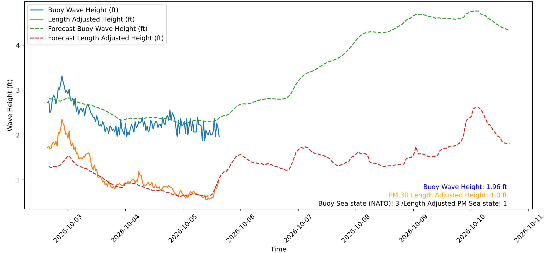
Wave Heights over Time for Oceanside Harbor at 2026-10-05 15:30:29
