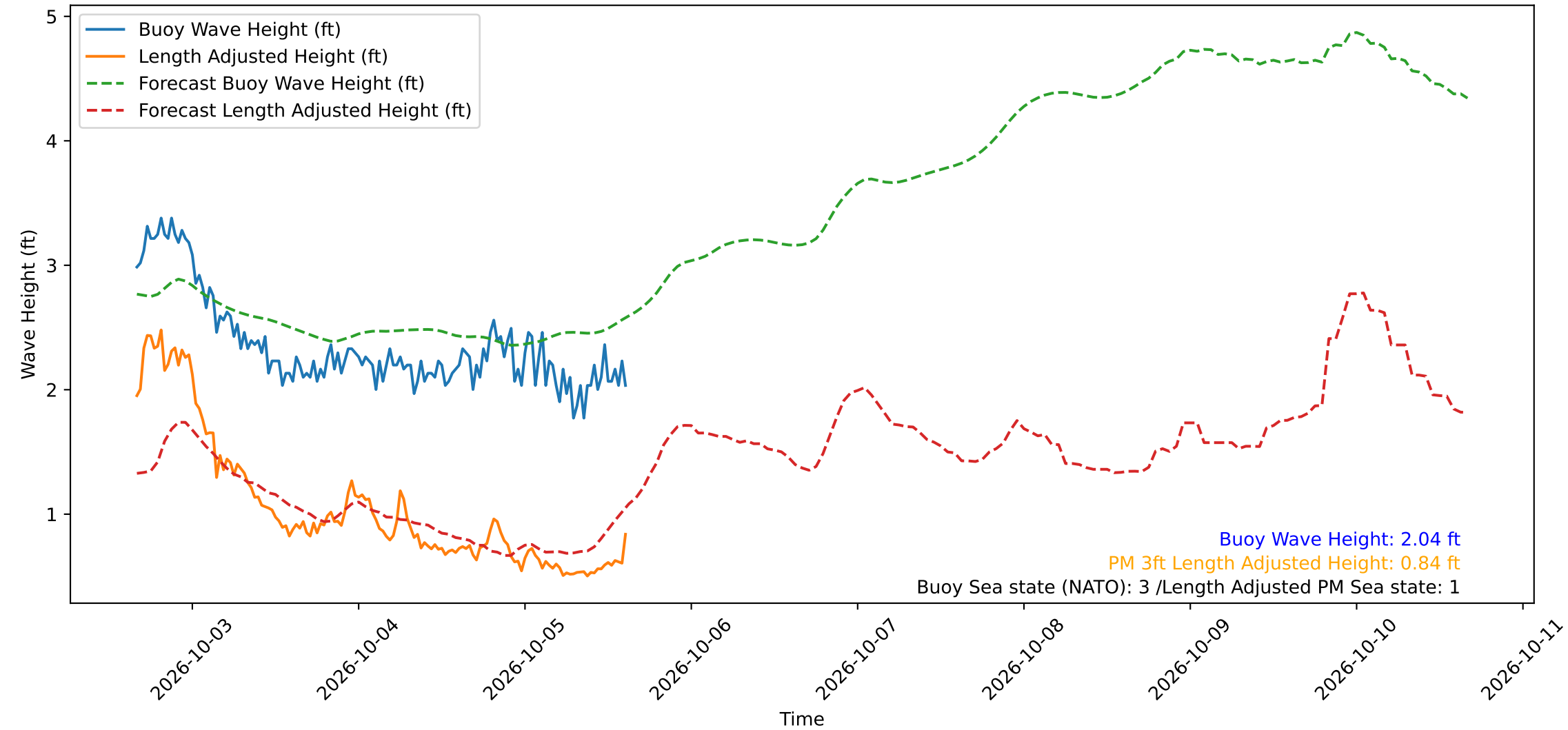
Wave Heights over Time for Green Beach at 2026-10-05 15:31:11
