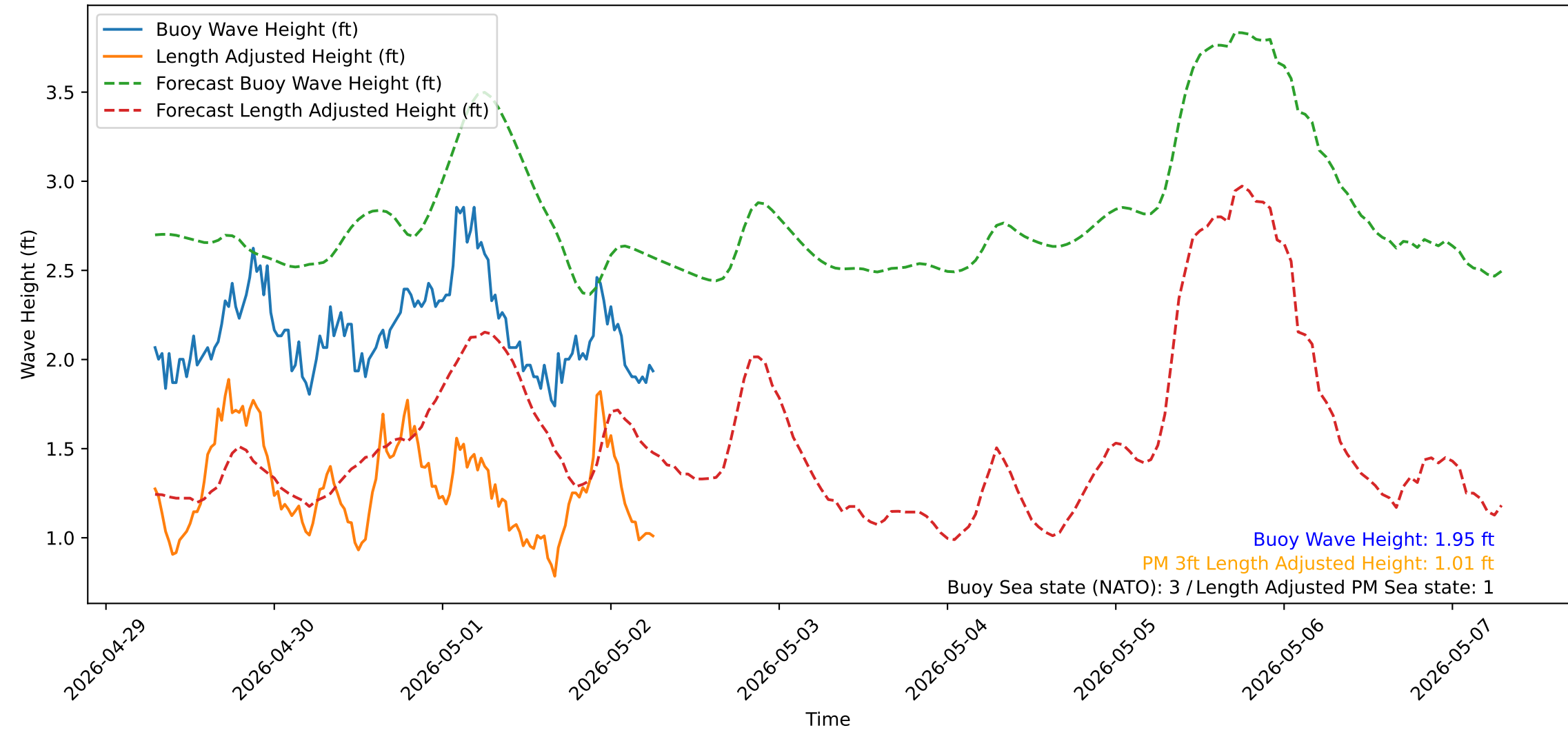
Wave Heights over Time for Green Beach at 2026-05-02 06:51:14
