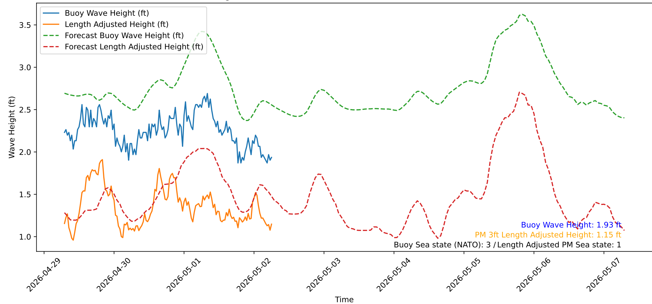
Wave Heights over Time for Oceanside Harbor at 2026-05-02 06:50:31
