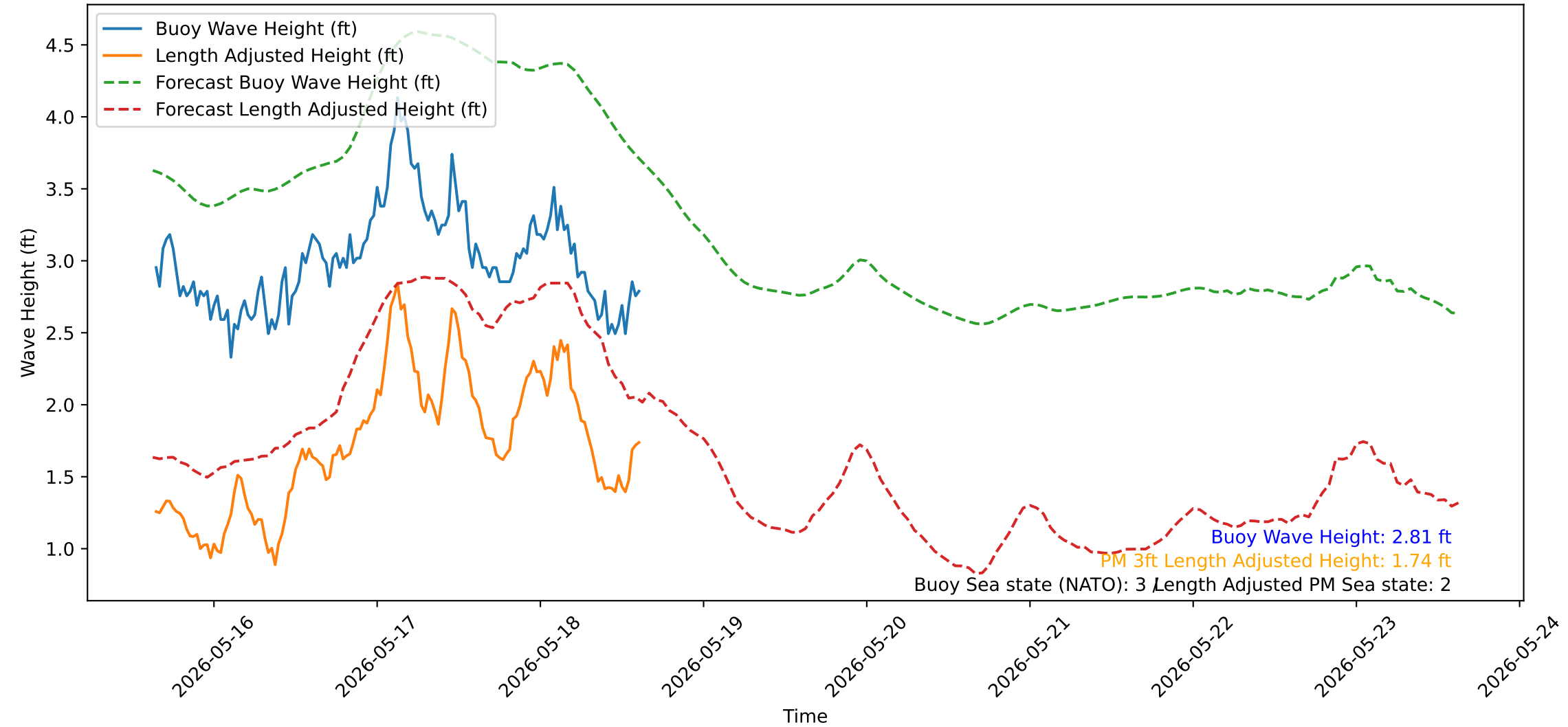
Wave Heights over Time for Red Beach at 2026-05-18 15:20:52
