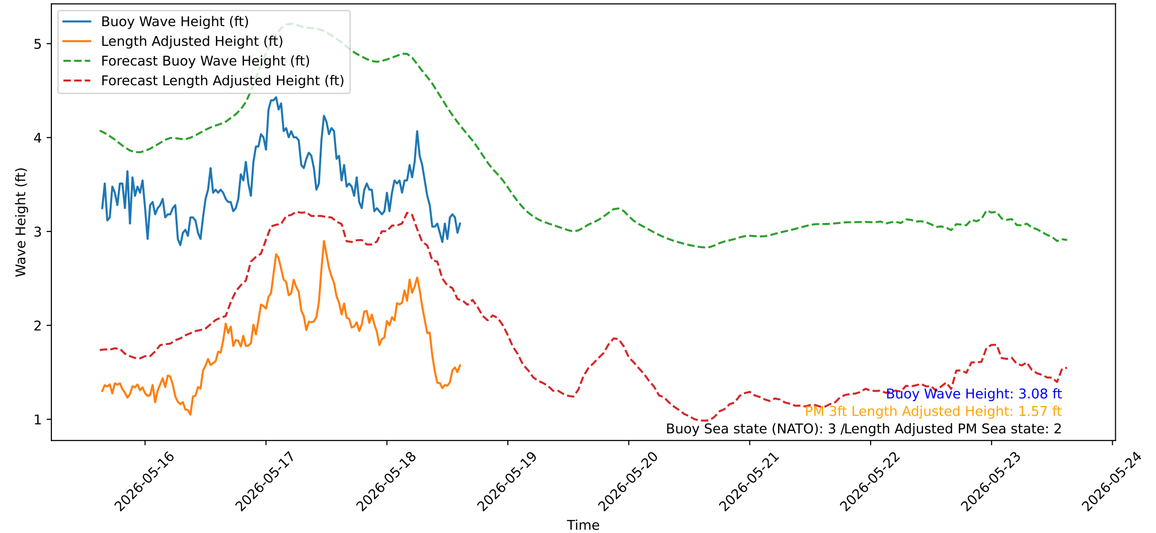
Wave Heights over Time for Green Beach at 2026-05-18 15:21:15
