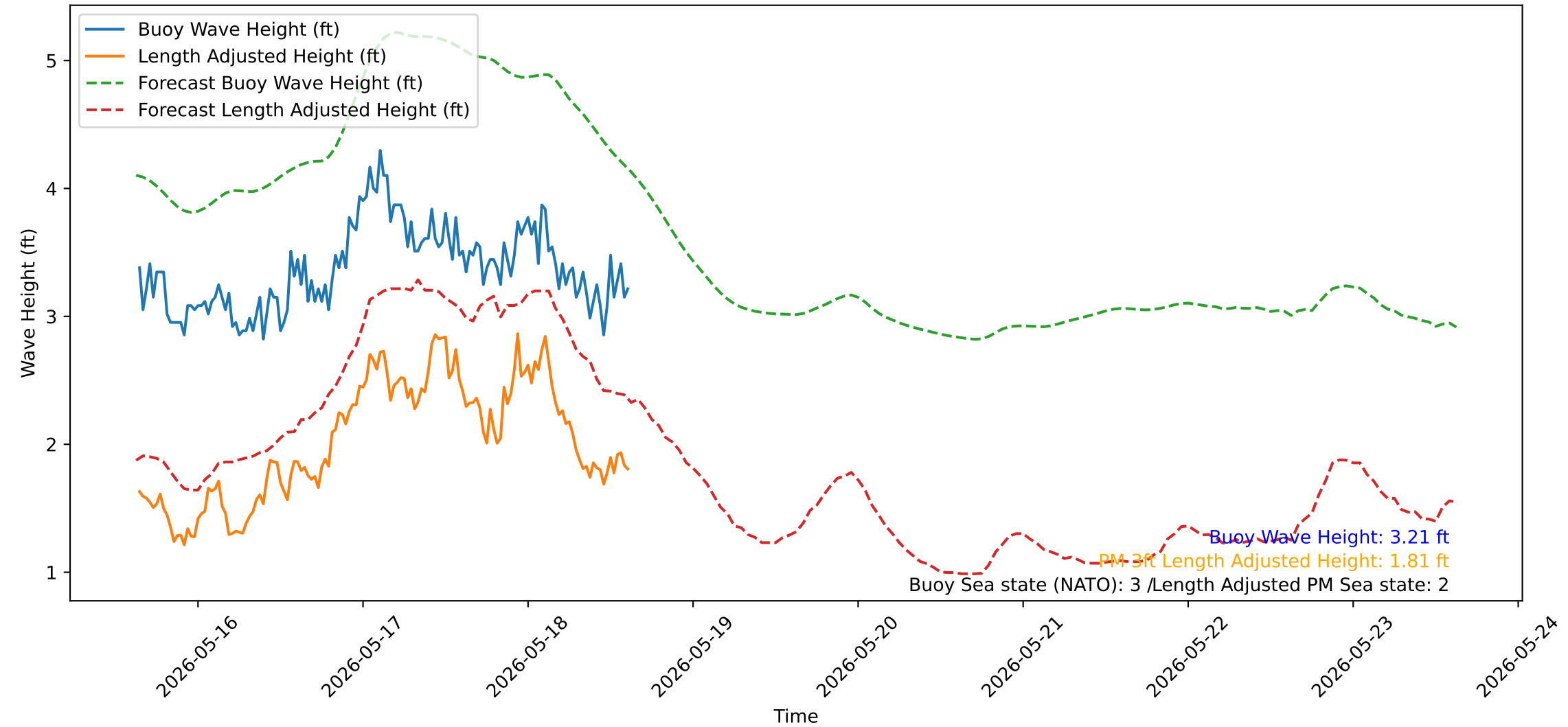
Wave Heights over Time for Oceanside Harbor at 2026-05-18 15:20:32
