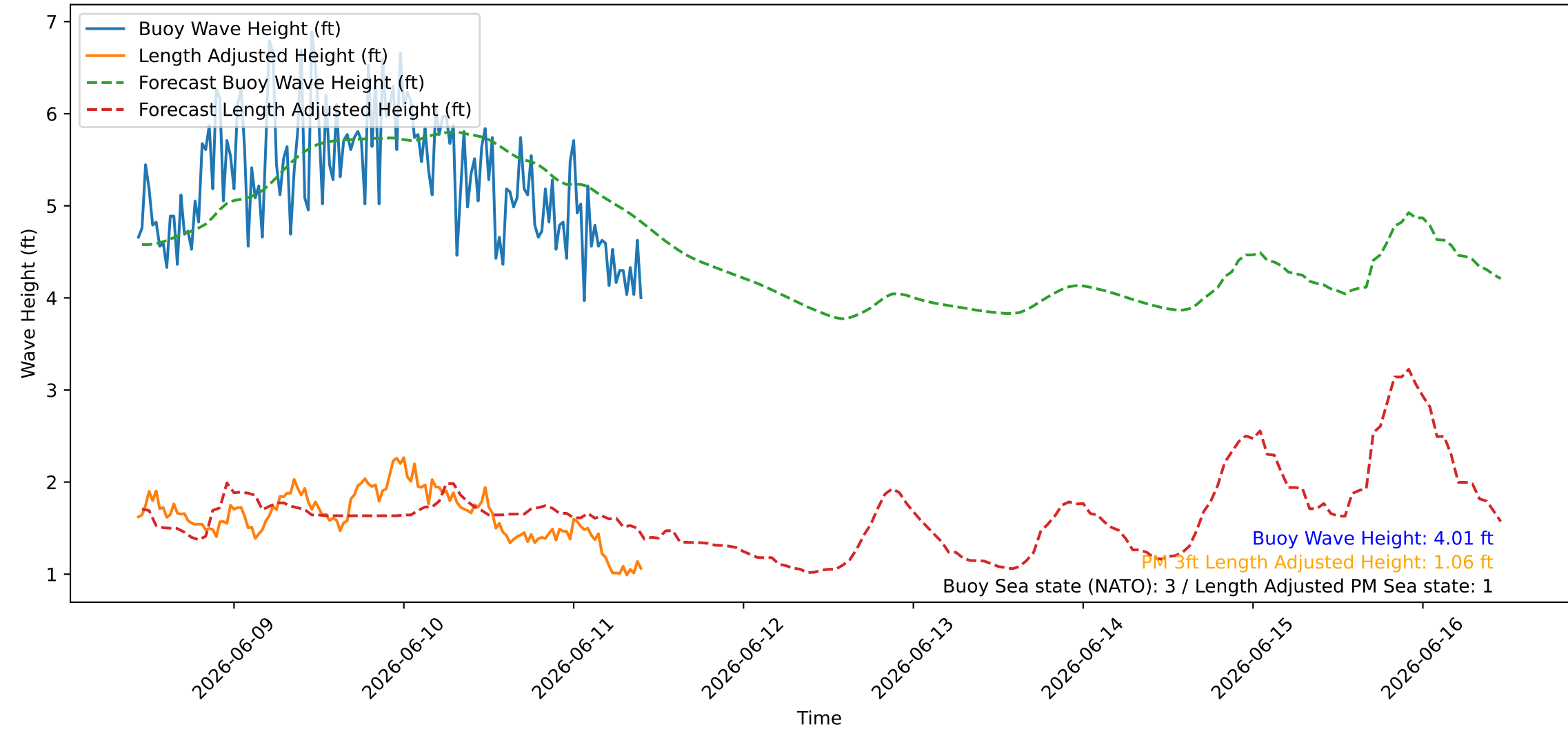
Wave Heights over Time for Green Beach at 2026-06-11 10:31:09
