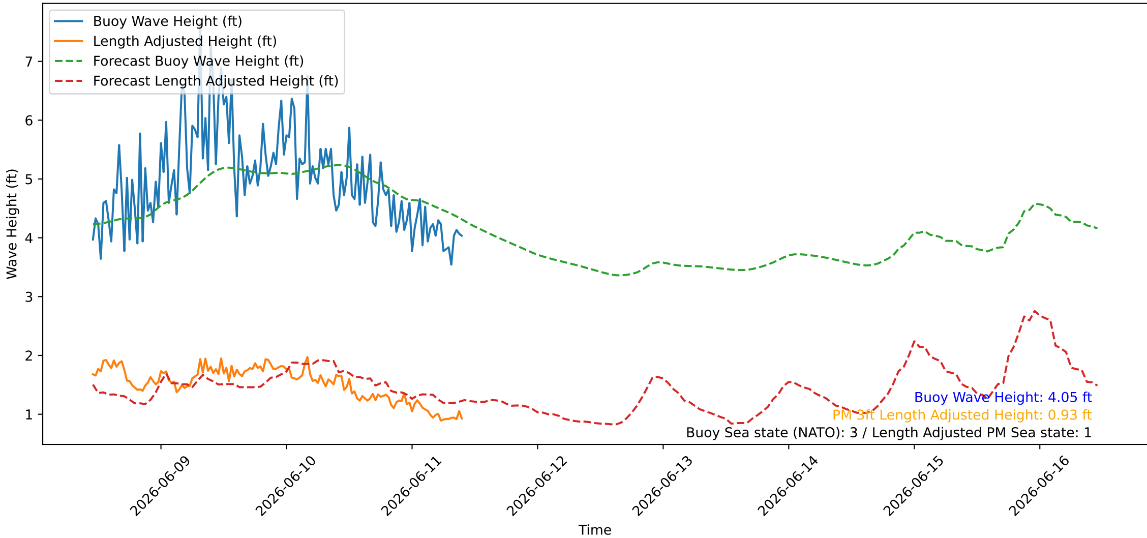
Wave Heights over Time for Red Beach at 2026-06-11 10:30:46
