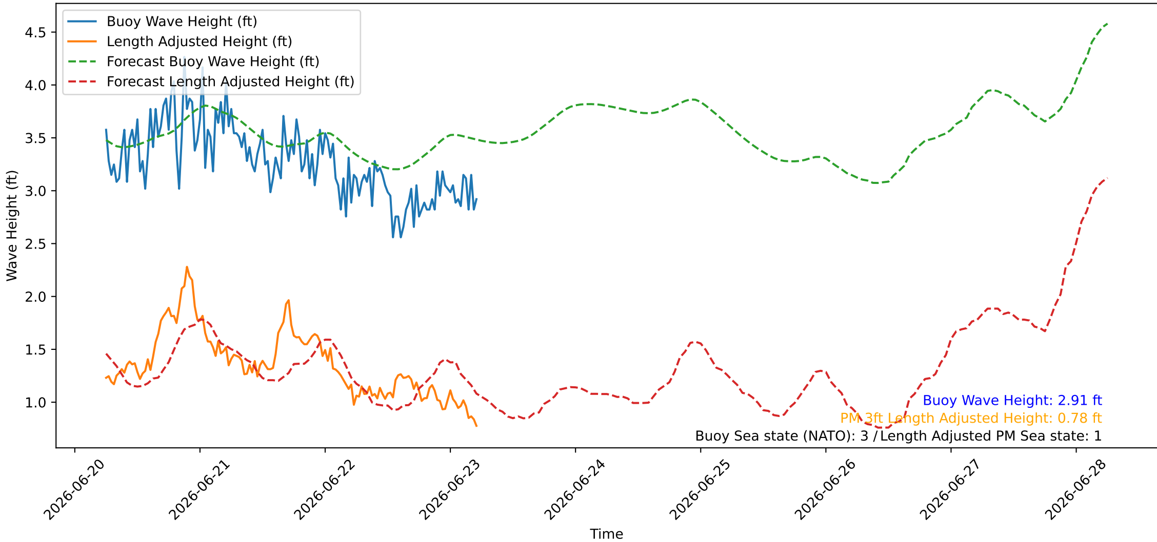
Wave Heights over Time for Oceanside Harbor at 2026-06-23 06:00:26
