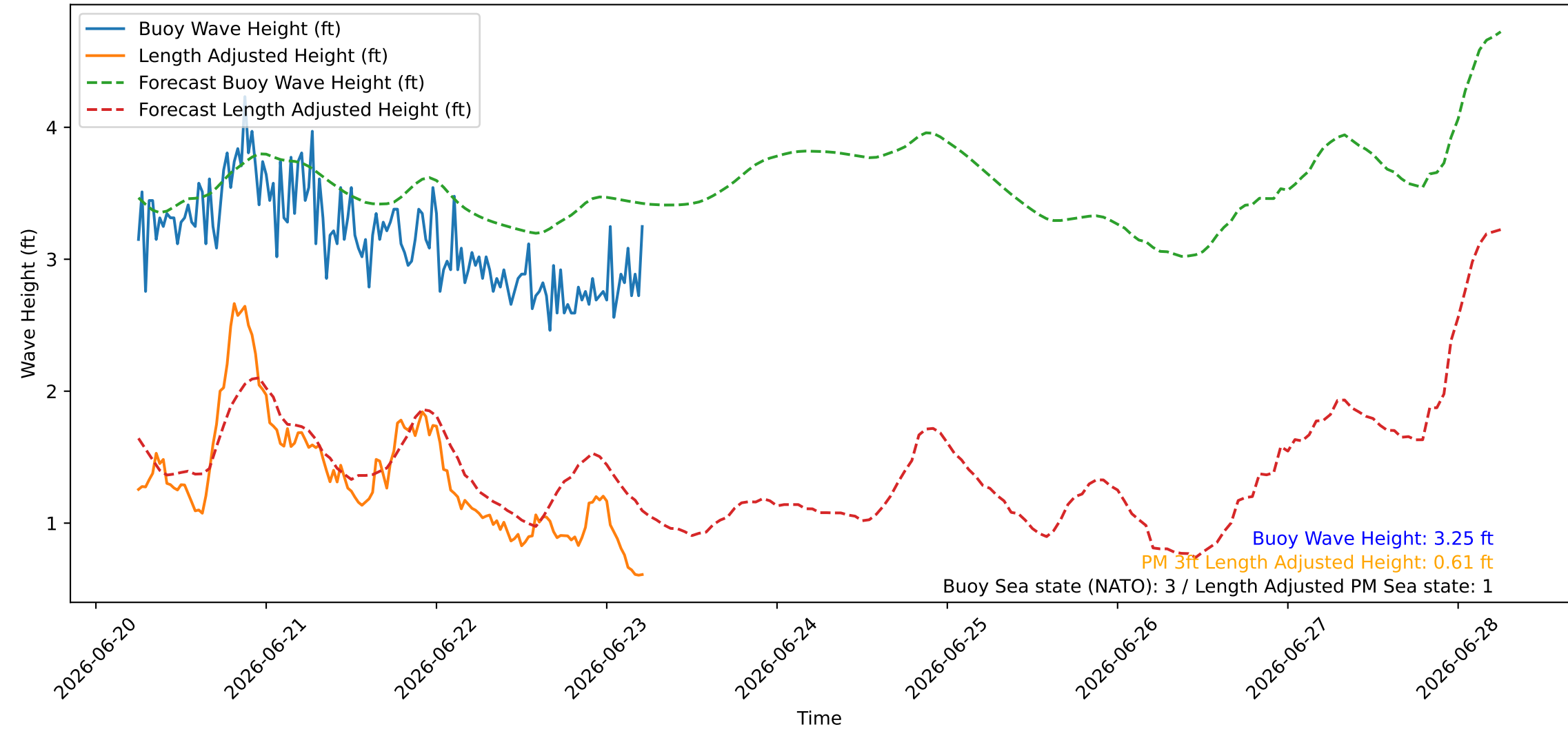
Wave Heights over Time for Green Beach at 2026-06-23 06:01:08
