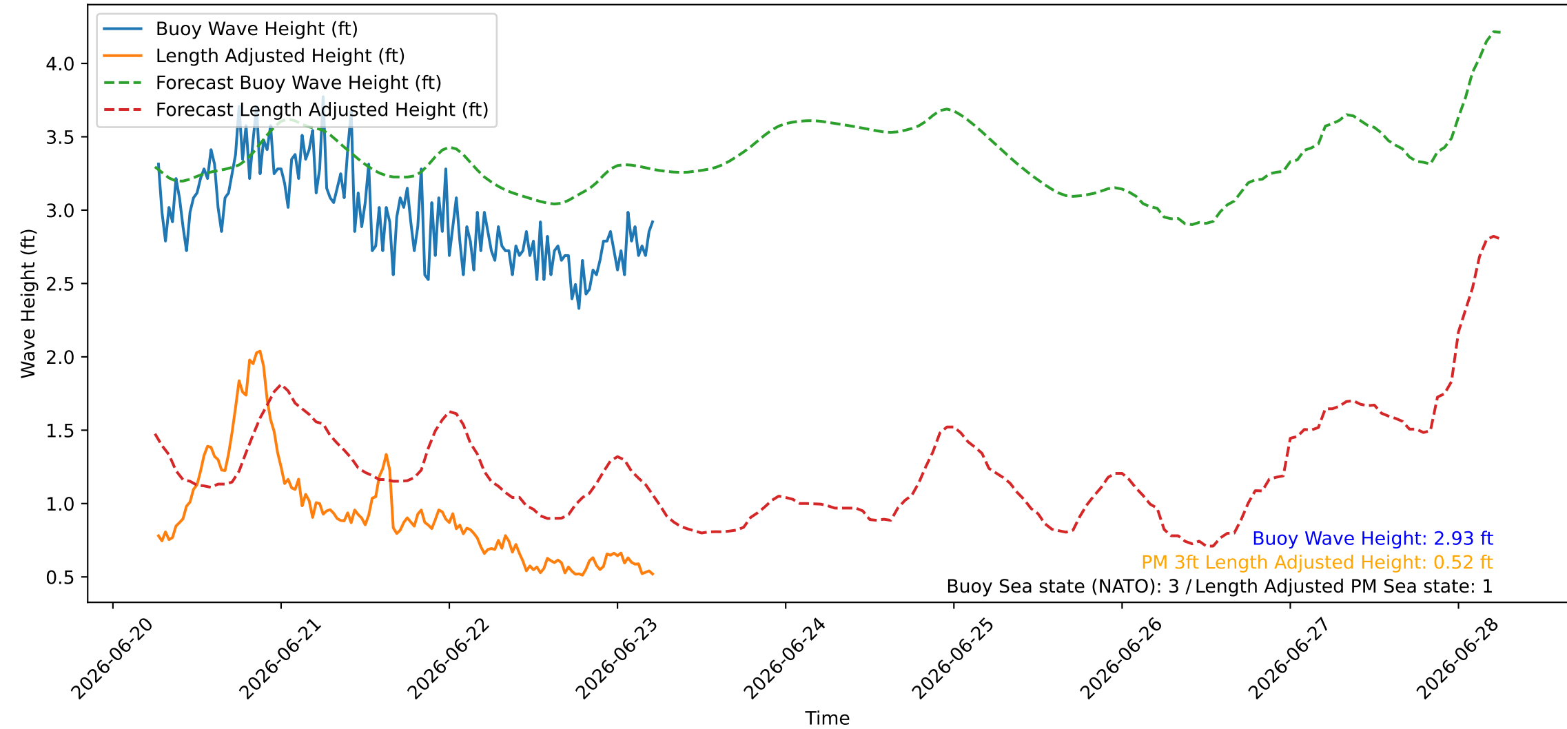
Wave Heights over Time for Red Beach at 2026-06-23 06:00:45
