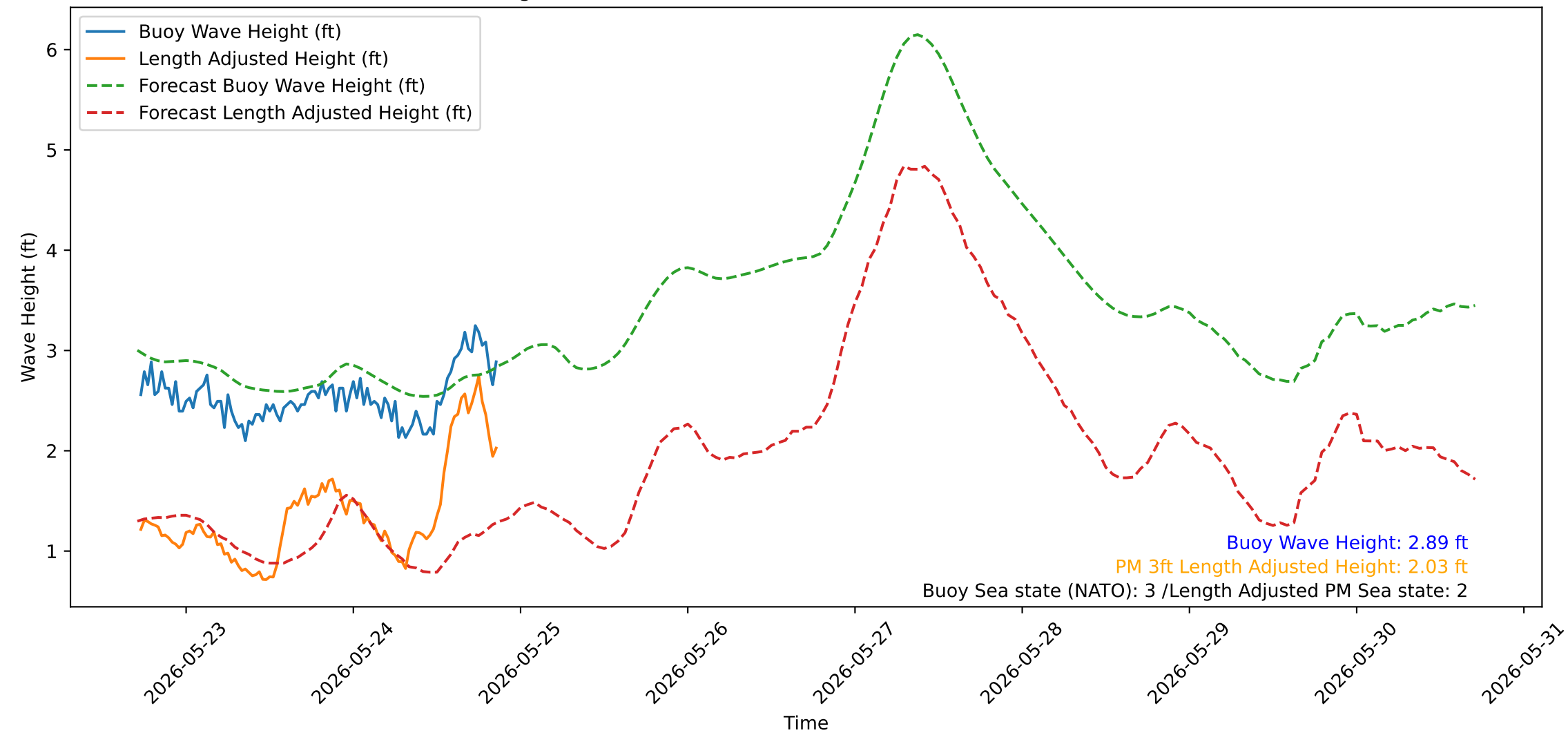
Wave Heights over Time for Oceanside Harbor at 2026-05-25 17:20:30
