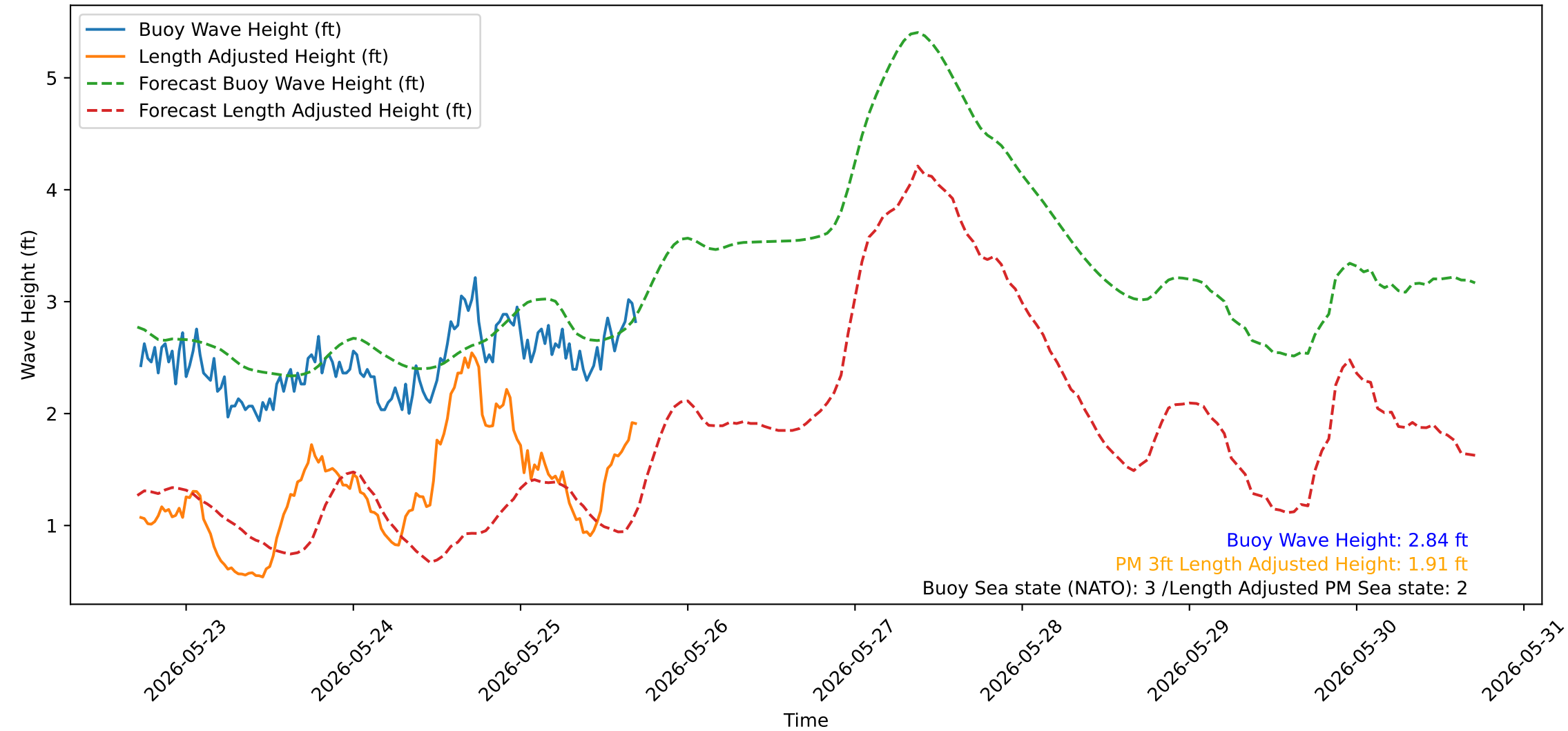
Wave Heights over Time for Red Beach at 2026-05-25 17:20:51
